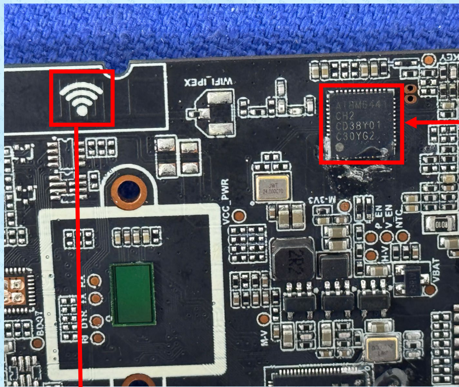
PCB Antenna
