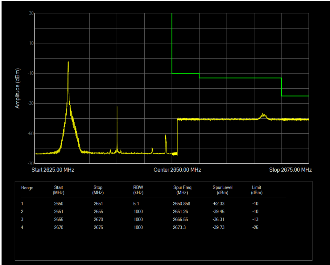
Band41 QAM16 BW=20MHz Channel=41090 RB Size=1 Position=#Max
