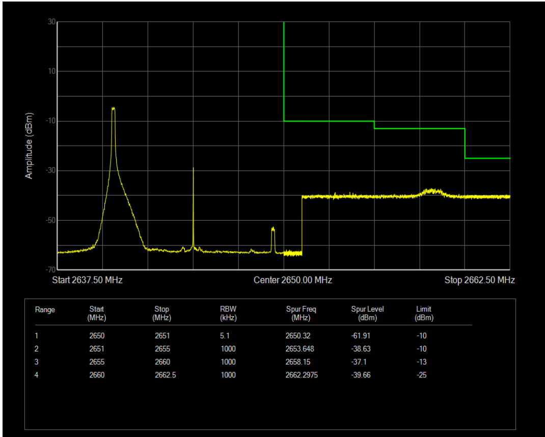
Band41 QAM16 BW=10MHz Channel=41140 RB Size=1 Position=#Max
