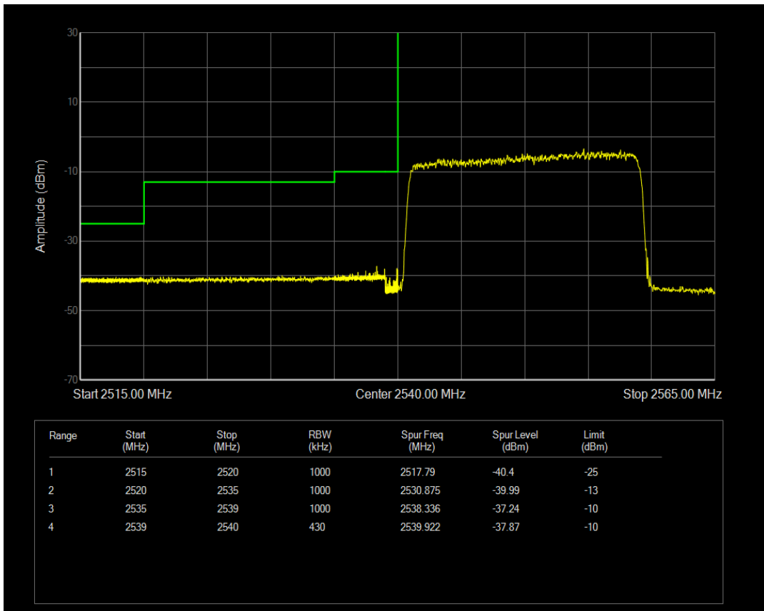
Band41 QAM16 BW=20MHz Channel=40190 RB Size=1 Position=#Max
