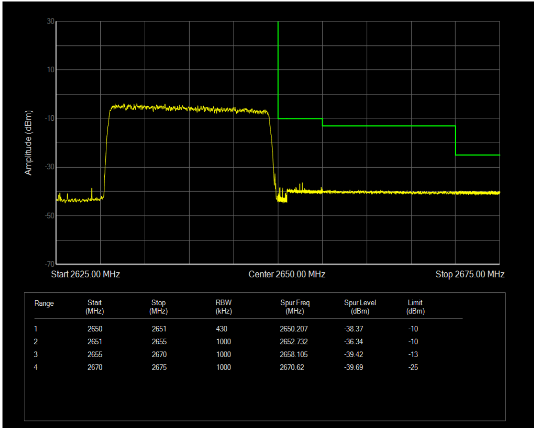
Band41 QPSK BW=20MHz Channel=41090 RB Size=1 Position=#Max
