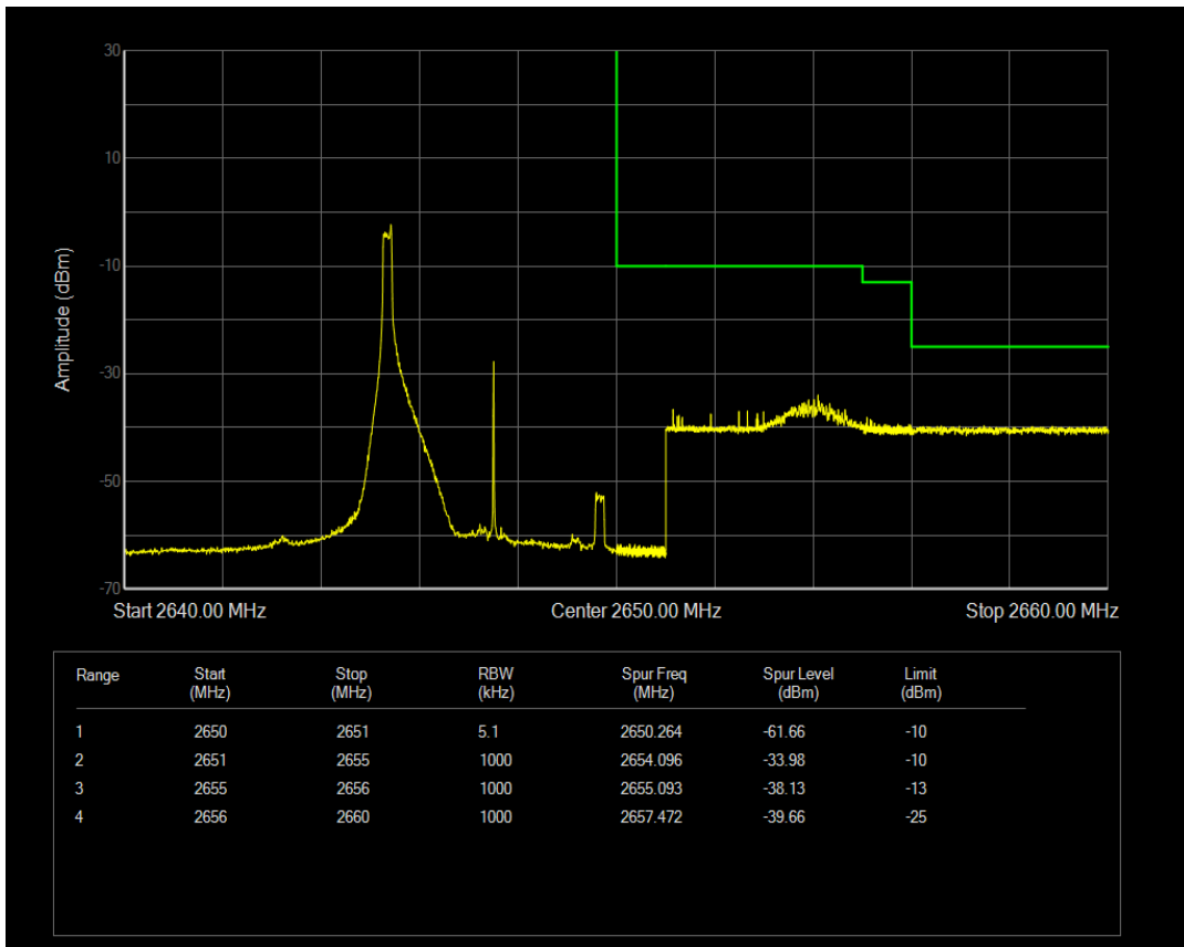
Band41 QPSK BW=5MHz Channel=41165 RB Size=1 Position=#Max
