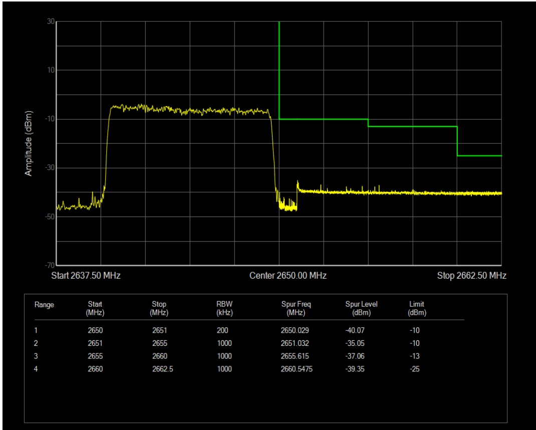
Band41 QPSK BW=10MHz Channel=41140 RB Size=1 Position=#Max
