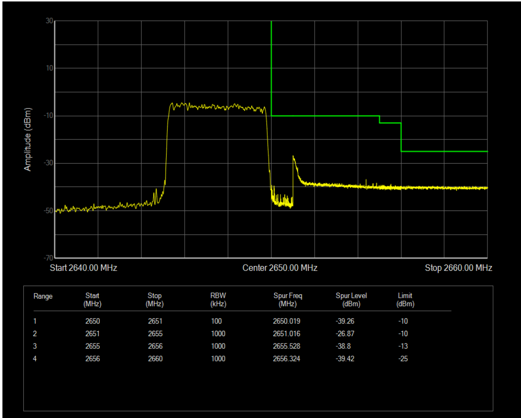
Band41 QAM16 BW=5MHz Channel=41165 RB Size=1 Position=#Max
