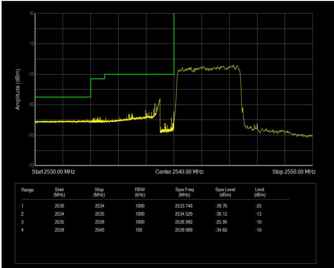
Band41 QAM16 BW=5MHz Channel=40115 RB Size=1 Position=#Max
