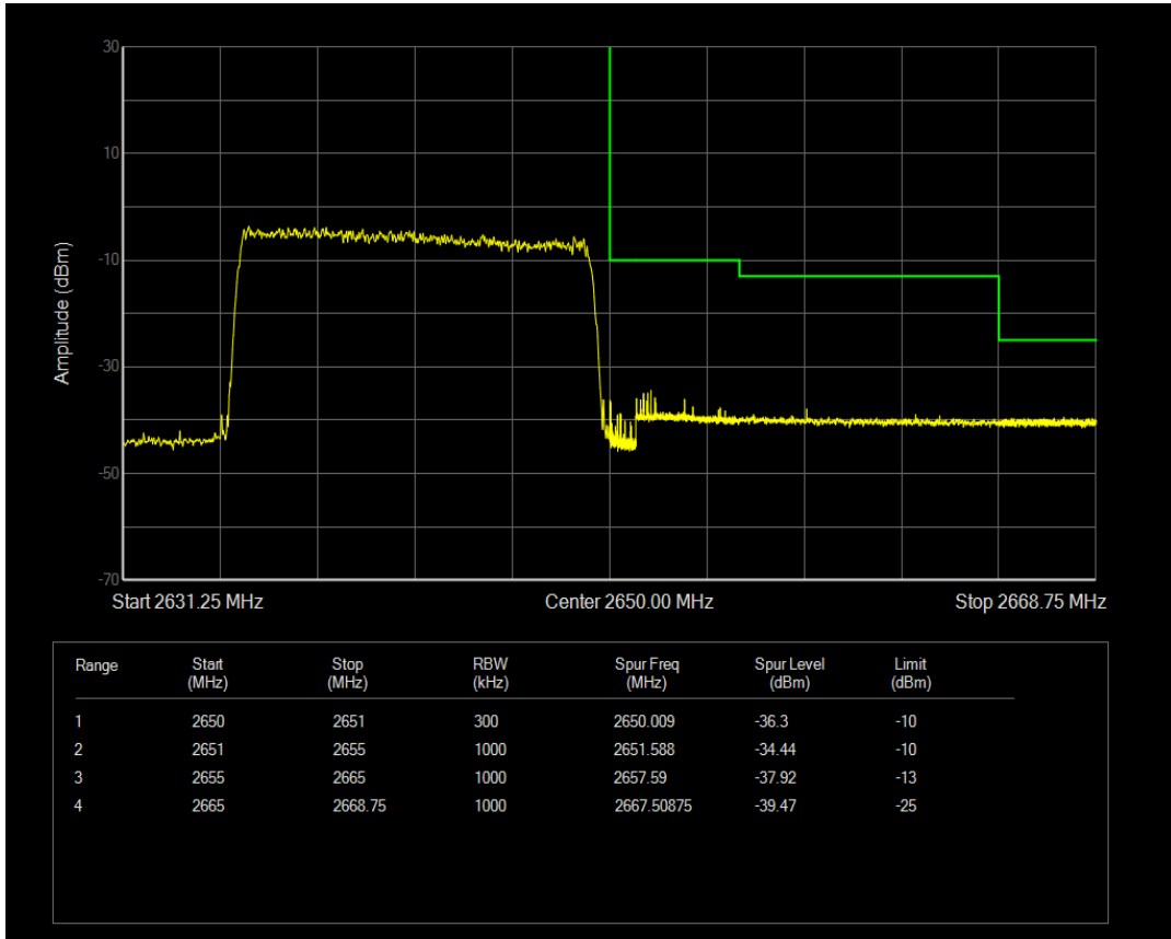
Band41 QAM16 BW=15MHz Channel=41115 RB Size=1 Position=#Max
