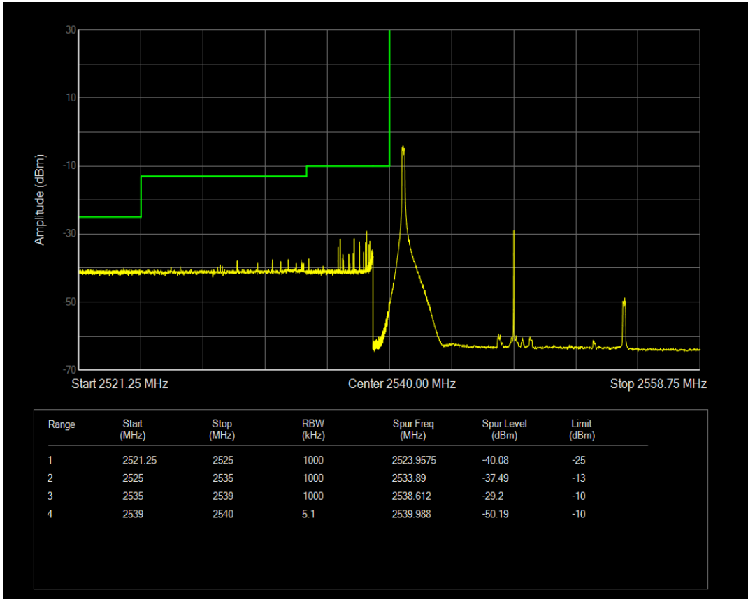
Band41 QAM16 BW=15MHz Channel=40165 RB Size=1 Position=#Max
