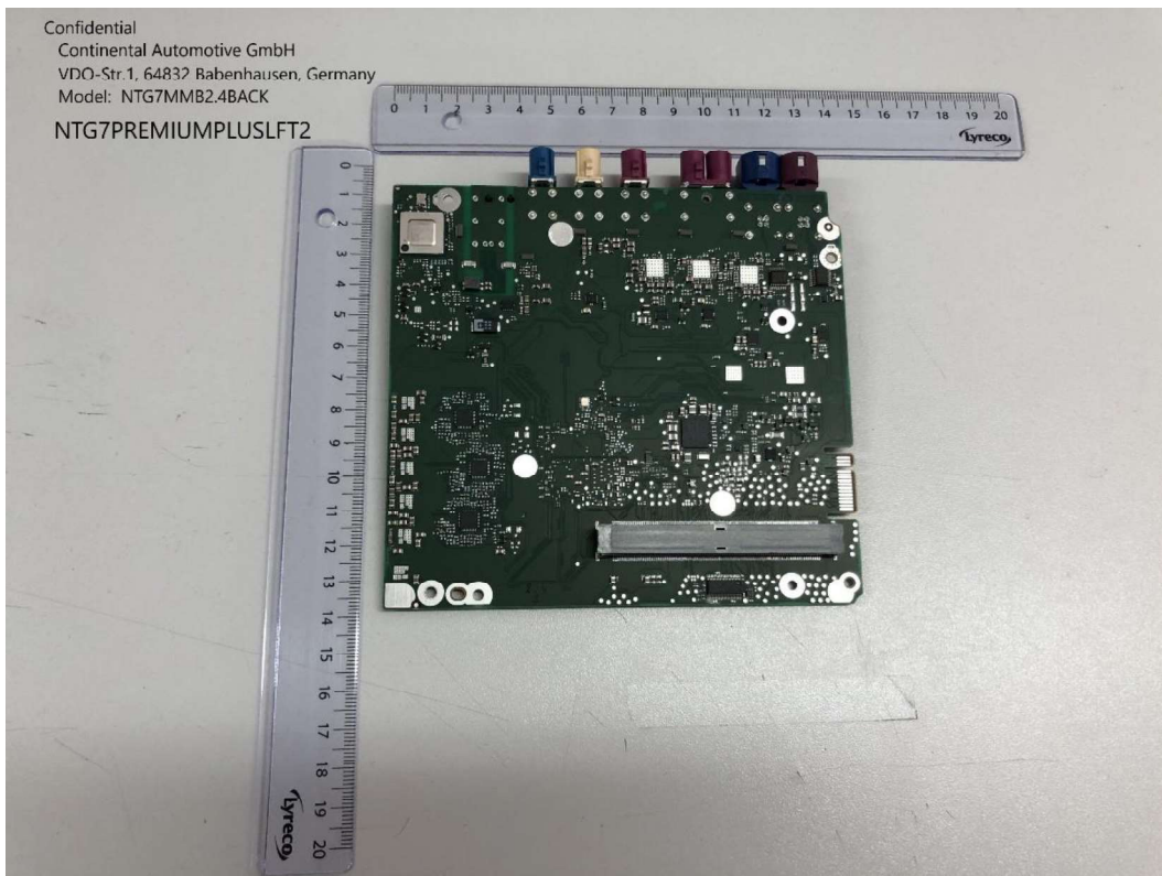
Multimedia board 2.4 bottom view
