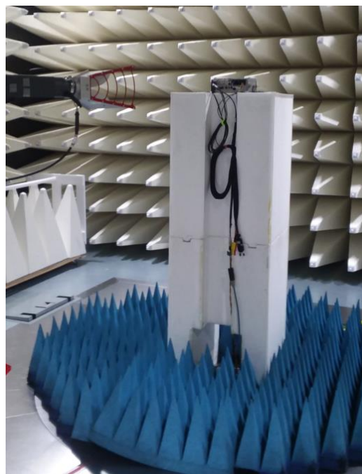
Figure C4: Radiated Emission Setup 2
