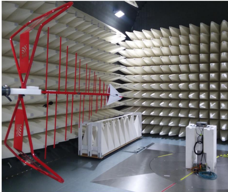
Figure C3: Radiated Emission Setup 1
