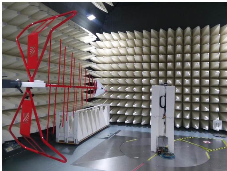
Figure B4: Radiated Emission Setup 1
