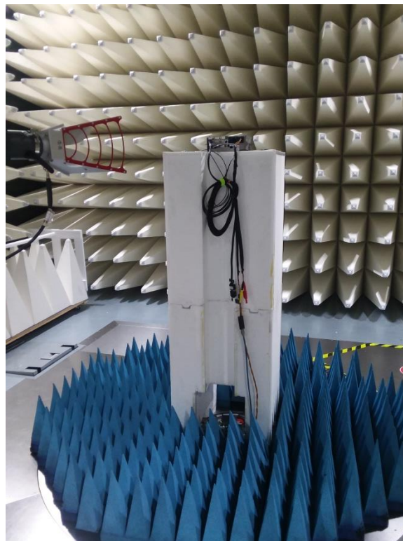
Figure 4. Radiated Setup – High Range1
