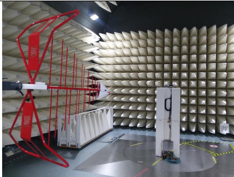
Figure3. Radiated Setup – Low Range
