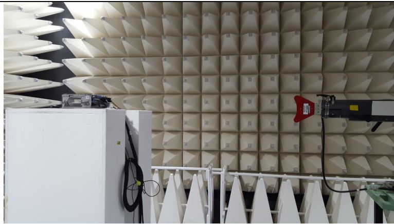
Figure 5. Radiated Setup – High Range2
