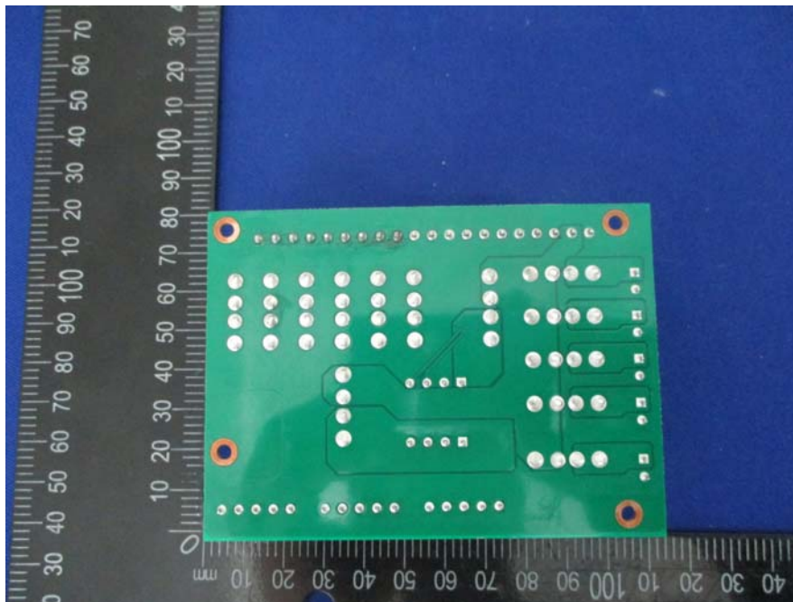
EUT – Interface Circuit Board Bottom View
