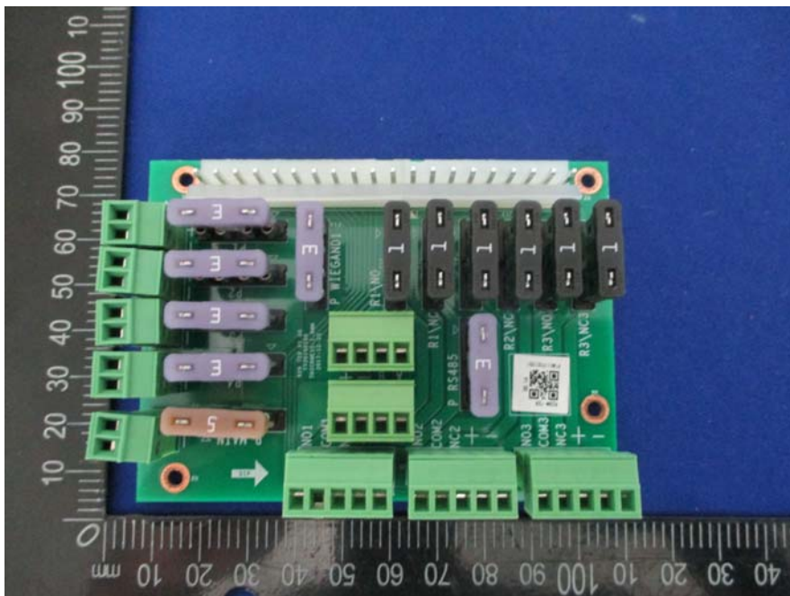
EUT – Interface Circuit Board Top View
