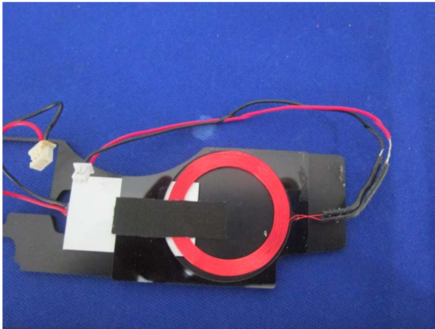
EUT –125KHz Antenna View
