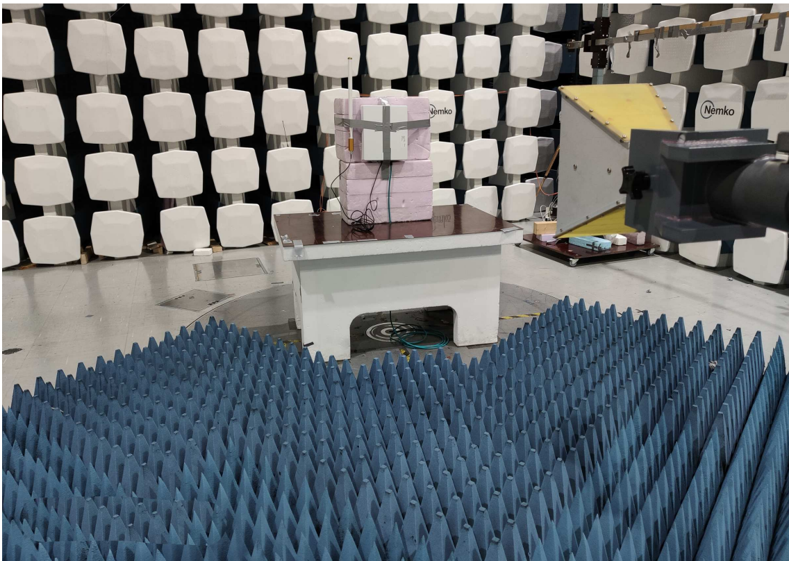
Radiated Emissions, 1-10 GHz
