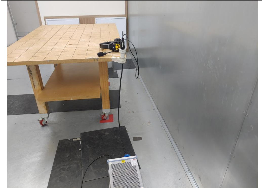
Conducted Emission_REAR
