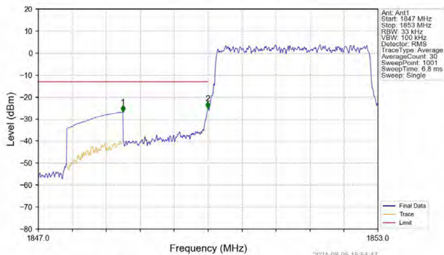
Band25_3MHz_QPSK_LCH_1851.5MHz_RB_15_0_NTNV
