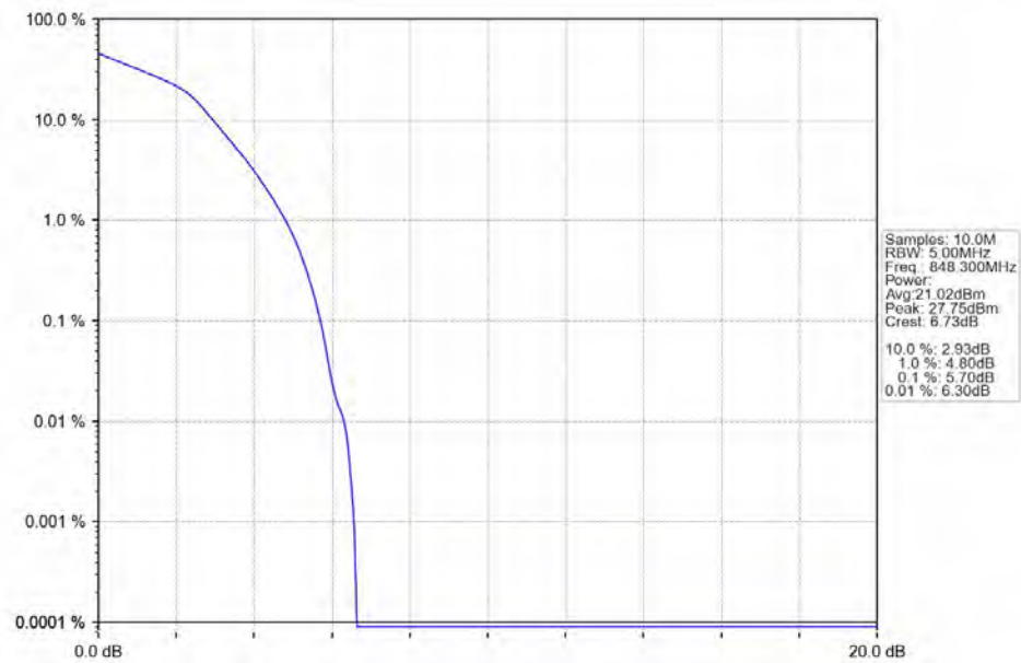
Band5_1.4MHz_16QAM_HCH_848.3MHz_RB_6_0_NTNV
