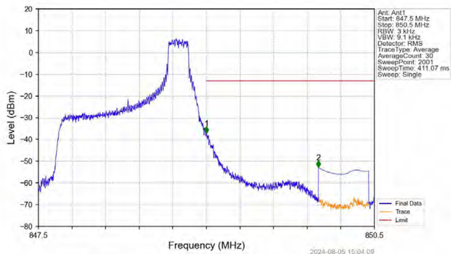
Band5_1.4MHz_QPSK_HCH_848.3MHz_RB_1_5_NTNV
