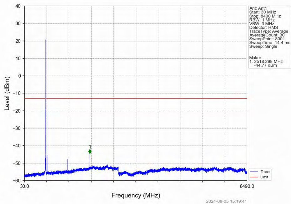
Band5_10MHz_16QAM_HCH_844MHz_RB_1_0_NTNV
