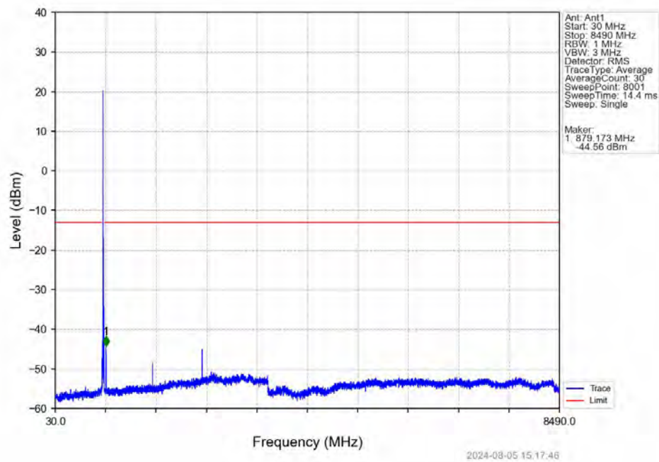
Band5_10MHz_16QAM_HCH_844MHz_RB_1_0_NTNV
