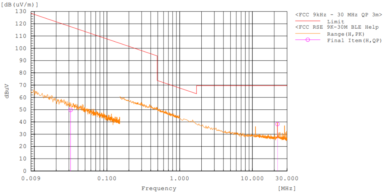
Radiated Spurious Emission 9 kHz – 30 MHz (Antenna Position 180°) : BLE MESH
