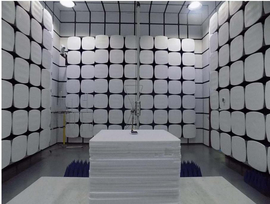
Photographs-Radiated Emission Test Setup in Chamber
