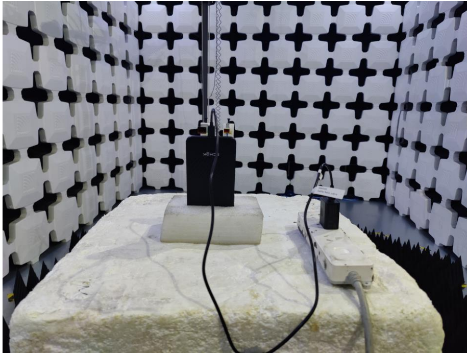
5. Radiated Emissions (Part 15C&Part 15E, 26.5GHz -40GHz)
