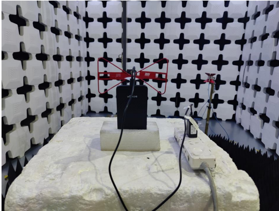
3. Radiated Emissions (Part 15C&Part 15E, 1GHz -18GHz)
