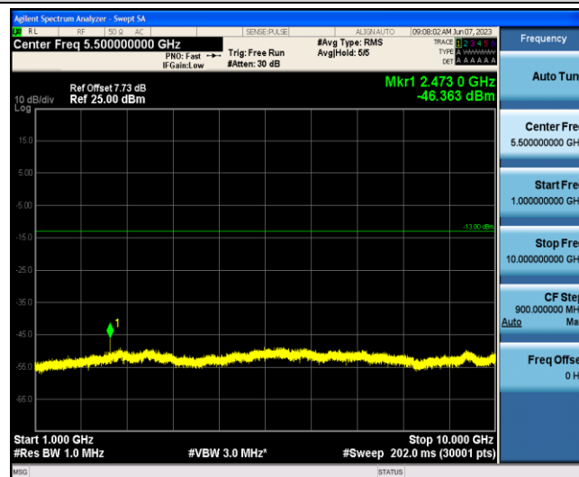
Band5-5MHz-QPSK-20425-1-0-Low-1000-10000--46.36-PASS
