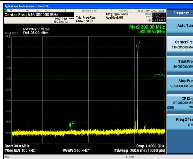
Band5-5MHz-16QAM-20425-1-0-Low-30-1000--60.4-PASS
