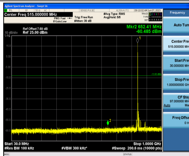
Band5-5MHz-16QAM-20625-1-0-Low-30-1000--60.49-PASS
