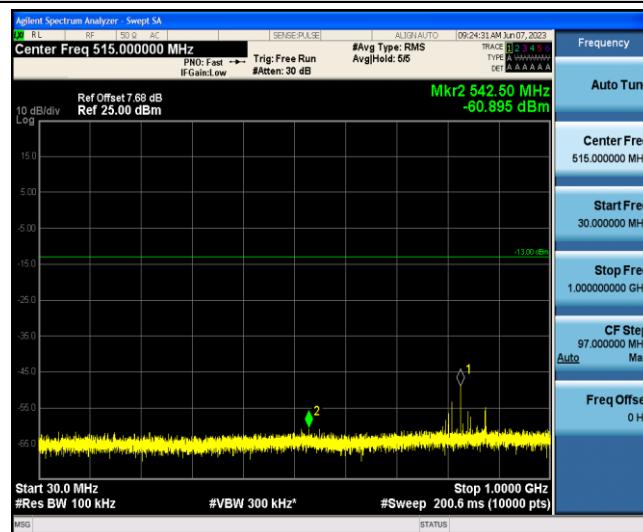
Band5-10MHz-16QAM-20450-1-0-Low-30-1000--60.9-PASS
