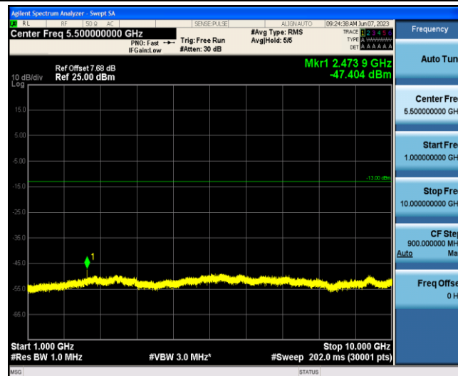
Band5-10MHz-16QAM-20450-1-0-Low-1000-10000--47.4-PASS
