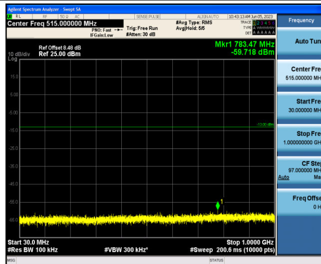
Band4-20MHz-16QAM-20175-1-0-Low-30-1000--59.72-PASS
