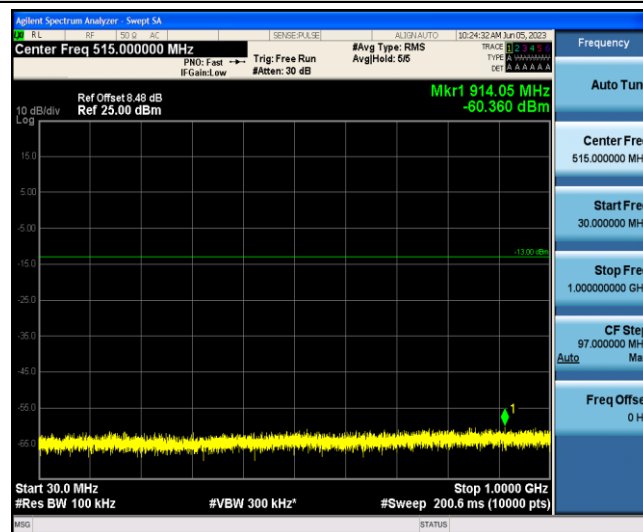
Band4-15MHz-16QAM-20325-1-0-Low-30-1000--60.36-PASS
