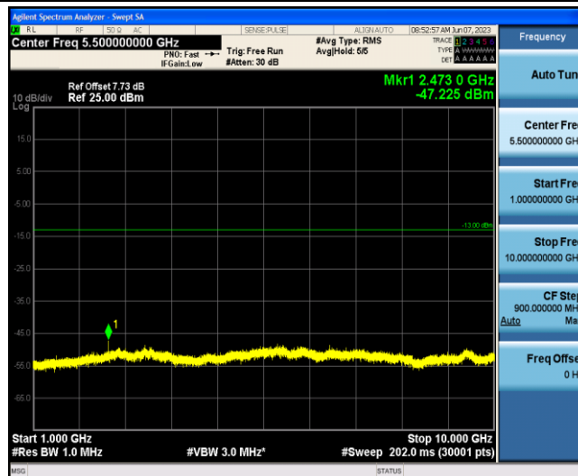
Band5-3MHz-16QAM-20415-1-0-Low-1000-10000--47.23-PASS
