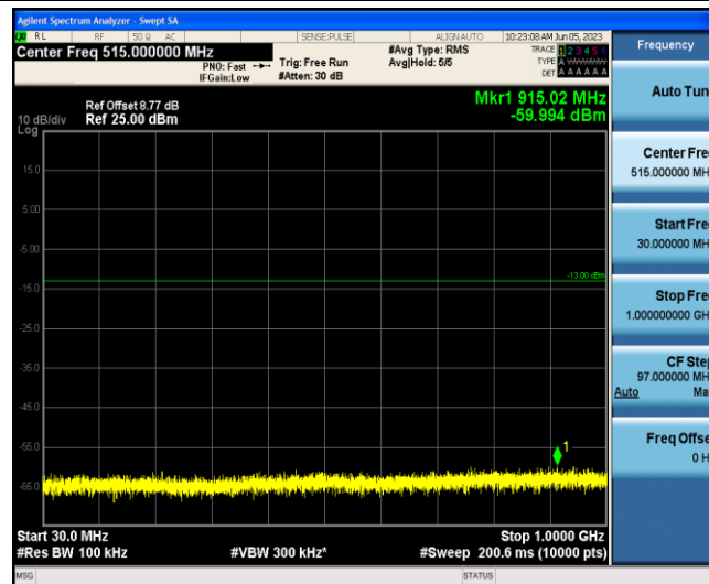
Band4-15MHz-16QAM-20025-1-0-Low-30-1000--59.99-PASS
