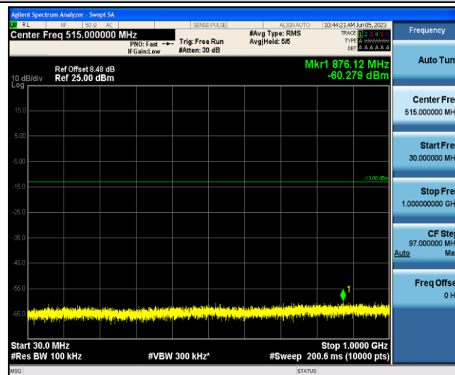
Band4-20MHz-1RB#0@Low-20300-1-0-High-30-1000--60.28-PASS
