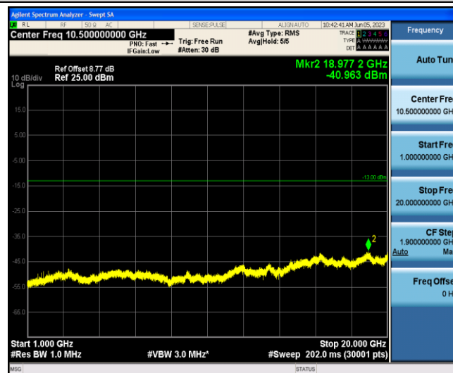
Band4-20MHz-16QAM-20050-1-0-Low-1000-20000--40.96-PASS
