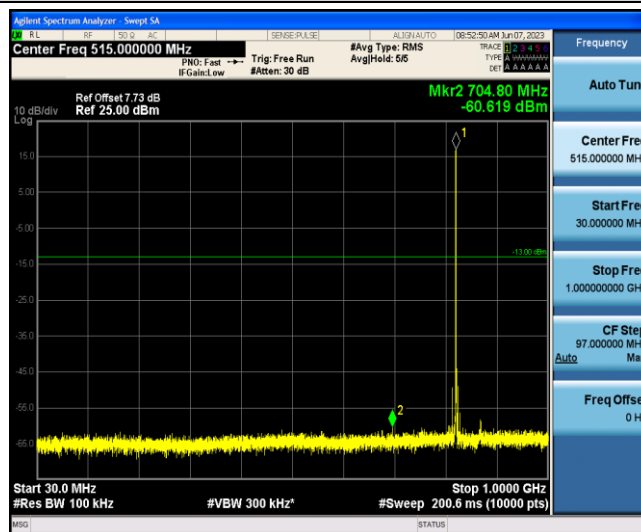
Band5-3MHz-16QAM-20415-1-0-Low-30-1000--60.62-PASS
