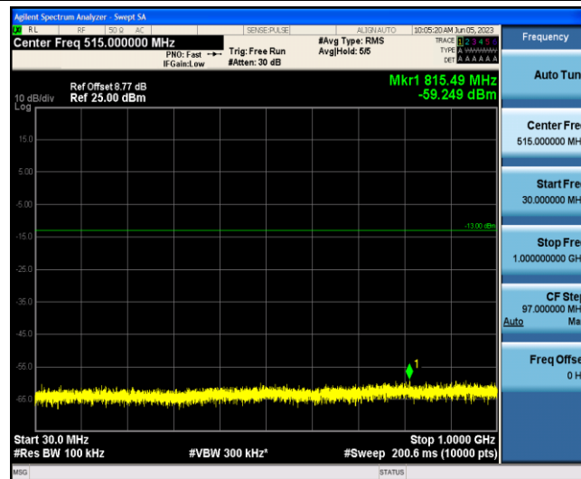
Band4-10MHz-16QAM-20000-1-0-Low-30-1000--59.25-PASS
