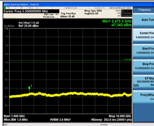
Band5-3MHz-QPSK-20415-1-0-Low-1000-10000--47.34-PASS
