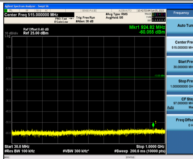
Band4-20MHz-QPSK-20175-1-0-Low-30-1000--60.06-PASS
