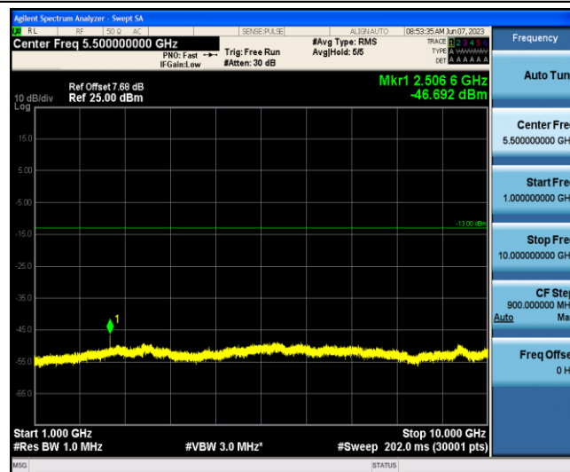
Band5-3MHz-16QAM-20525-1-0-Low-1000-10000--46.69-PASS
