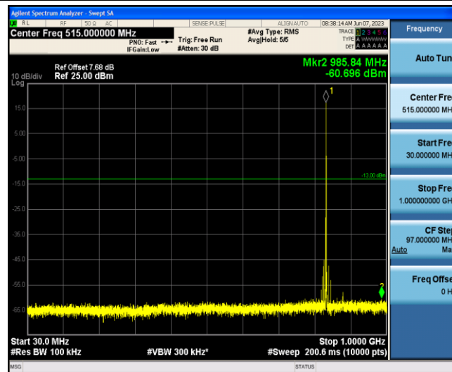
Band5-1.4MHz-16QAM-20525-1-0-Low-30-1000--60.7-PASS
