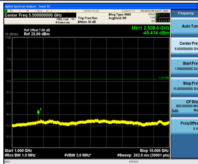
Band5-1.4MHz-QPSK-20525-1-0-Low-1000-10000--45.41-PASS
