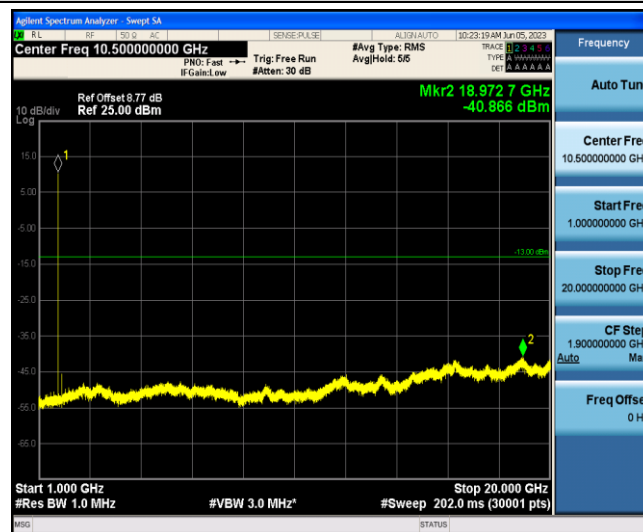
Band4-15MHz-16QAM-20025-1-0-Low-1000-20000--40.87-PASS
