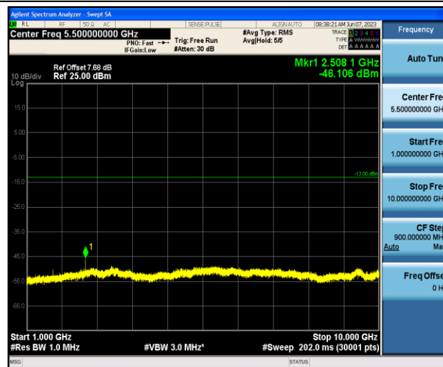
Band5-1.4MHz-16QAM-20525-1-0-Low-1000-10000--46.11-PASS
