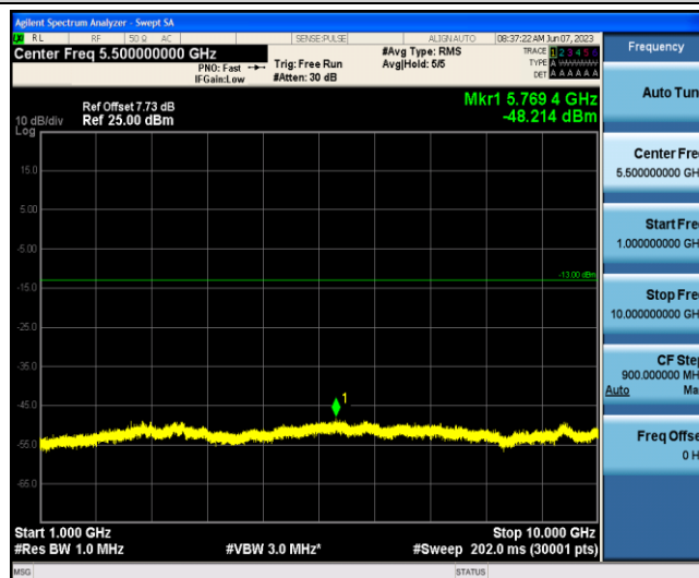
Band5-1.4MHz-QPSK-20407-1-0-Low-1000-10000--48.21-PASS
