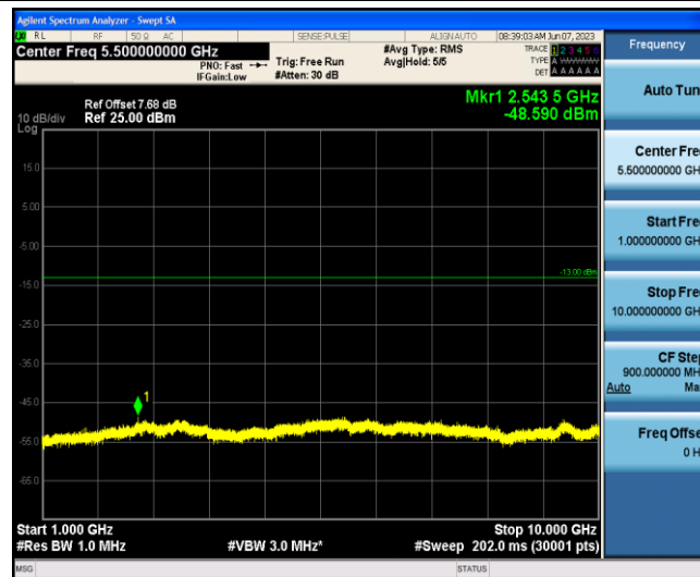
Band5-1.4MHz-16QAM-20643-1-0-Low-1000-10000--48.59-PASS
