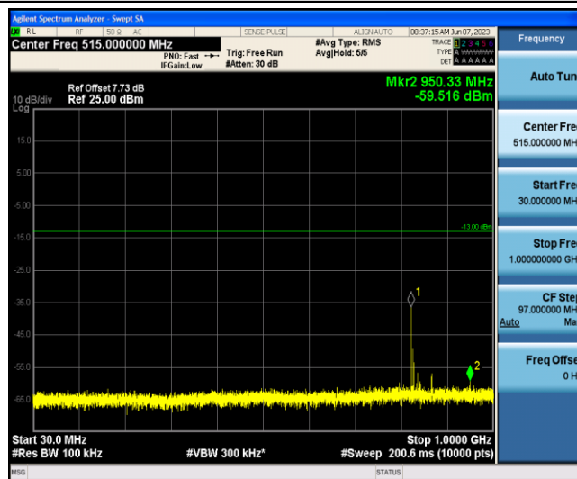
Band5-1.4MHz-QPSK-20407-1-0-Low-30-1000--59.52-PASS
