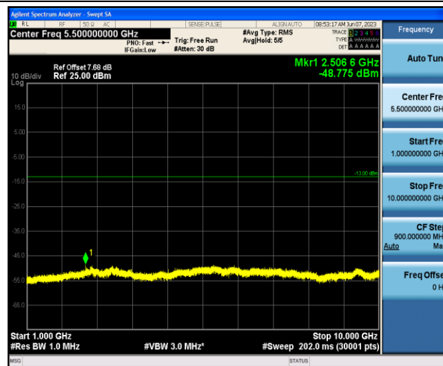
Band5-3MHz-QPSK-20525-1-0-Low-1000-10000--48.78-PASS
