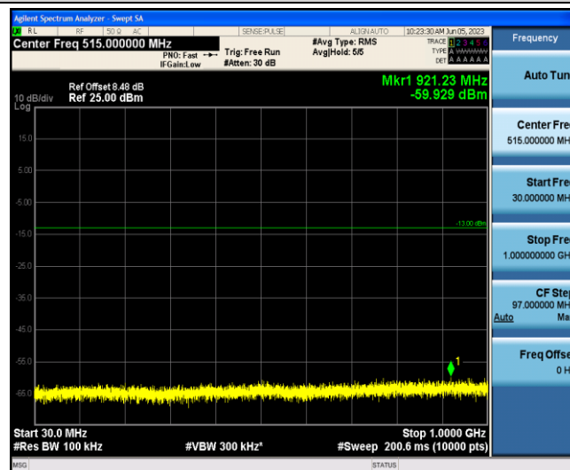
Band4-15MHz-QPSK-20175-1-0-Low-30-1000--59.93-PASS
