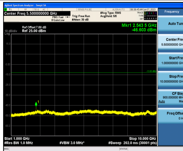
Band5-1.4MHz-QPSK-20643-1-0-Low-1000-10000--46.6-PASS
