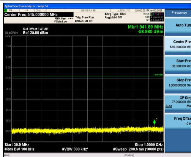
Band4-10MHz-16QAM-20175-1-0-Low-30-1000--58.98-PASS
