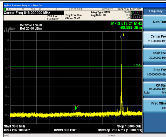
Band5-1.4MHz-QPSK-20643-1-0-Low-30-1000--60.59-PASS
