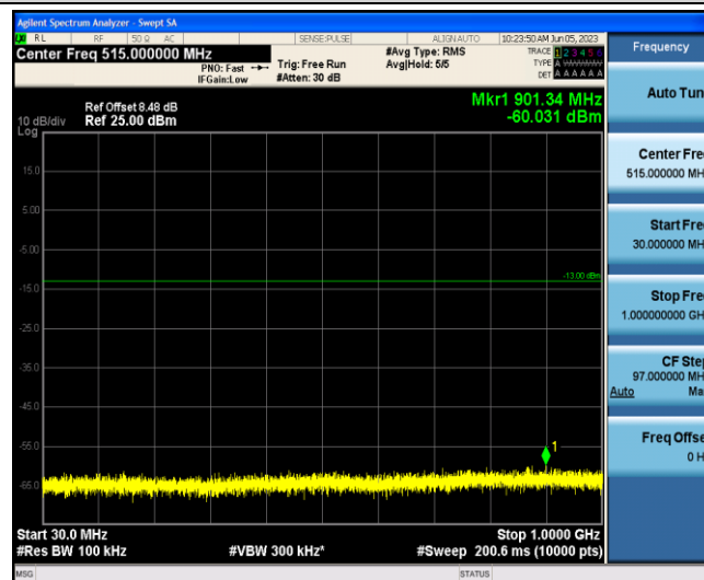
Band4-15MHz-16QAM-20175-1-0-Low-30-1000--60.03-PASS
