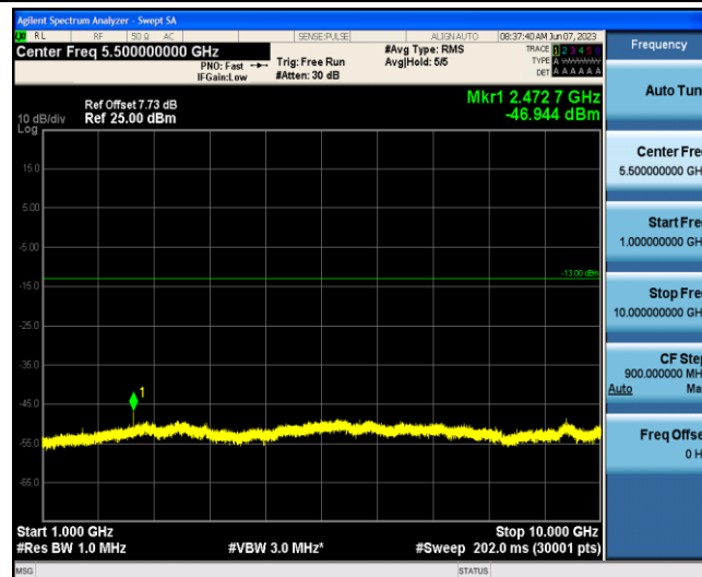
Band5-1.4MHz-16QAM-20407-1-0-Low-1000-10000--46.94-PASS
