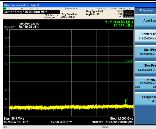
Band4-15MHz-QPSK-20325-1-0-Low-30-1000--60.09-PASS
