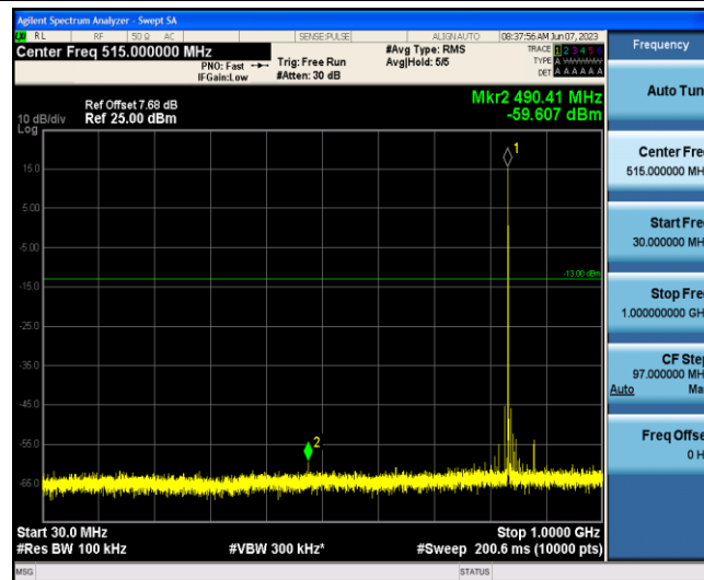
Band5-1.4MHz-QPSK-20525-1-0-Low-30-1000--59.61-PASS
