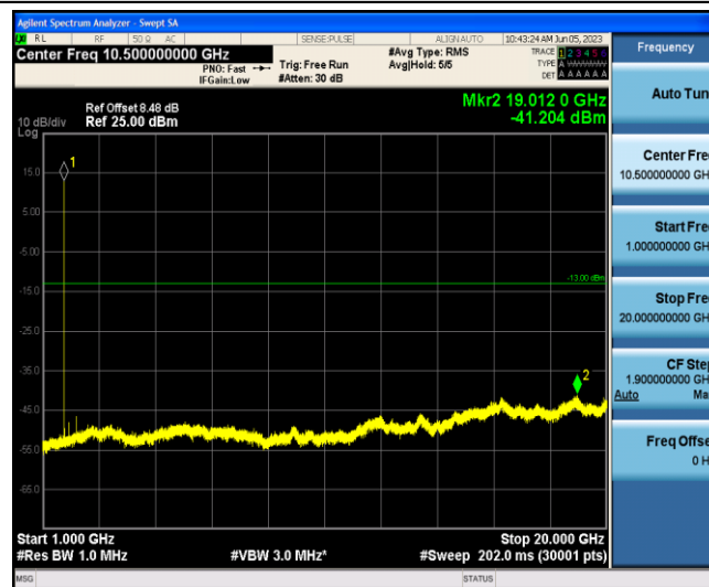
Band4-20MHz-16QAM-20175-1-0-Low-1000-20000--41.2-PASS
