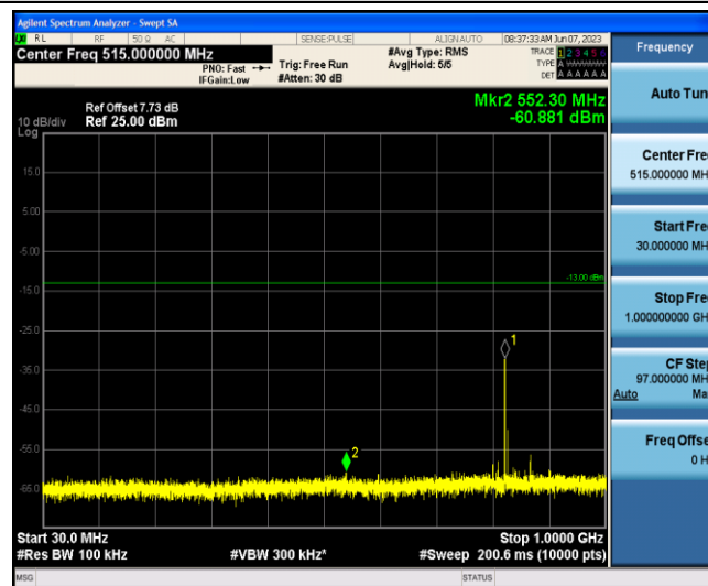
Band5-1.4MHz-16QAM-20407-1-0-Low-30-1000--60.88-PASS
