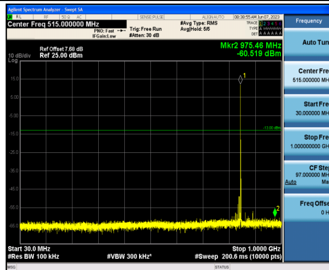
Band5-1.4MHz-16QAM-20643-1-0-Low-30-1000--60.52-PASS
