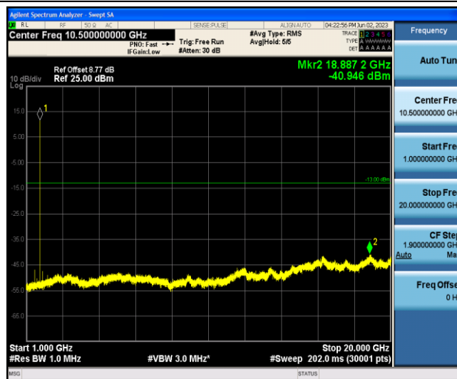
Band4-1.4MHz-16QAM-19957-1-0-Low-1000-20000--40.95-PASS
