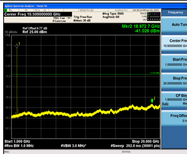
Band4-3MHz-16QAM-19965-1-0-Low-1000-20000--41.03-PASS
