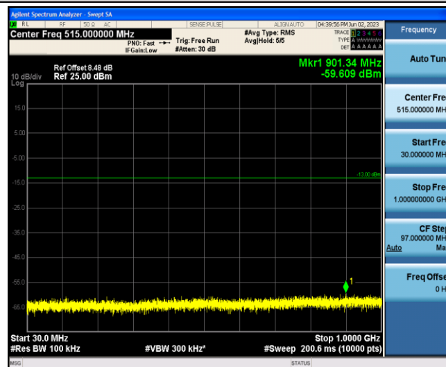
Band4-3MHz-16QAM-20175-1-0-Low-30-1000--59.61-PASS
