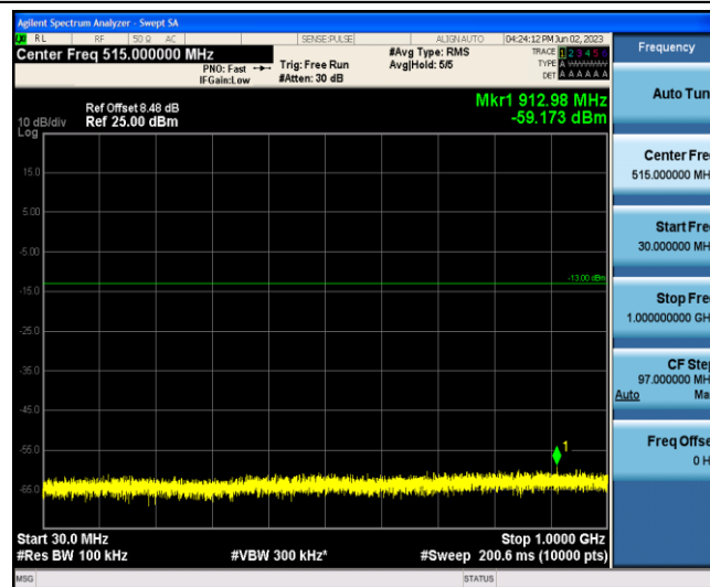
Band4-1.4MHz-16QAM-20393-1-0-Low-30-1000--59.17-PASS
