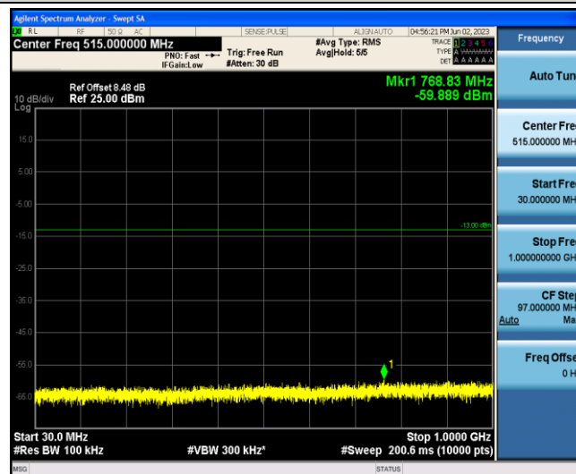
Band4-5MHz-16QAM-20175-1-0-Low-30-1000--59.89-PASS
