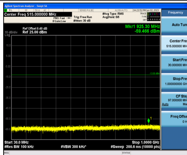
Band4-1.4MHz-QPSK-20393-1-0-Low-30-1000--59.47-PASS
