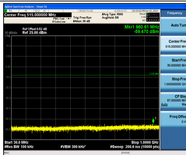
Band2-15MHz-16QAM-19125-1-0-Low-30-1000--59.47-PASS
