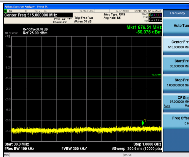
Band4-3MHz-QPSK-20385-1-0-Low-30-1000--60.08-PASS
