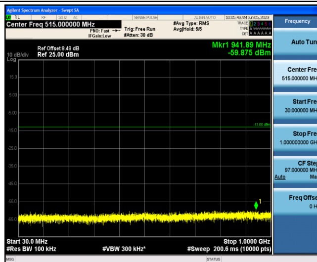
Band4-10MHz-QPSK-20175-1-0-Low-30-1000--59.88-PASS
