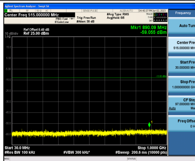
Band4-3MHz-16QAM-20385-1-0-Low-30-1000--59.06-PASS
