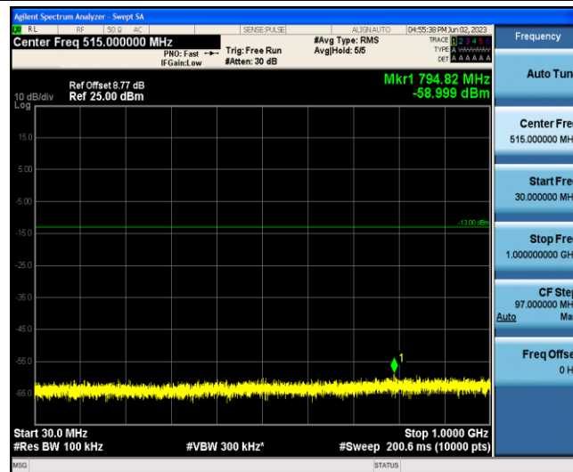
Band4-5MHz-16QAM-19975-1-0-Low-30-1000--59-PASS
