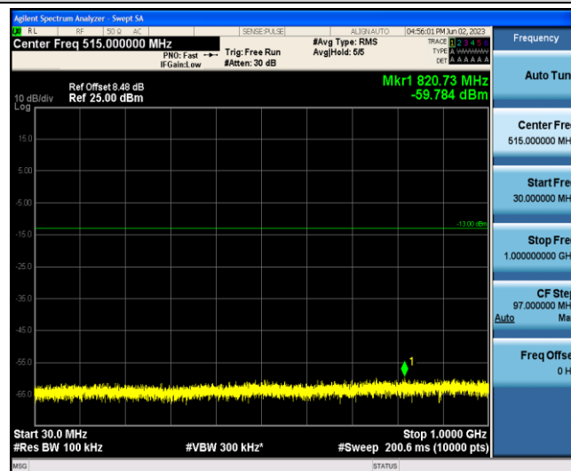
Band4-5MHz-QPSK-20175-1-0-Low-30-1000--59.78-PASS
