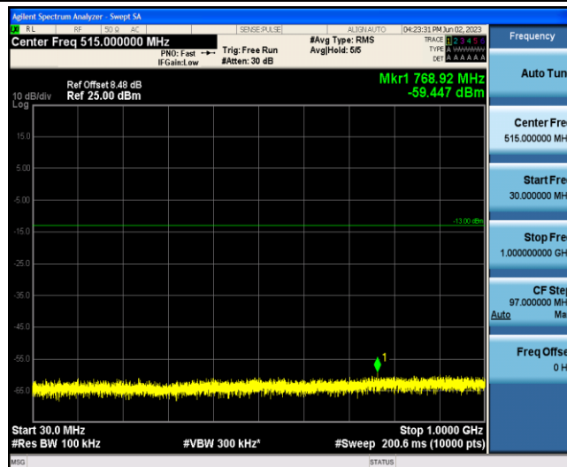
Band4-1.4MHz-16QAM-20175-1-0-Low-30-1000--59.45-PASS
