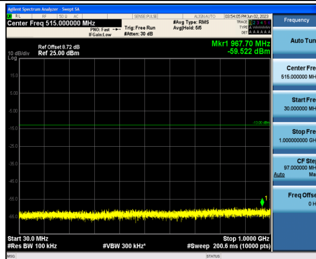
Band2-20MHz-16QAM-18900-1-0-Low-30-1000--59.52-PASS
