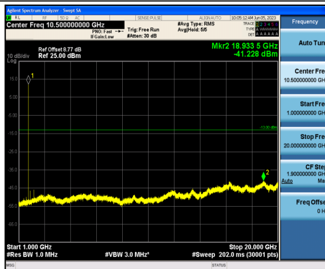
Band4-10MHz-QPSK-20000-1-0-Low-1000-20000--41.23-PASS
