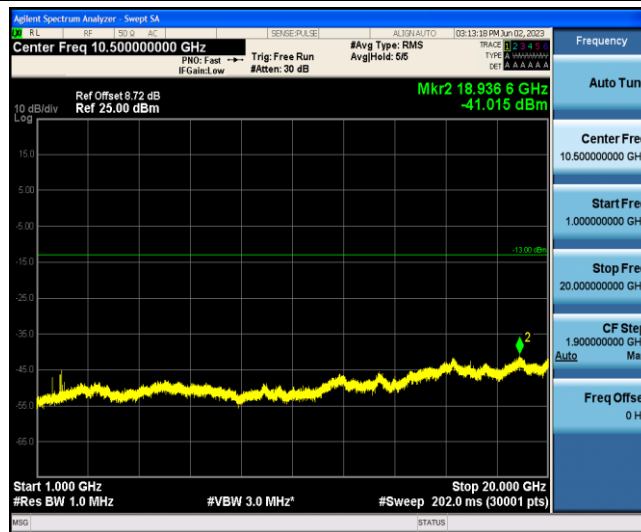
Band2-10MHz-QPSK-18650-1-0-Low-1000-20000--41.02-PASS
