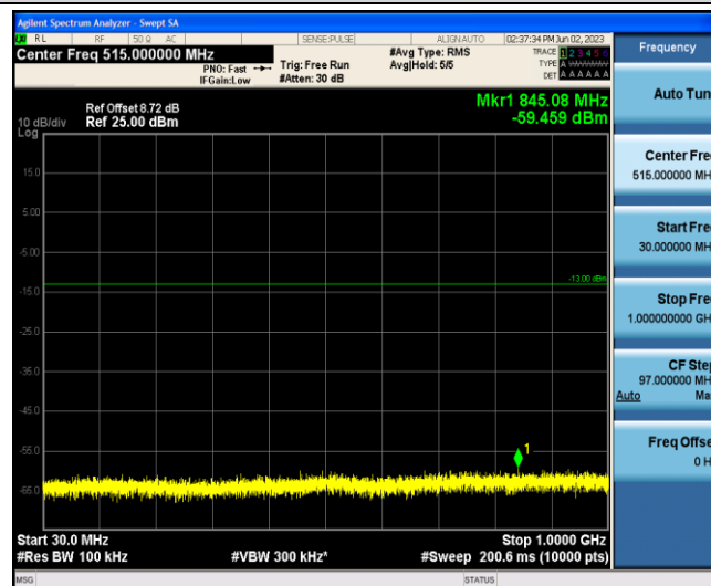
Band2-3MHz-16QAM-18900-1-0-Low-30-1000--59.46-PASS
