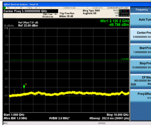
Band12-10MHz-16QAM-23130-1-0-Low-1000-10000--46.79-PASS
