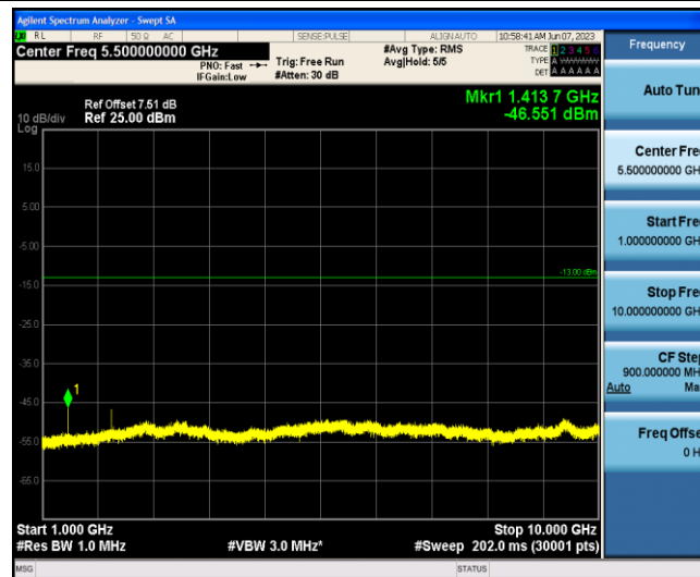
Band12-10MHz-QPSK-23130-1-0-Low-1000-10000--46.55-PASS
