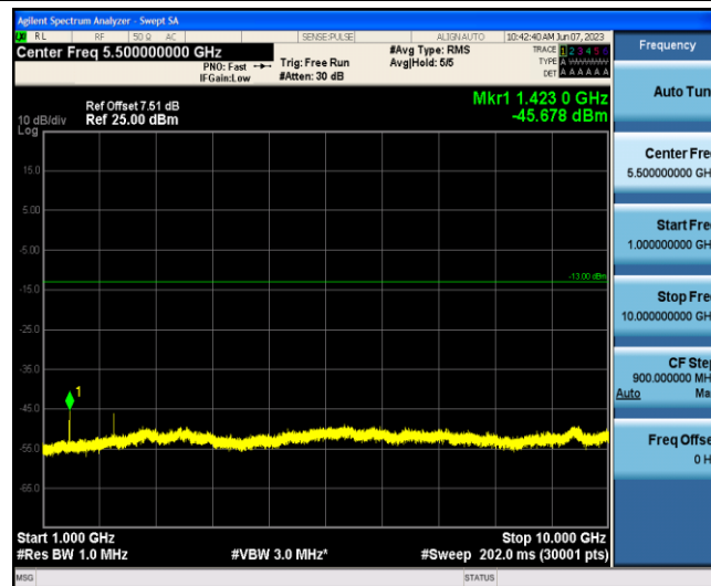
Band12-5MHz-QPSK-23155-1-0-Low-1000-10000--45.68-PASS
