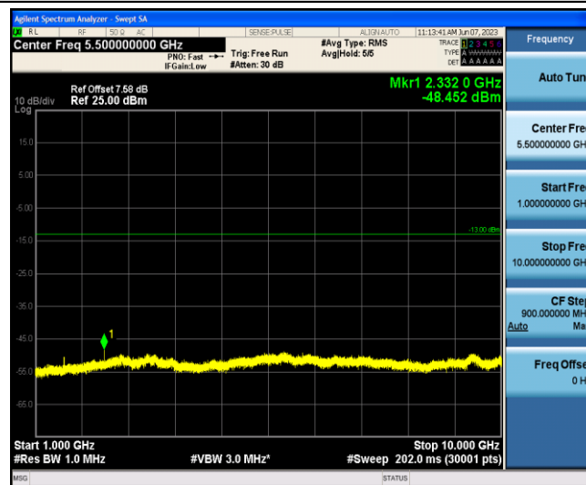
Band13-5MHz-QPSK-23205-1-0-Low-1000-10000--48.45-PASS
