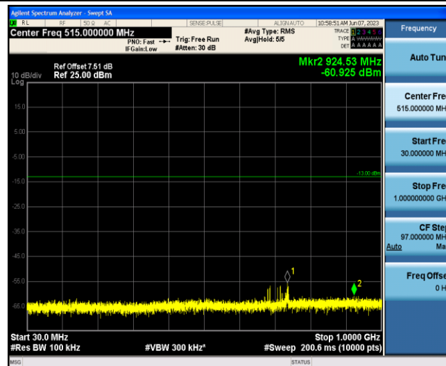
Band12-10MHz-16QAM-23130-1-0-Low-30-1000--60.93-PASS
