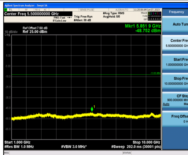
Band13-5MHz-16QAM-23255-1-0-Low-1000-10000--48.75-PASS
