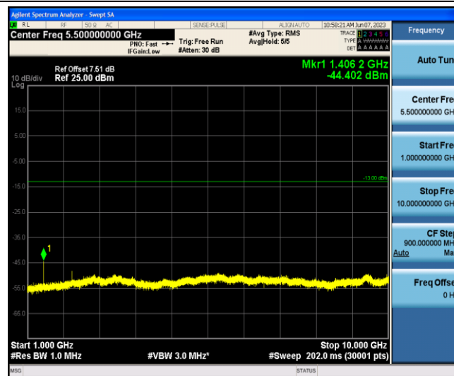
Band12-10MHz-16QAM-23095-1-0-Low-1000-10000--44.4-PASS
