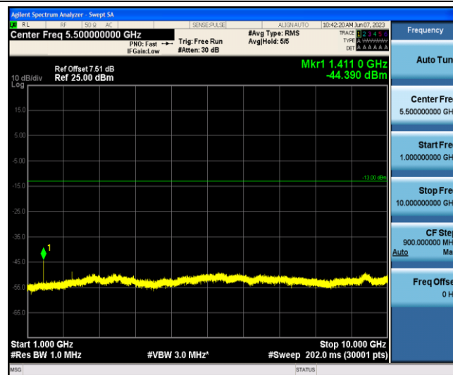
Band12-5MHz-16QAM-23095-1-0-Low-1000-10000--44.39-PASS
