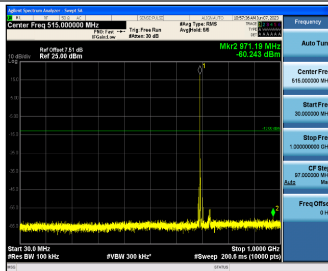
Band12-10MHz-16QAM-23060-1-0-Low-30-1000--60.24-PASS
