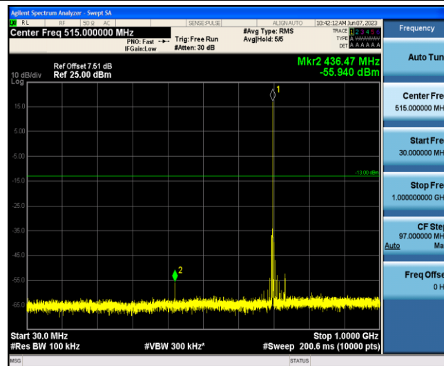
Band12-5MHz-16QAM-23095-1-0-Low-30-1000--55.94-PASS
