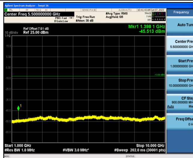
Band12-5MHz-16QAM-23035-1-0-Low-1000-10000--45.51-PASS
