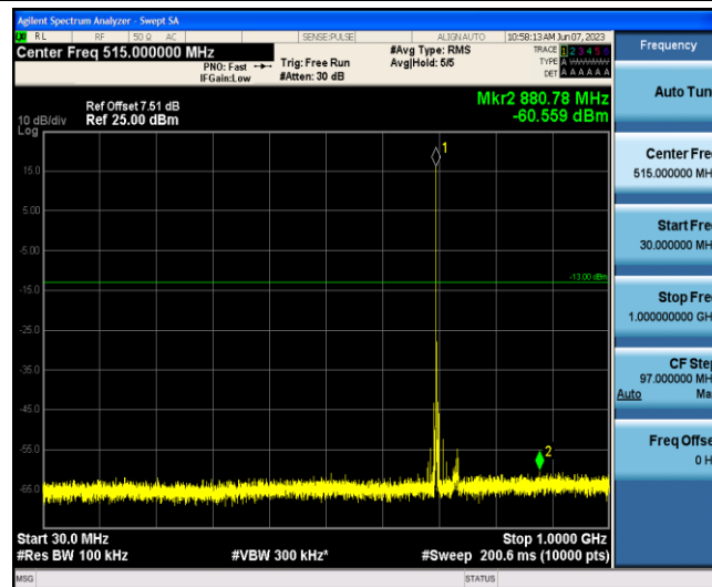
Band12-10MHz-16QAM-23095-1-0-Low-30-1000--60.56-PASS
