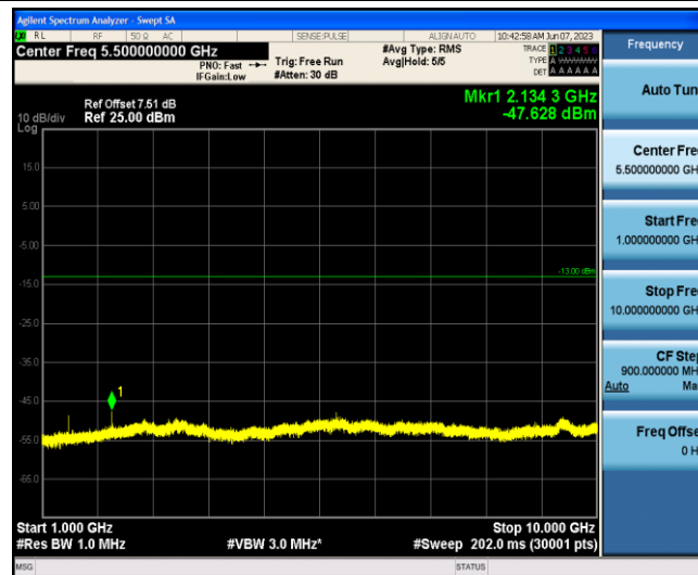
Band12-5MHz-16QAM-23155-1-0-Low-1000-10000--47.63-PASS
