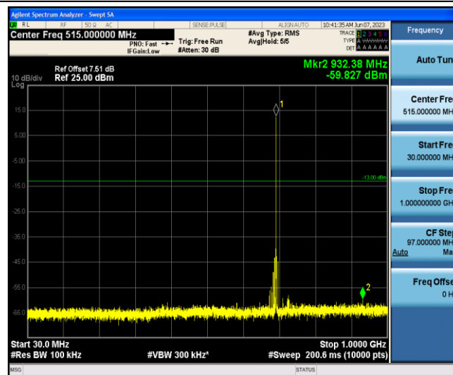
Band12-5MHz-16QAM-23035-1-0-Low-30-1000--59.83-PASS
