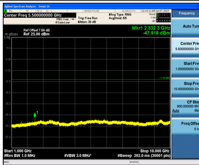
Band13-5MHz-16QAM-23205-1-0-Low-1000-10000--47.92-PASS
