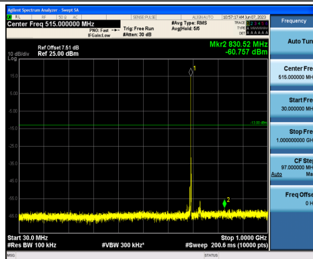
Band12-10MHz-QPSK-23060-1-0-Low-30-1000--60.76-PASS
