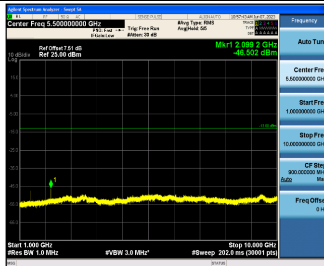
Band12-10MHz-16QAM-23060-1-0-Low-1000-10000--46.5-PASS
