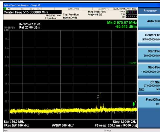
Band12-5MHz-16QAM-23155-1-0-Low-30-1000--60.44-PASS
