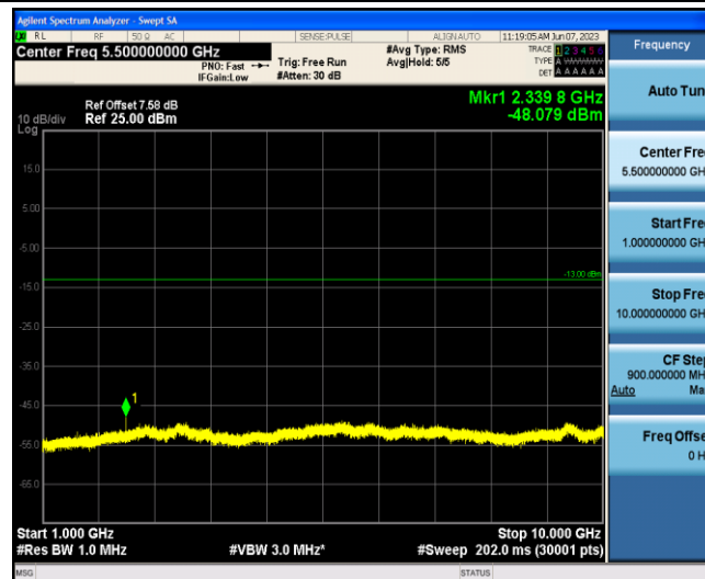
Band13-5MHz-16QAM-23230-1-0-Low-1000-10000--48.08-PASS
