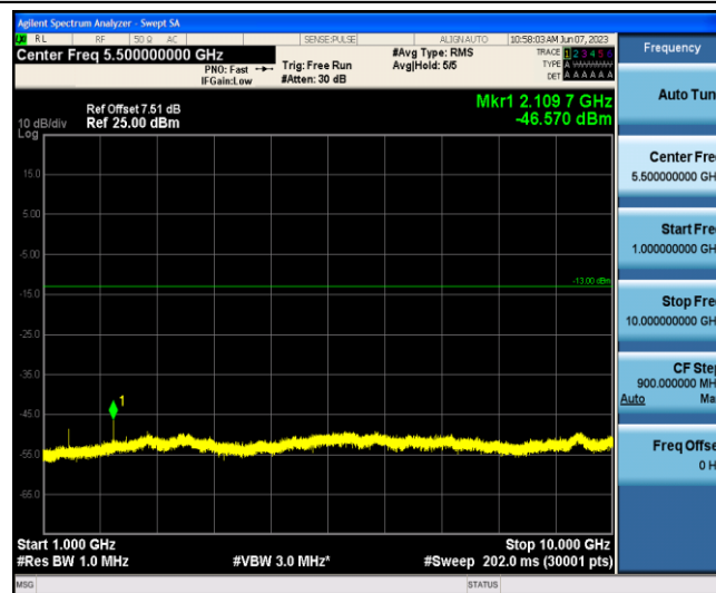
Band12-10MHz-QPSK-23095-1-0-Low-1000-10000--46.57-PASS
