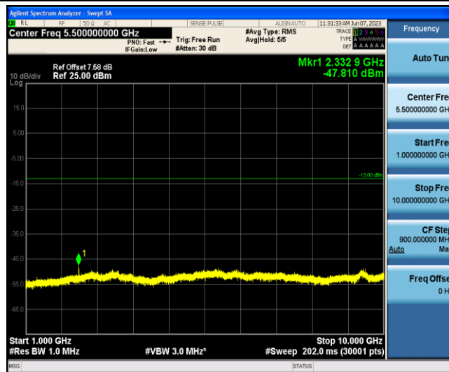
Band13-10MHz-16QAM-23230-1-0-Low-1000-10000--47.81-PASS
