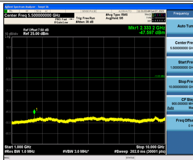
Band13-10MHz-QPSK-23230-1-0-Low-1000-10000--47.6-PASS
