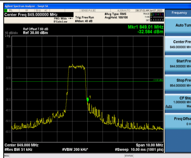
Band5-1.4MHz-16QAM-20643-6-0-High--32.58-PASS
