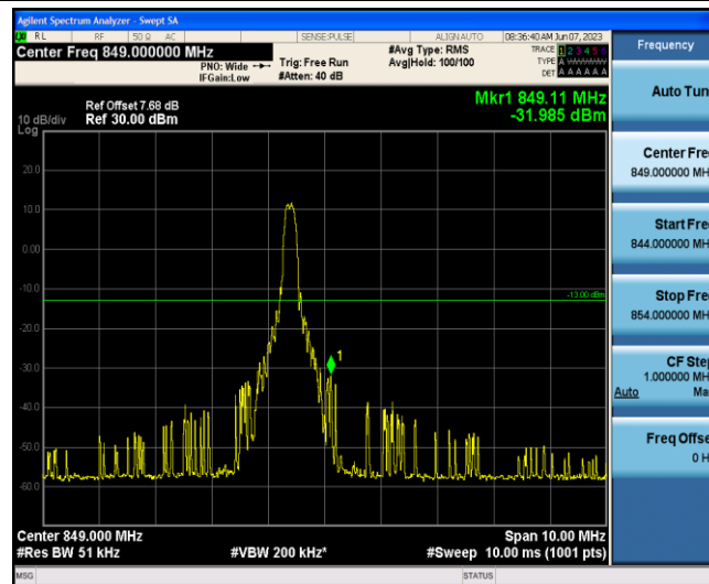
Band5-1.4MHz-16QAM-20643-1-5-High--31.99-PASS
