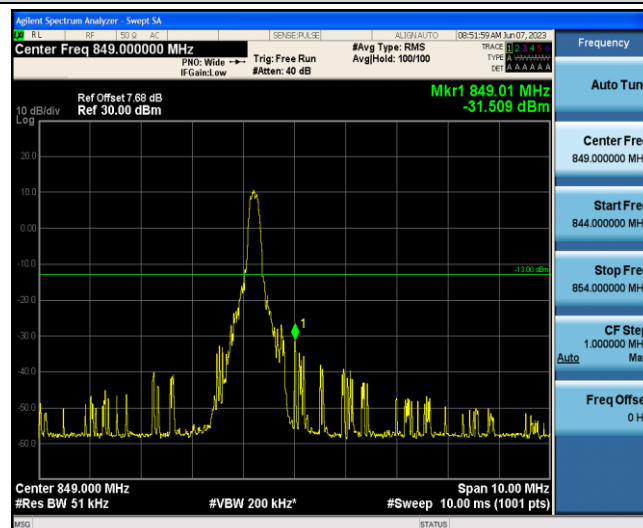
Band5-3MHz-16QAM-20635-1-5-High--31.51-PASS
