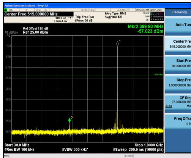
Band12-1.4MHz-QPSK-23095-1-0-Low-30-1000--57.02-PASS
