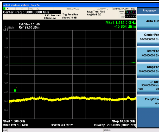
Band12-1.4MHz-16QAM-23095-1-0-Low-1000-10000--45.65-PASS
