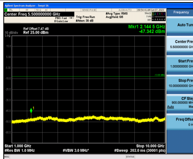
Band12-1.4MHz-QPSK-23173-1-0-Low-1000-10000--47.34-PASS
