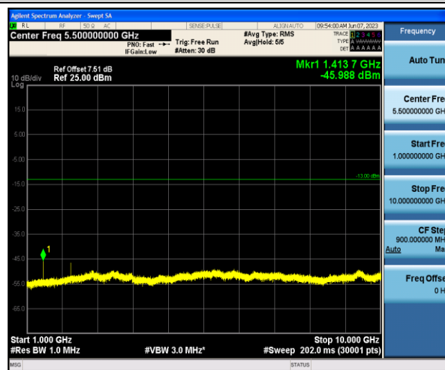
Band12-1.4MHz-QPSK-23095-1-0-Low-1000-10000--45.99-PASS
