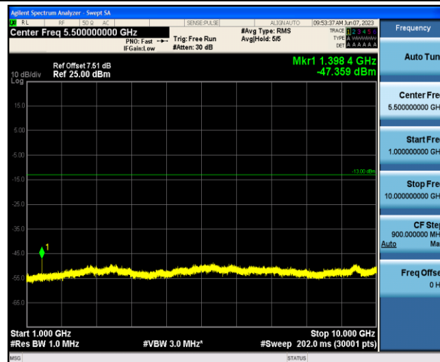
Band12-1.4MHz-16QAM-23017-1-0-Low-1000-10000--47.36-PASS
