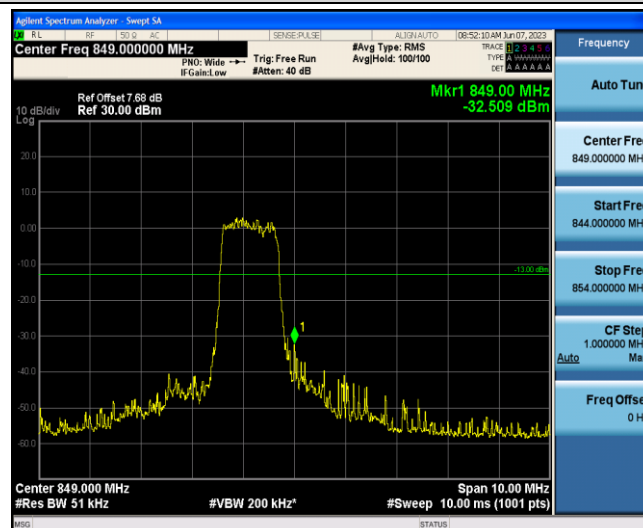
Band5-3MHz-QPSK-20635-6-0-High--32.51-PASS
