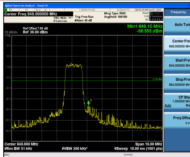
Band5-3MHz-16QAM-20635-6-0-High--36.56-PASS
