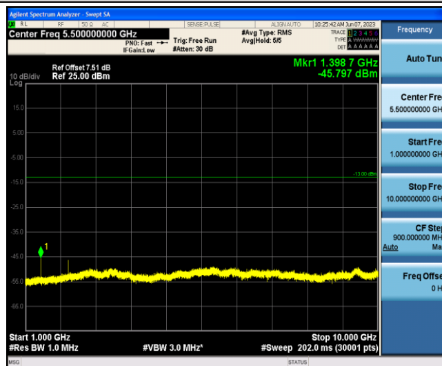
Band12-3MHz-QPSK-23025-1-0-Low-1000-10000--45.8-PASS
