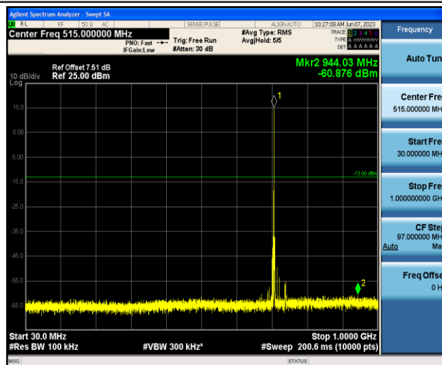
Band12-3MHz-16QAM-23165-1-0-Low-30-1000--60.88-PASS
