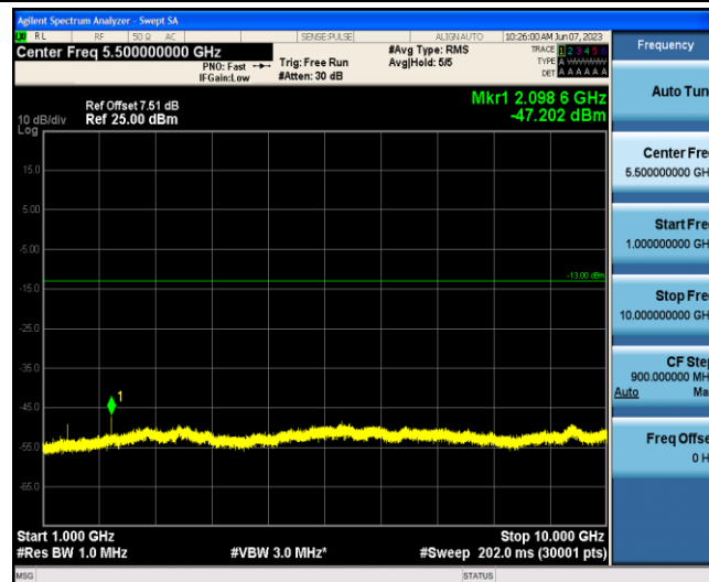
Band12-3MHz-16QAM-23025-1-0-Low-1000-10000--47.2-PASS
