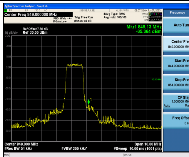
Band5-5MHz-QPSK-20625-6-0-High--35.36-PASS
