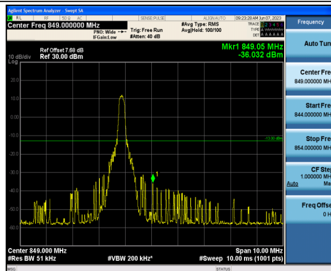
Band5-10MHz-QPSK-20600-1-5-High--36.03-PASS
