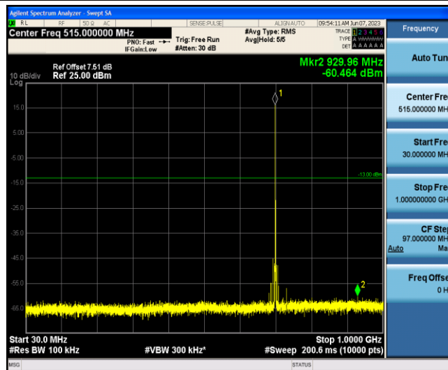
Band12-1.4MHz-16QAM-23095-1-0-Low-30-1000--60.46-PASS
