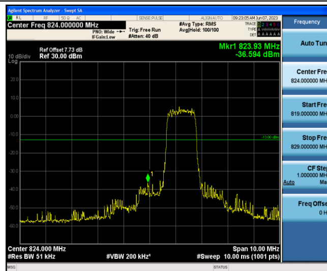
Band5-10MHz-QPSK-20450-6-0-Low--36.59-PASS
