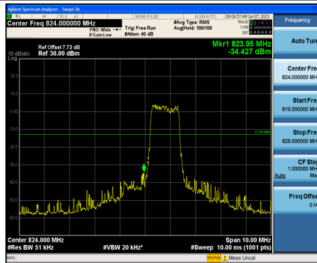
Band5-5MHz-16QAM-20425-6-0-Low--34.43-PASS
