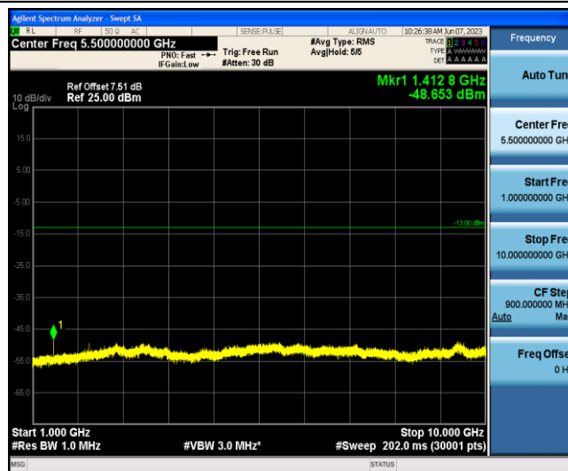
Band12-3MHz-16QAM-23095-1-0-Low-1000-10000--48.65-PASS
