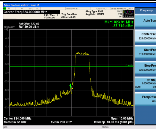
Band5-3MHz-16QAM-20415-6-0-Low--37.72-PASS
