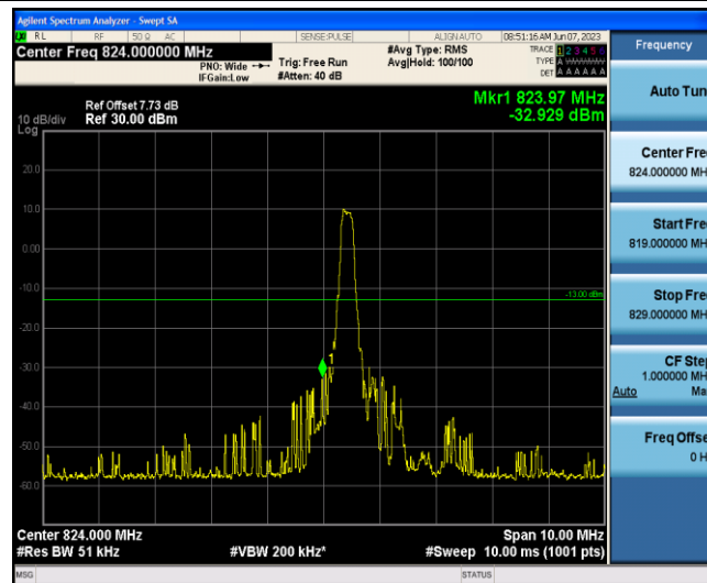
Band5-3MHz-16QAM-20415-1-0-Low--32.93-PASS
