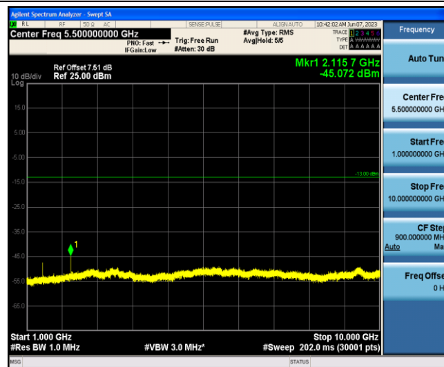
Band12-5MHz-QPSK-23095-1-0-Low-1000-10000--45.07-PASS
