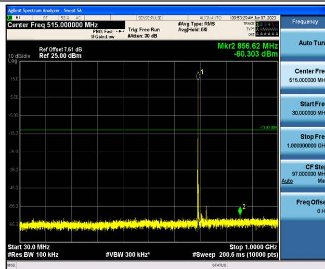
Band12-1.4MHz-16QAM-23017-1-0-Low-30-1000--60.3-PASS
