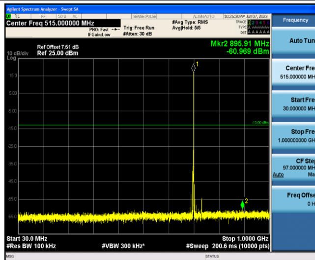
Band12-3MHz-16QAM-23095-1-0-Low-30-1000--60.97-PASS
