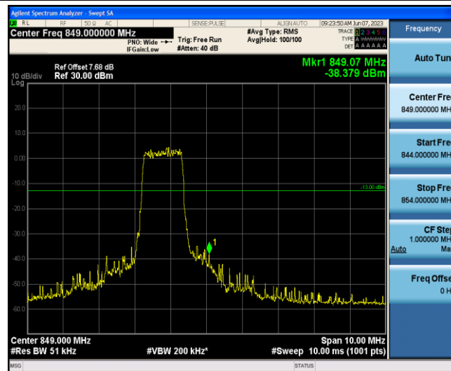
Band5-10MHz-QPSK-20600-6-0-High--38.38-PASS
