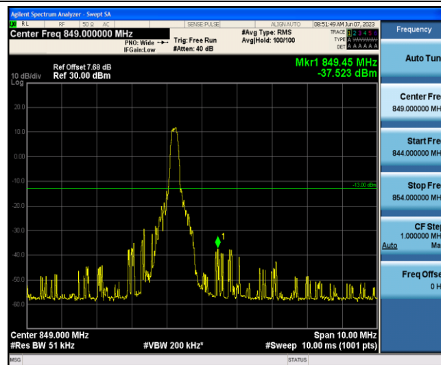
Band5-3MHz-QPSK-20635-1-5-High--37.52-PASS
