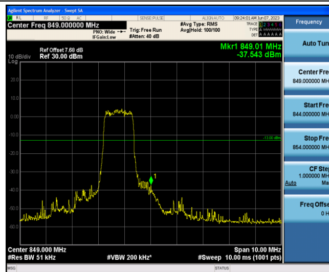
Band5-10MHz-16QAM-20600-6-0-High--37.54-PASS
