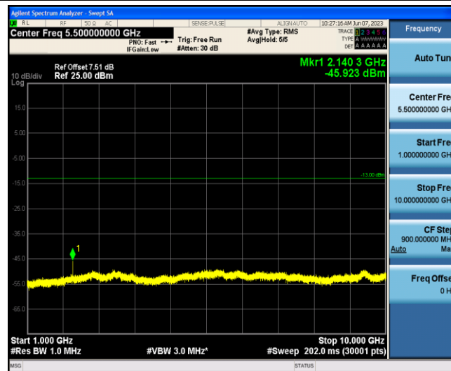
Band12-3MHz-16QAM-23165-1-0-Low-1000-10000--45.92-PASS
