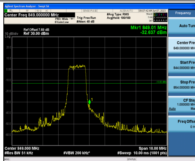
Band5-5MHz-16QAM-20625-6-0-High--32.64-PASS
