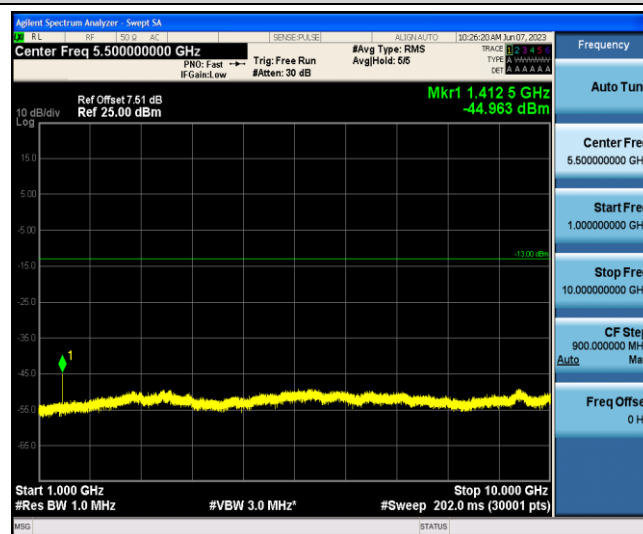
Band12-3MHz-QPSK-23095-1-0-Low-1000-10000--44.96-PASS
