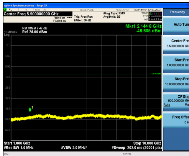
Band12-1.4MHz-16QAM-23173-1-0-Low-1000-10000--48.61-PASS
