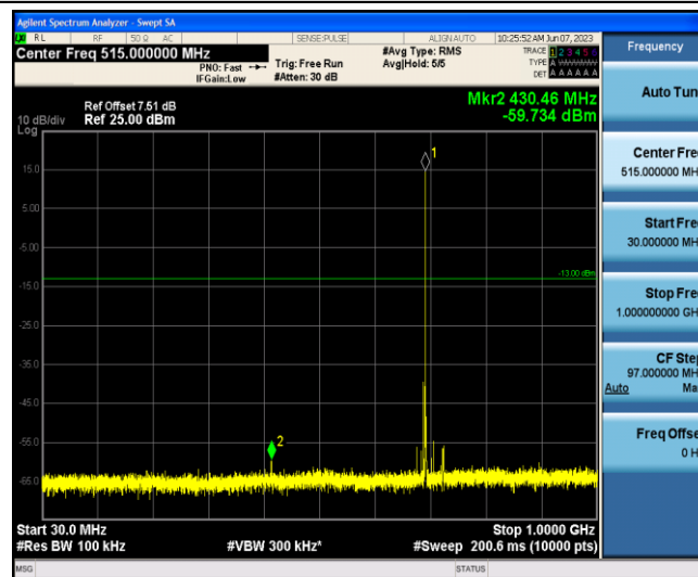
Band12-3MHz-16QAM-23025-1-0-Low-30-1000--59.73-PASS
