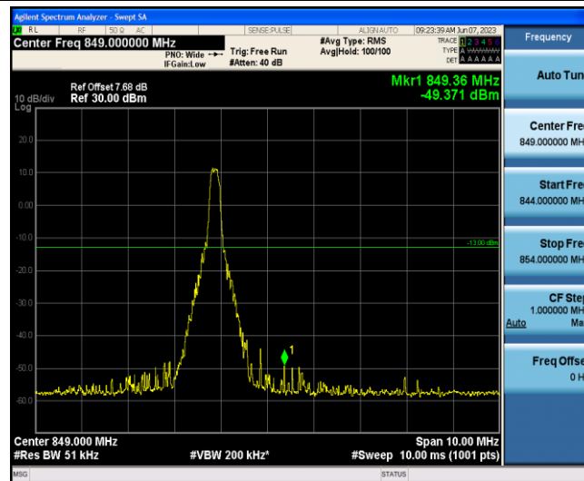
Band5-10MHz-16QAM-20600-1-5-High--49.37-PASS
