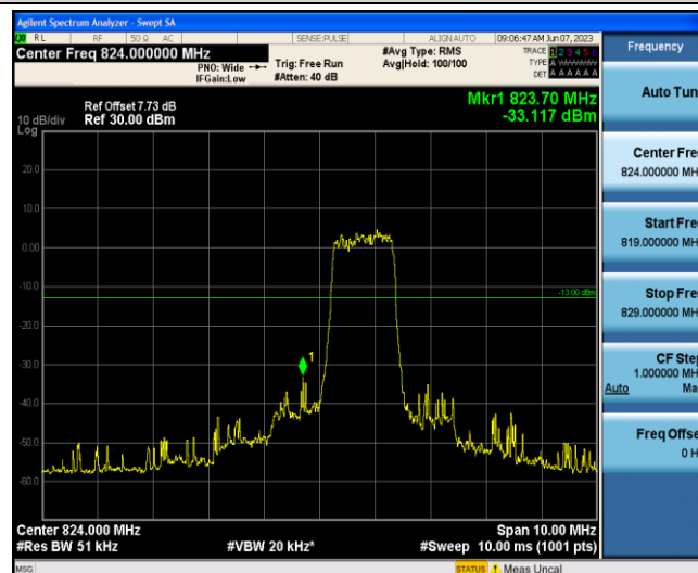
Band5-5MHz-QPSK-20425-6-0-Low--33.12-PASS
