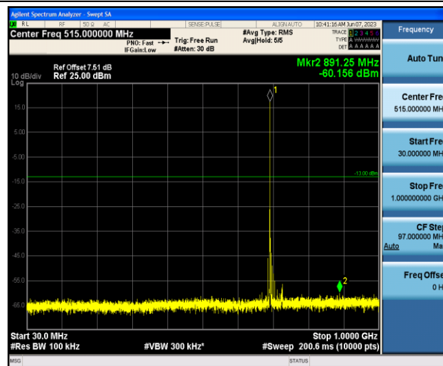
Band12-5MHz-QPSK-23035-1-0-Low-30-1000--60.16-PASS
