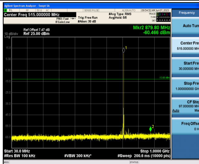
Band12-1.4MHz-16QAM-23173-1-0-Low-30-1000--60.47-PASS
