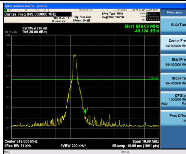
Band5-5MHz-16QAM-20625-1-5-High--46.12-PASS
