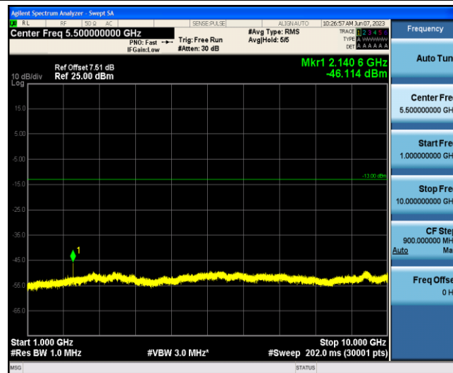
Band12-3MHz-QPSK-23165-1-0-Low-1000-10000--46.11-PASS
