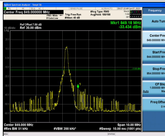
Band5-5MHz-QPSK-20625-1-5-High--33.43-PASS
