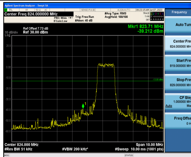
Band5-10MHz-16QAM-20450-6-0-Low--39.21-PASS
