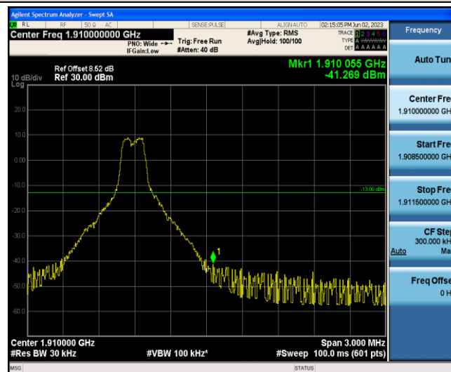
Band2-1.4MHz-QPSK-19193-1-5-High--41.27-PASS
