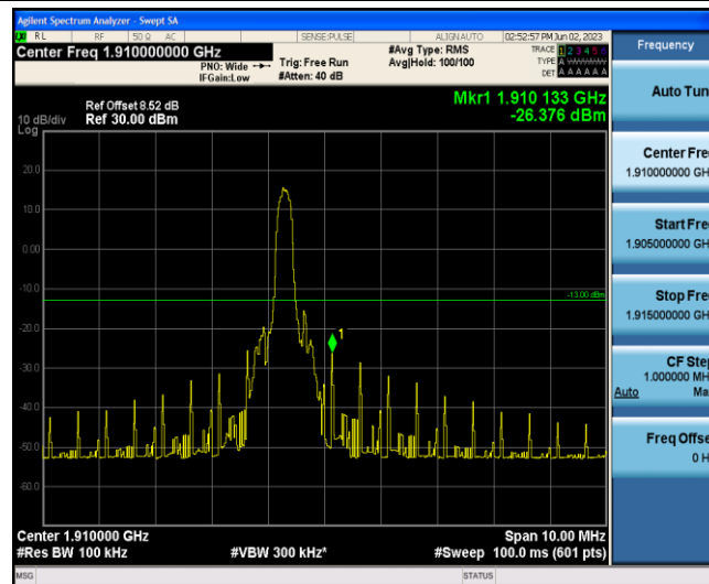
Band2-5MHz-QPSK-19175-1-5-High--26.38-PASS
