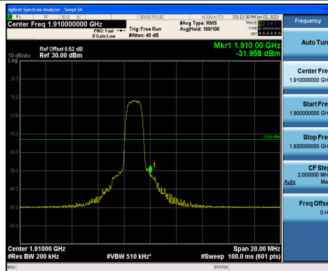
Band2-10MHz-QPSK-19150-6-0-High--31.96-PASS
