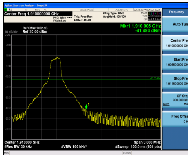
Band2-1.4MHz-16QAM-19193-1-5-High--41.49-PASS
