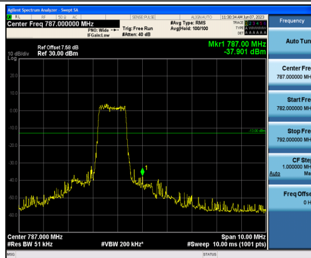
Band13-10MHz-QPSK-23230-6-0-High--37.90-PASS
