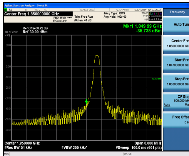
Band2-3MHz-16QAM-18615-1-0-Low--35.74-PASS
