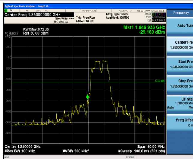
Band2-5MHz-QPSK-18625-6-0-Low--29.17-PASS
