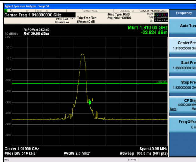
Band2-20MHz-QPSK-19100-6-0-High--32.82-PASS
