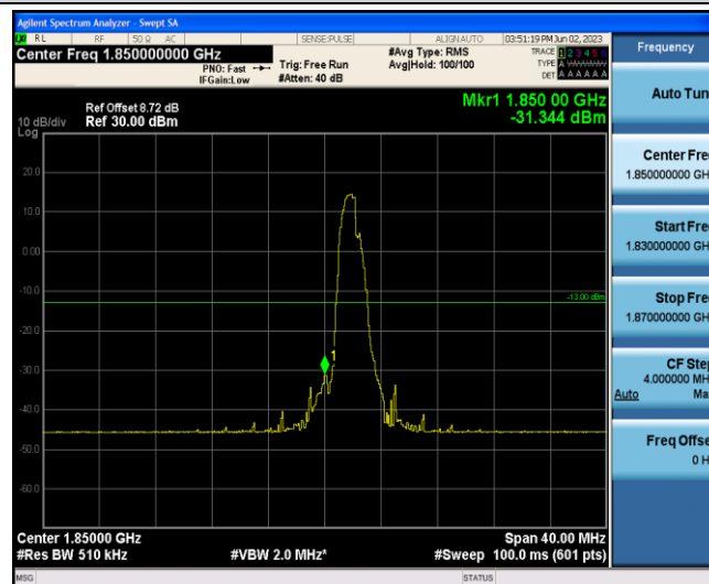
Band2-20MHz-QPSK-18700-6-0-Low--31.34-PASS
