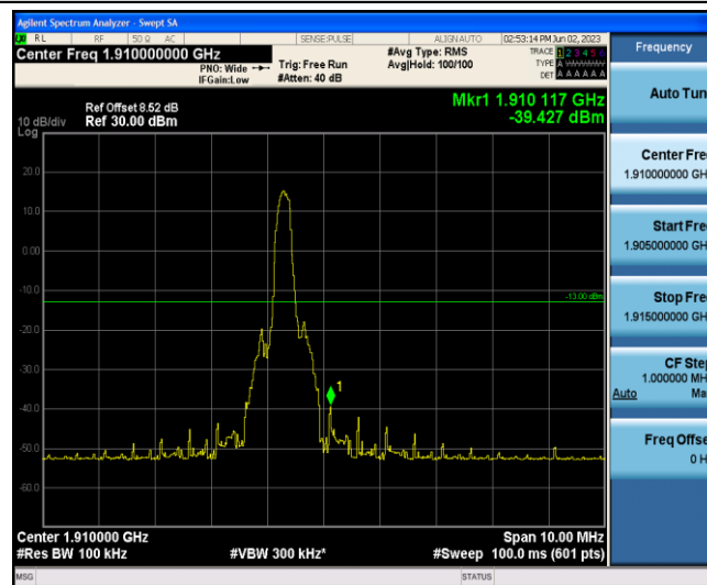
Band2-5MHz-16QAM-19175-1-5-High--39.43-PASS
