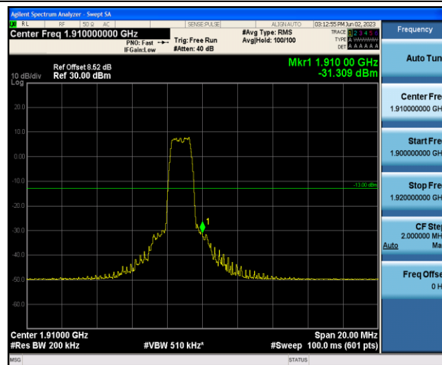
Band2-10MHz-16QAM-19150-6-0-High--31.31-PASS
