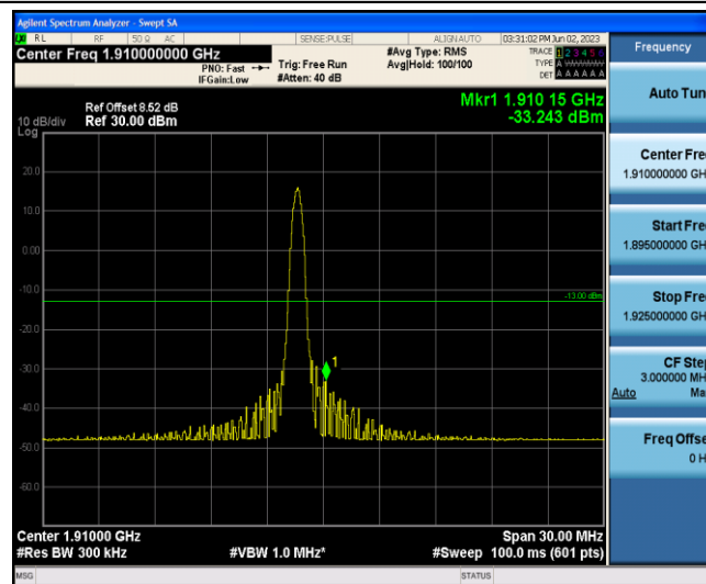
Band2-15MHz-QPSK-19125-1-5-High--33.24-PASS
