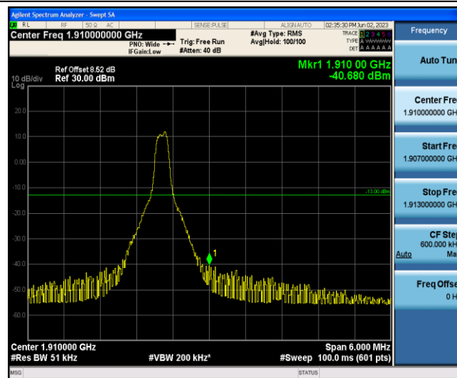
Band2-3MHz-QPSK-19185-1-5-High--40.68-PASS
