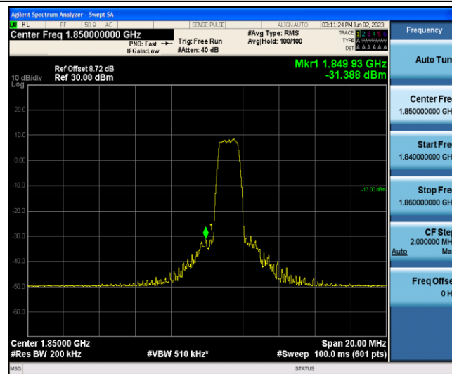
Band2-10MHz-QPSK-18650-6-0-Low--31.39-PASS
