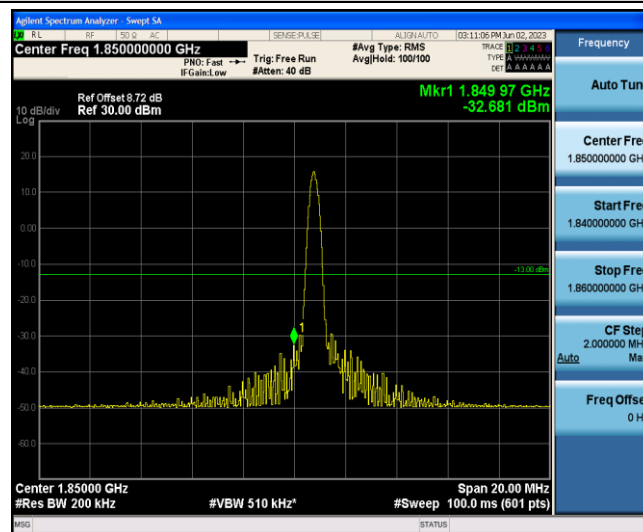
Band2-10MHz-16QAM-18650-1-0-Low--32.68-PASS
