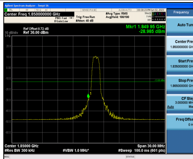
Band2-15MHz-QPSK-18675-6-0-Low--28.98-PASS
