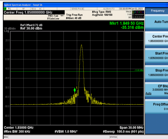
Band2-15MHz-16QAM-18675-1-0-Low--35.32-PASS
