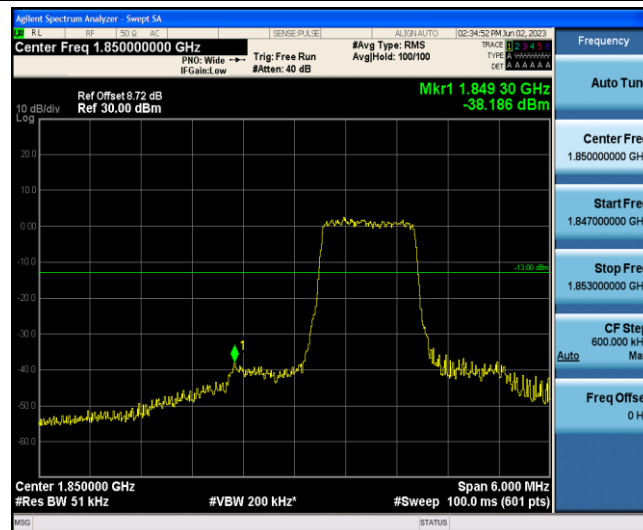
Band2-3MHz-QPSK-18615-6-0-Low--38.19-PASS
