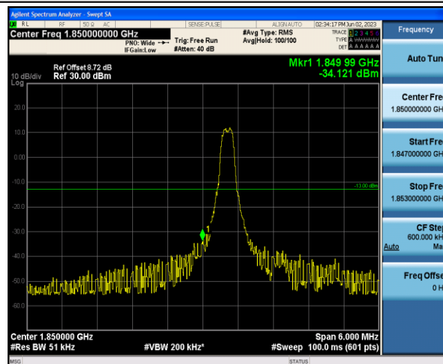
Band2-3MHz-QPSK-18615-1-0-Low--34.12-PASS
