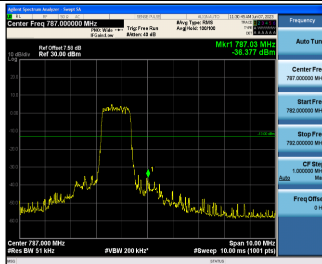
Band13-10MHz-16QAM-23230-6-0-High--36.38-PASS
