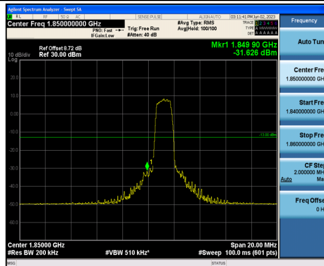
Band2-10MHz-16QAM-18650-6-0-Low--31.63-PASS
