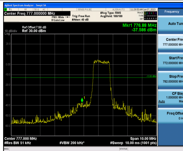
Band13-10MHz-QPSK-23230-6-0-Low--37.59-PASS
