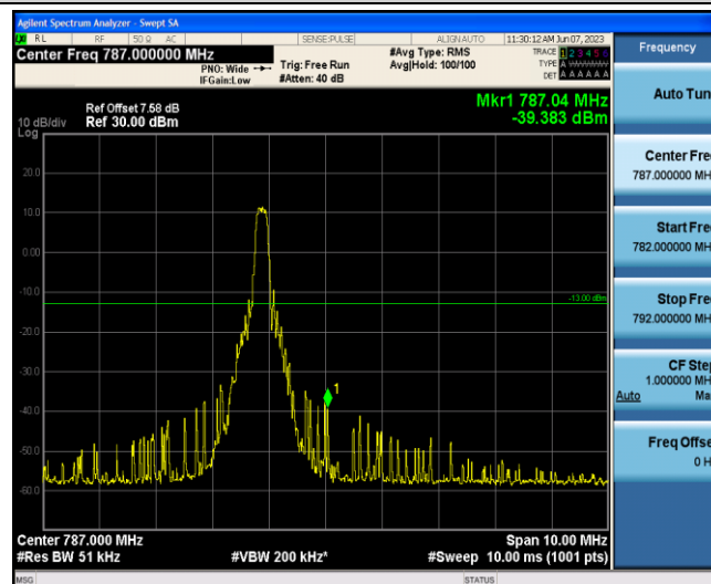
Band13-10MHz-QPSK-23230-1-5-High--39.38-PASS
