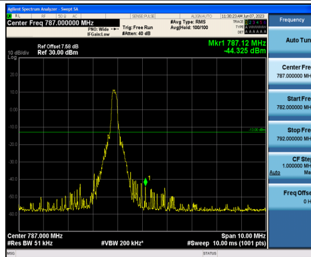
Band13-10MHz-16QAM-23230-1-5-High--44.32-PASS
