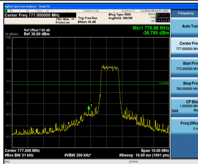
Band13-10MHz-16QAM-23230-6-0-Low--36.80-PASS
