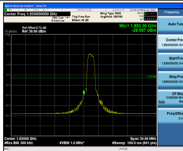
Band2-15MHz-16QAM-18675-6-0-Low--29.60-PASS
