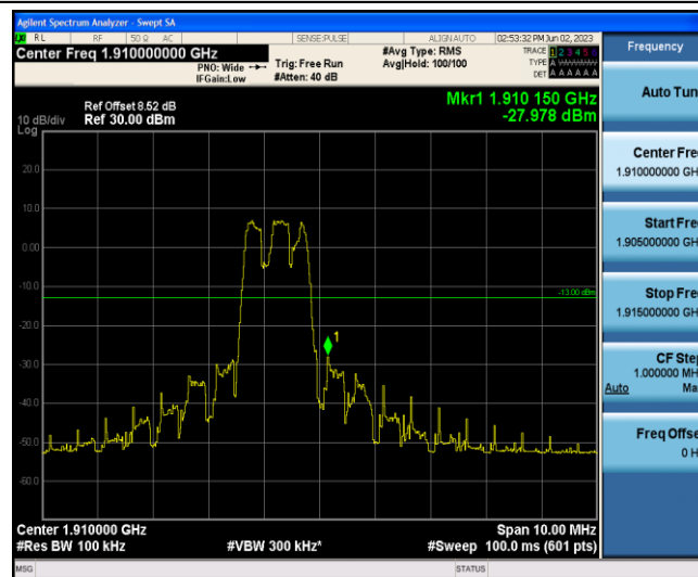
Band2-5MHz-QPSK-19175-6-0-High--27.98-PASS
