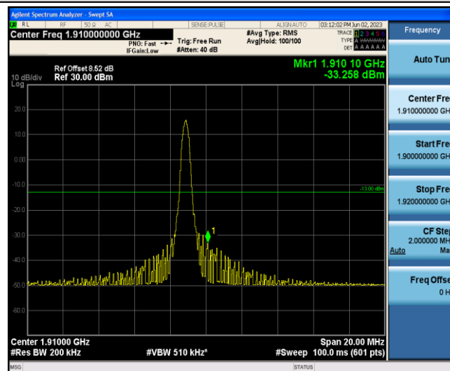
Band2-10MHz-QPSK-19150-1-5-High--33.26-PASS
