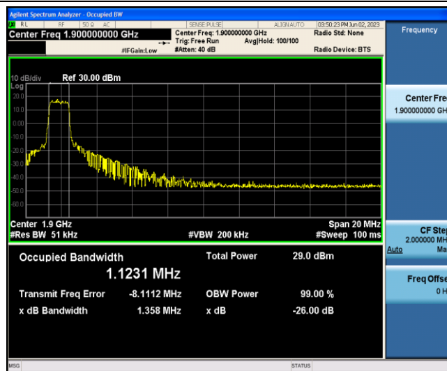
Band2-20MHz-16QAM-19100-6-0-Low-1.1231-1.358-PASS
