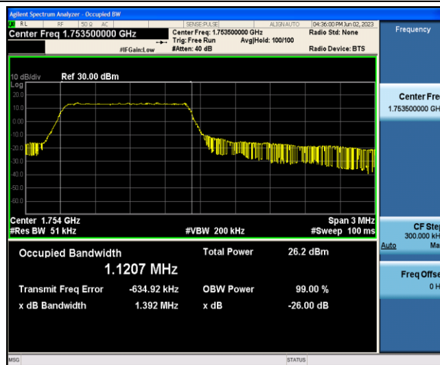
Band4-3MHz-QPSK-20385-6-0-Low-1.1207-1.392-PASS
