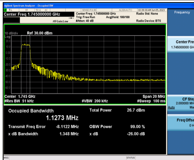
Band4-20MHz-16QAM-20300-6-0-Low-1.1273-1.348-PASS
