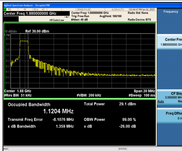
Band2-20MHz-16QAM-18900-6-0-Low-1.1204-1.359-PASS
