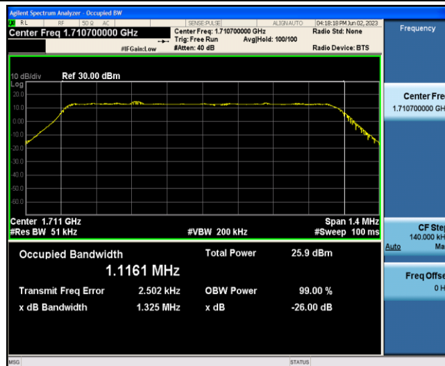
Band4-1.4MHz-16QAM-19957-6-0-Low-1.1161-1.325-PASS
