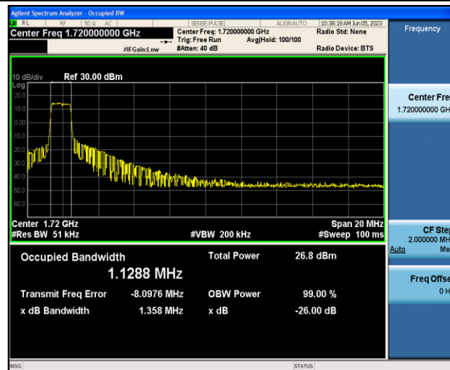
Band4-20MHz-16QAM-20050-6-0-Low-1.1288-1.358-PASS
