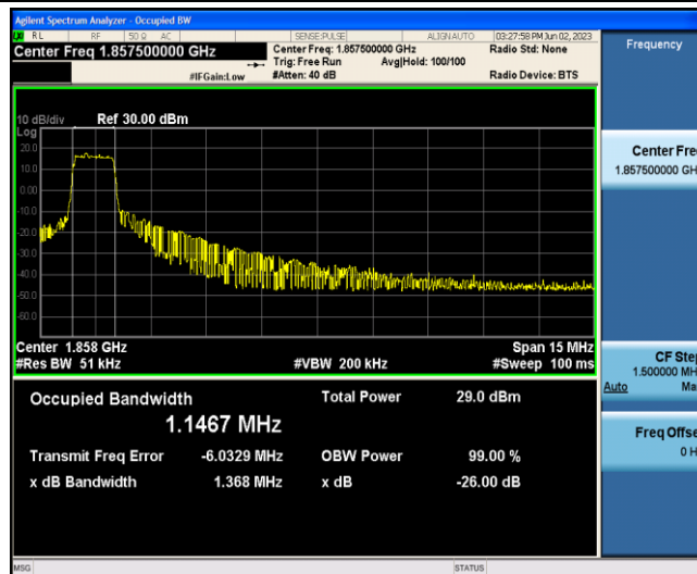
Band2-15MHz-QPSK-18675-6-0-Low-1.1467-1.368-PASS
