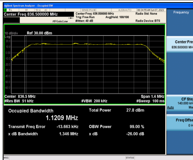
Band5-1.4MHz-16QAM-20525-6-0-Low-1.1209-1.346-PASS
