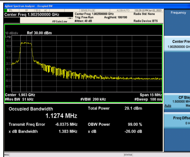
Band2-15MHz-QPSK-19125-6-0-Low-1.1274-1.383-PASS
