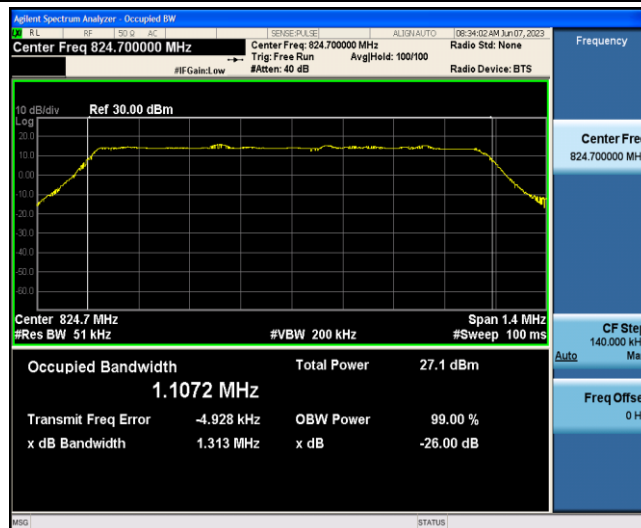
Band5-1.4MHz-QPSK-20407-6-0-Low-1.1072-1.313-PASS
