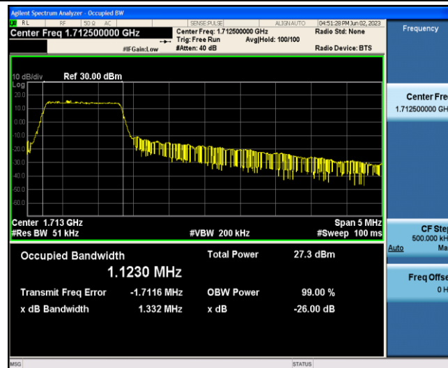
Band4-5MHz-16QAM-19975-6-0-Low-1.1230-1.332-PASS
