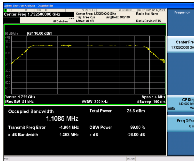
Band4-1.4MHz-16QAM-20175-6-0-Low-1.1085-1.363-PASS
