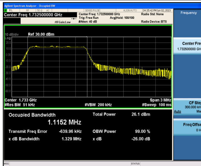
Band4-3MHz-16QAM-20175-6-0-Low-1.1152-1.329-PASS
