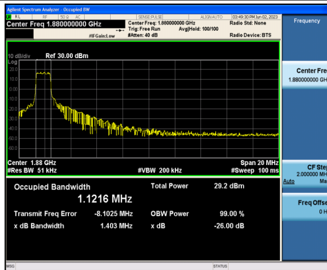
Band2-20MHz-QPSK-18900-6-0-Low-1.1216-1.403-PASS
