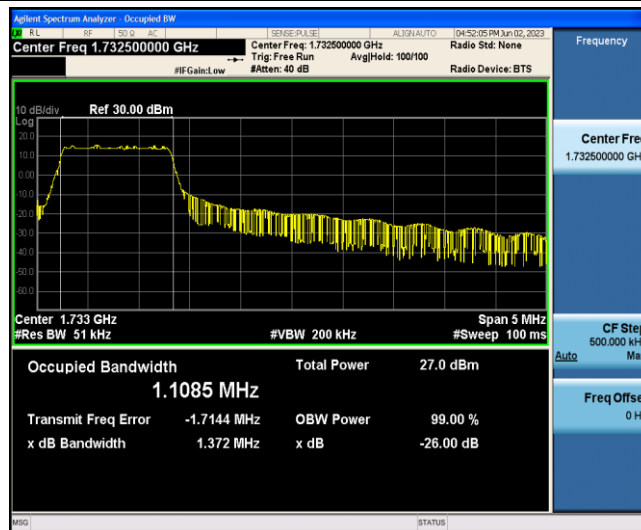
Band4-5MHz-16QAM-20175-6-0-Low-1.1085-1.372-PASS
