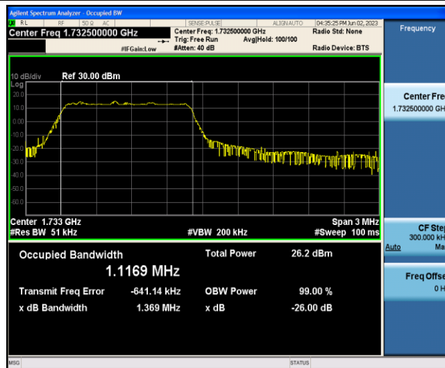
Band4-3MHz-QPSK-20175-6-0-Low-1.1169-1.369-PASS
