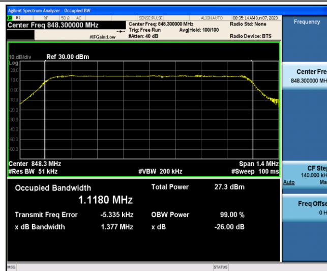
Band5-1.4MHz-QPSK-20643-6-0-Low-1.1180-1.377-PASS
