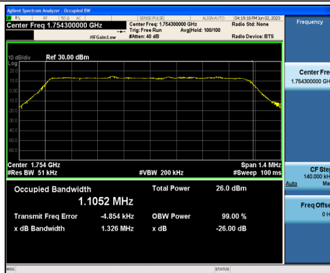
Band4-1.4MHz-QPSK-20393-6-0-Low-1.1052-1.326-PASS
