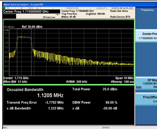
Band4-10MHz-QPSK-20000-6-0-Low-1.1205-1.322-PASS
