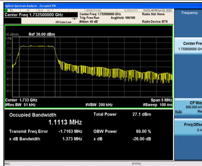
Band4-5MHz-QPSK-20175-6-0-Low-1.1113-1.373-PASS
