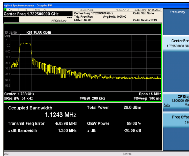
Band4-15MHz-QPSK-20175-6-0-Low-1.1243-1.350-PASS
