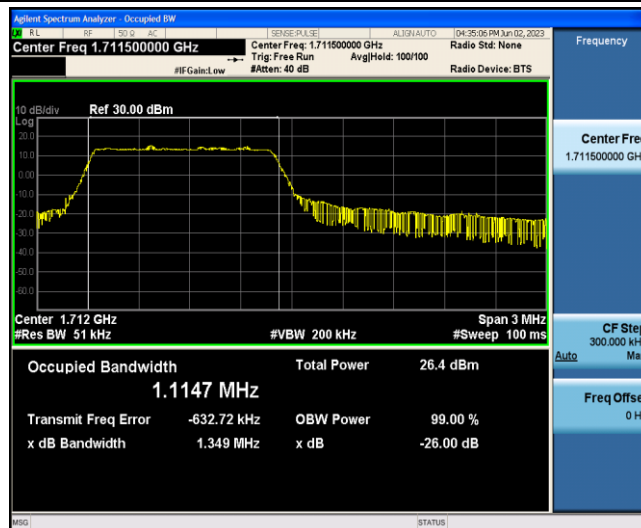
Band4-3MHz-16QAM-19965-6-0-Low-1.1147-1.349-PASS
