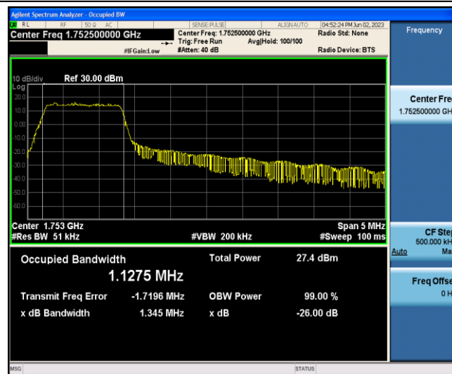
Band4-5MHz-QPSK-20375-6-0-Low-1.1275-1.345-PASS
