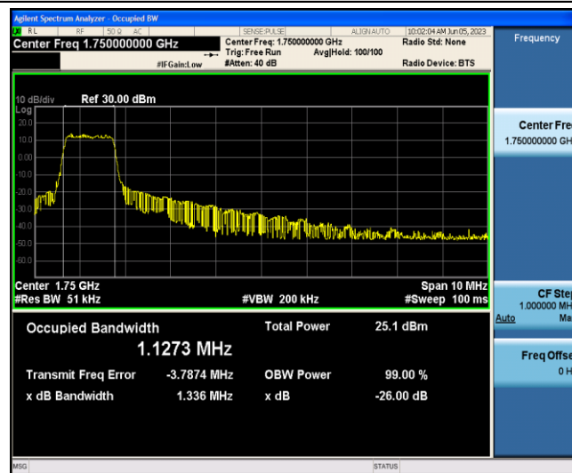
Band4-10MHz-QPSK-20350-6-0-Low-1.1273-1.336-PASS
