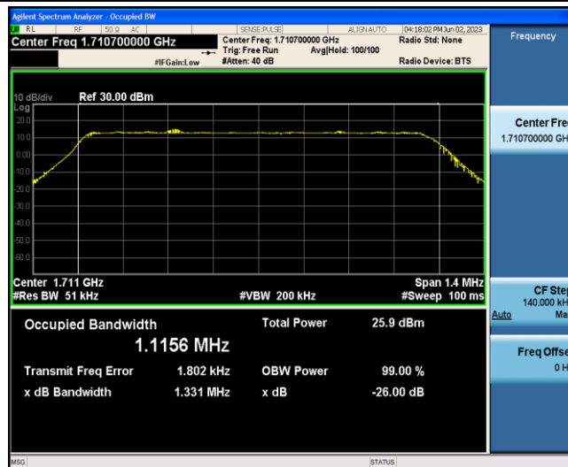
Band4-1.4MHz-QPSK-19957-6-0-Low-1.1156-1.331-PASS
