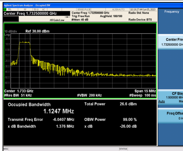
Band4-15MHz-16QAM-20175-6-0-Low-1.1247-1.376-PASS
