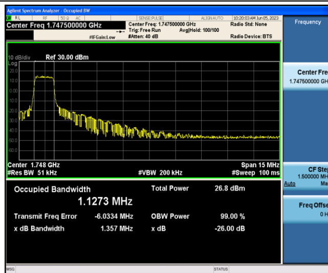
Band4-15MHz-16QAM-20325-6-0-Low-1.1273-1.357-PASS
