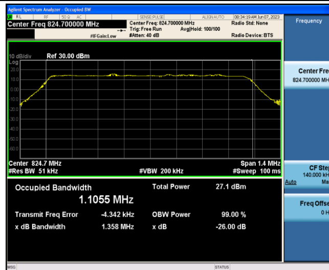
Band5-1.4MHz-16QAM-20407-6-0-Low-1.1055-1.358-PASS
