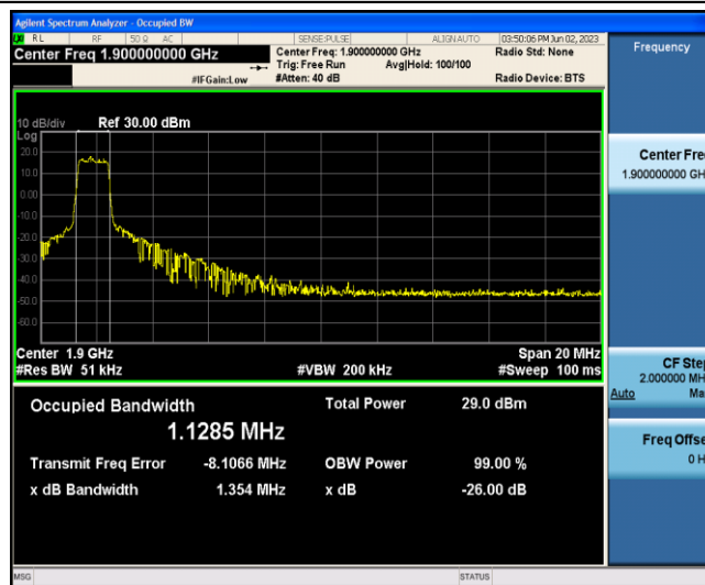
Band2-20MHz-QPSK-19100-6-0-Low-1.1285-1.354-PASS
