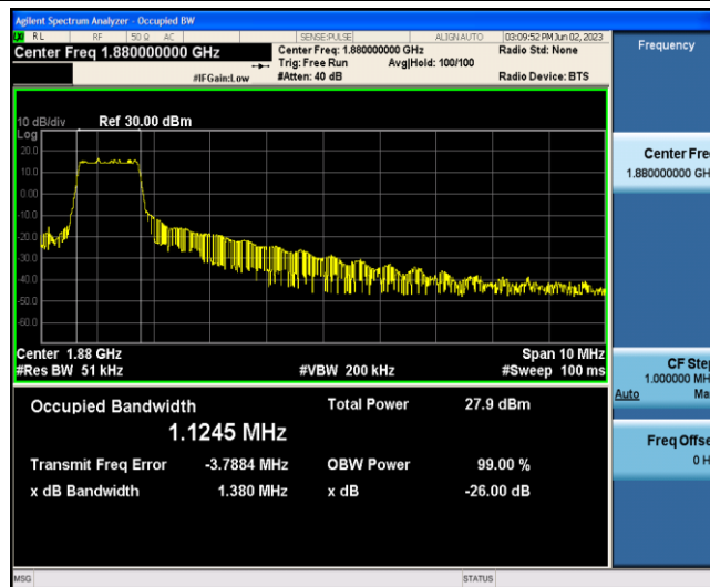
Band2-10MHz-16QAM-18900-6-0-Low-1.1245-1.380-PASS
