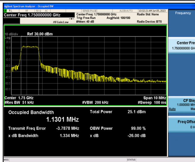
Band4-10MHz-16QAM-20350-6-0-Low-1.1301-1.334-PASS
