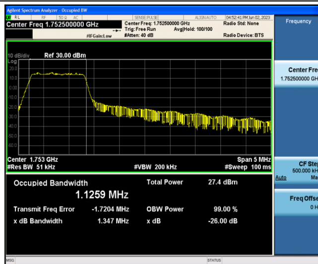
Band4-5MHz-16QAM-20375-6-0-Low-1.1259-1.347-PASS
