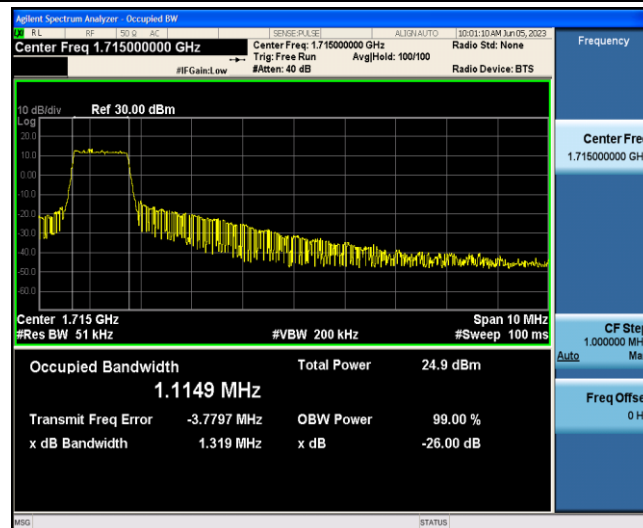
Band4-10MHz-16QAM-20000-6-0-Low-1.1149-1.319-PASS
