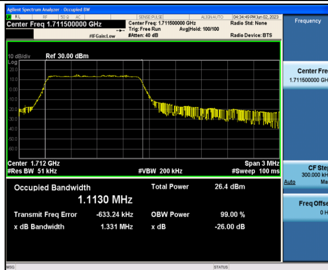
Band4-3MHz-QPSK-19965-6-0-Low-1.1130-1.331-PASS
