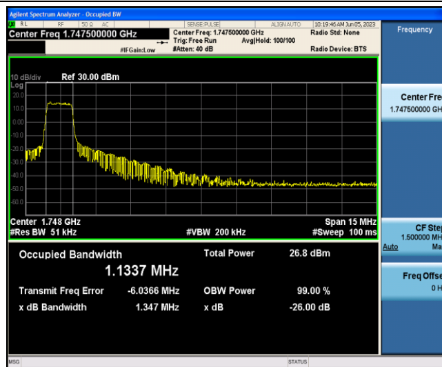
Band4-15MHz-QPSK-20325-6-0-Low-1.1337-1.347-PASS
