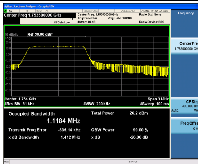
Band4-3MHz-16QAM-20385-6-0-Low-1.1184-1.412-PASS
