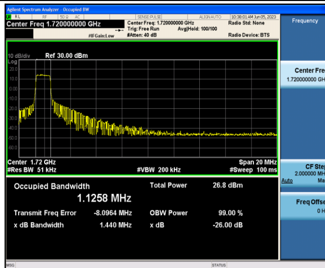
Band4-20MHz-QPSK-20050-6-0-Low-1.1258-1.440-PASS
