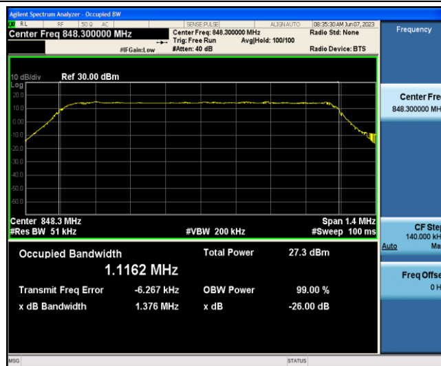
Band5-1.4MHz-16QAM-20643-6-0-Low-1.1162-1.376-PASS
