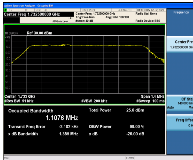
Band4-1.4MHz-QPSK-20175-6-0-Low-1.1076-1.355-PASS
