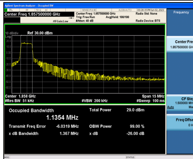
Band2-15MHz-16QAM-18675-6-0-Low-1.1354-1.367-PASS
