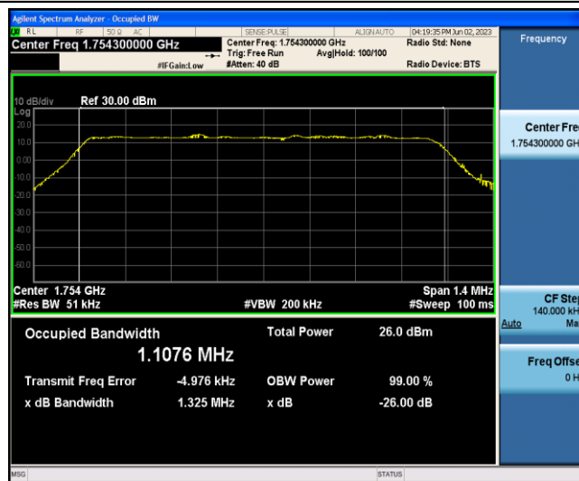
Band4-1.4MHz-16QAM-20393-6-0-Low-1.1076-1.325-PASS
