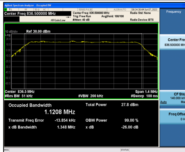
Band5-1.4MHz-QPSK-20525-6-0-Low-1.1208-1.348-PASS
