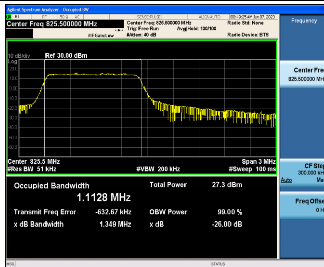
Band5-3MHz-QPSK-20415-6-0-Low-1.1128-1.349-PASS
