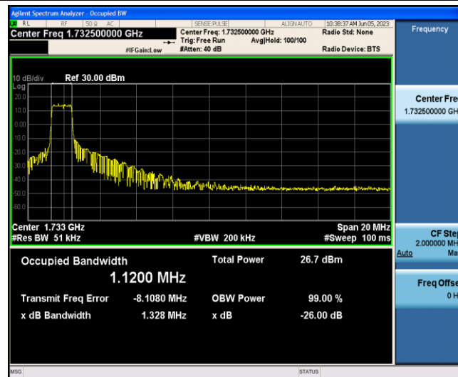
Band4-20MHz-QPSK-20175-6-0-Low-1.1200-1.328-PASS
