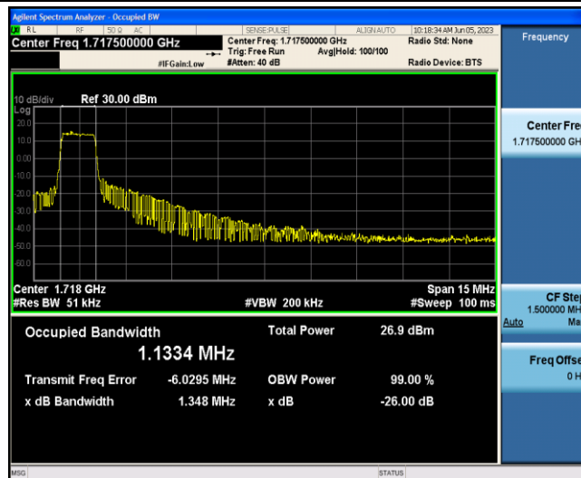
Band4-15MHz-QPSK-20025-6-0-Low-1.1334-1.348-PASS
