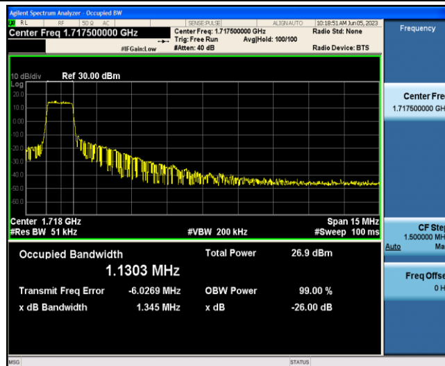
Band4-15MHz-16QAM-20025-6-0-Low-1.1303-1.345-PASS
