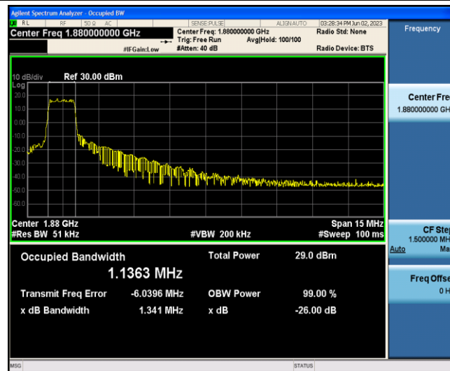
Band2-15MHz-QPSK-18900-6-0-Low-1.1363-1.341-PASS
