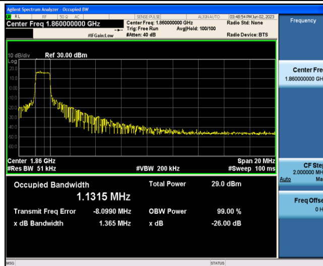
Band2-20MHz-QPSK-18700-6-0-Low-1.1315-1.365-PASS
