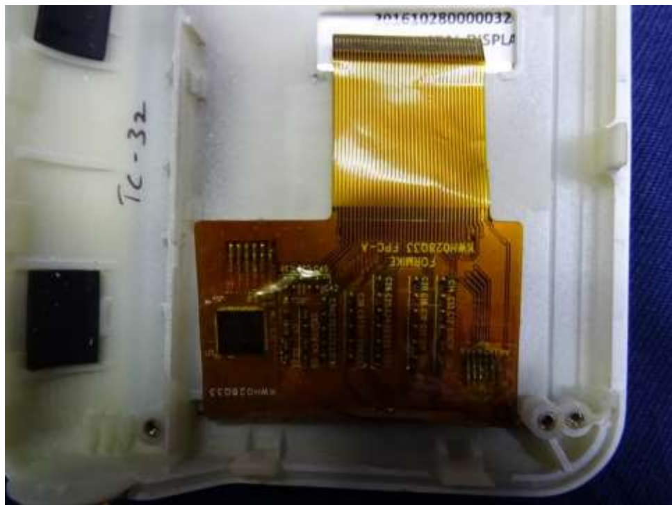
Internal display cable.
