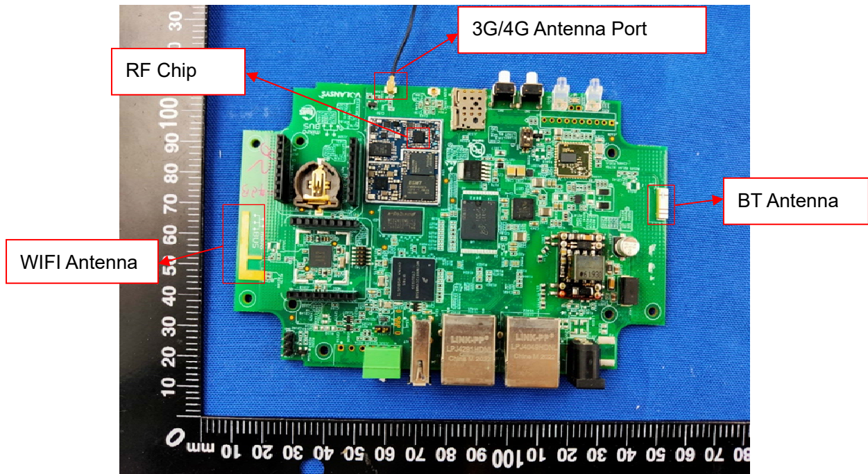
MAIN BOARD TOP VIEW(WITHOUT SHIELDING)
