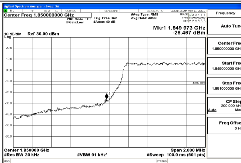
Band25-1.4MHz-16QAM-26683-6RB#0
