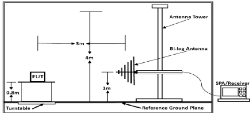
Below 1GHz
