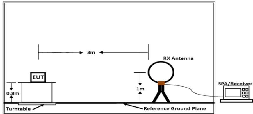
Below 30MHz
