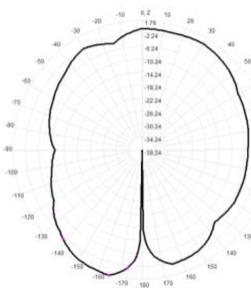
915MHZ, Total=YZ, Max=1.5dBi
