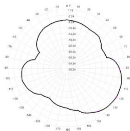
915MHZ, Total=XZ, Max=0.78dBi
