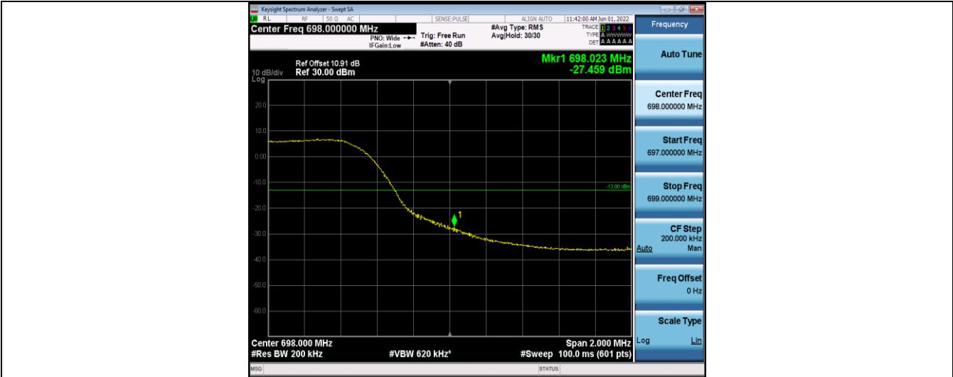
Band71-10MHz-16QAM-133172-50RB#0
