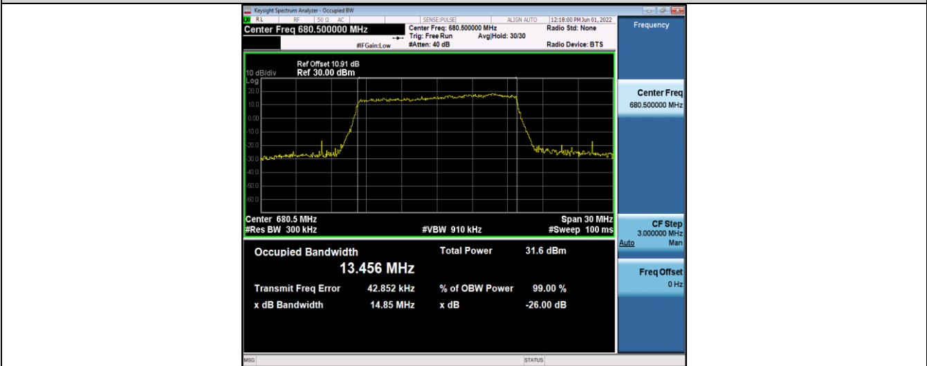
Band71-15MHz-16QAM-133397-75RB#0
