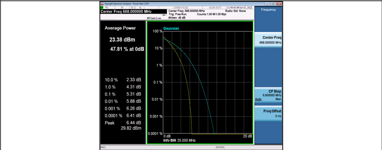
Band71-10MHz-QPSK-133297-50RB#0
