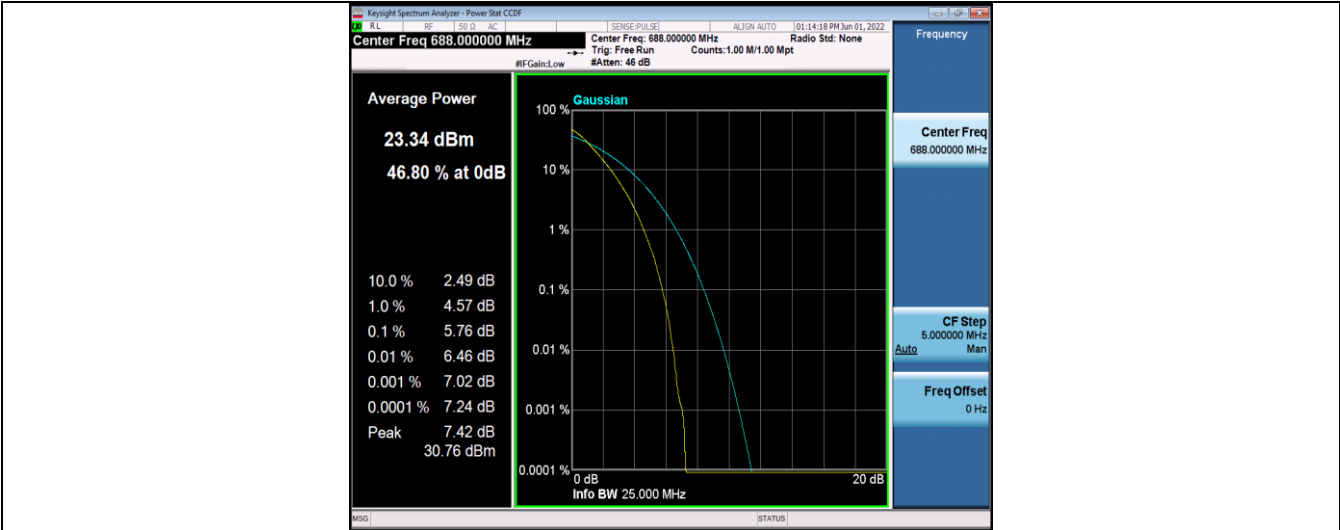
Band71-20MHz-16QAM-133222-100RB#0
