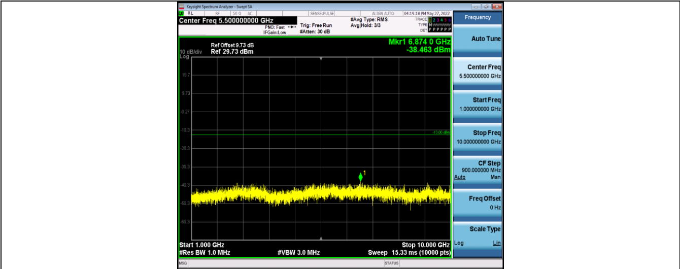
Band26-3MHz-16QAM-26805-15RB#0-Range1:30~1000MHz
