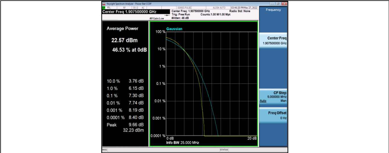
Band25-15MHz-16QAM-26115-75RB#0
