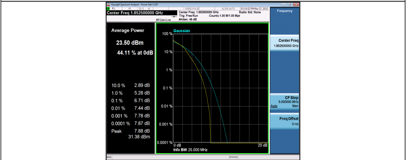
Band25-5MHz-16QAM-26365-25RB#0
