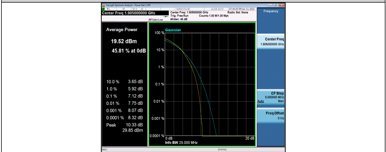
Band2-15MHz-QPSK-18675-75RB#0
