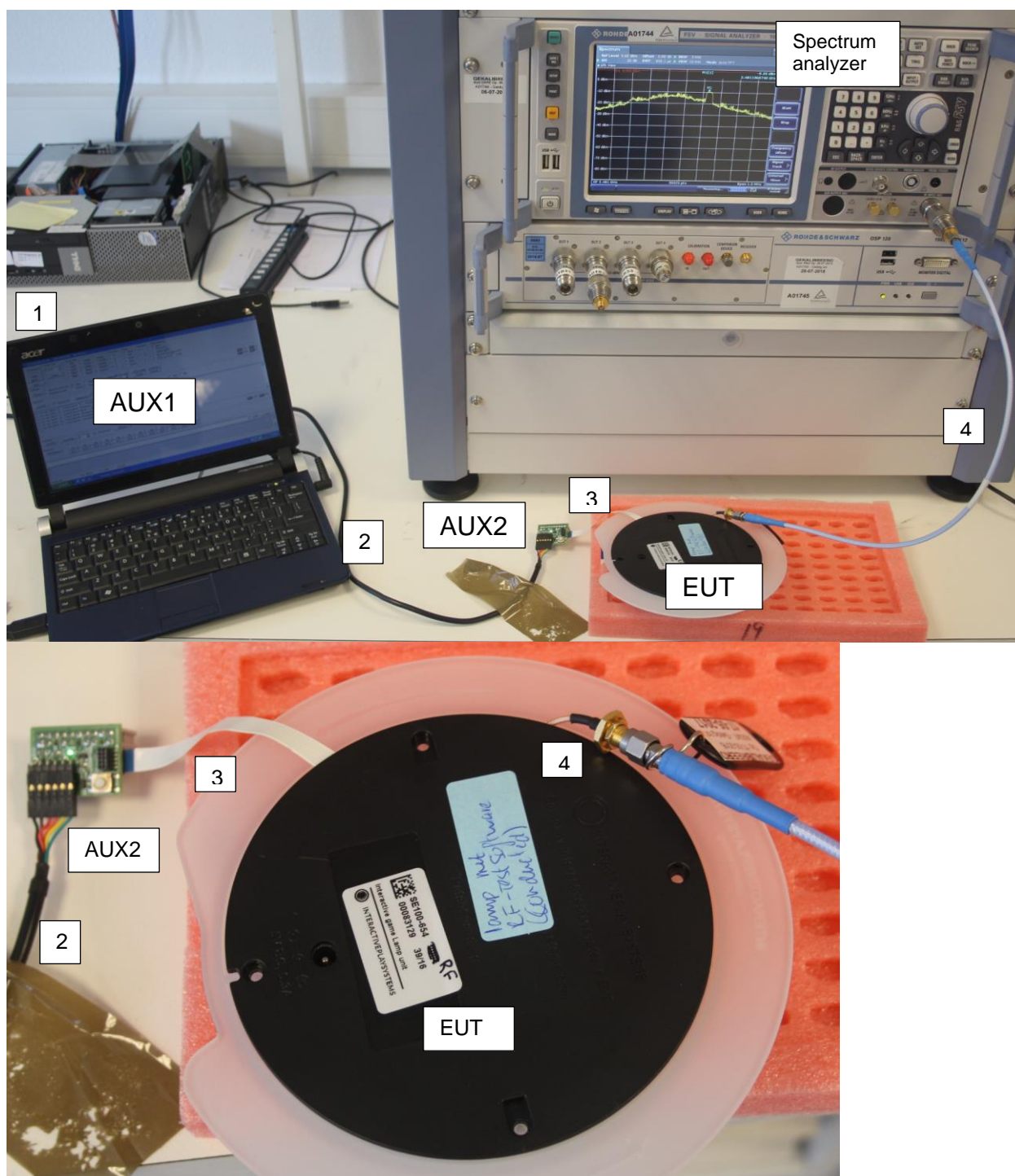
Figure 2b: Test Setup Photos – conducted tests and programming.
