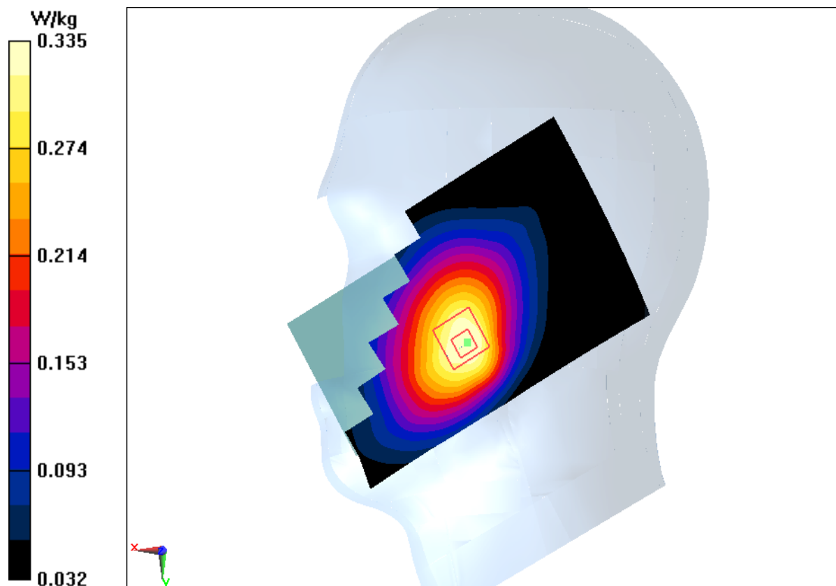
Fig.7 LTE Band5
