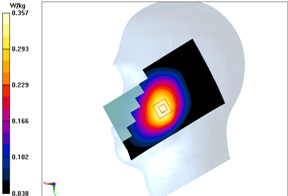
Fig.1 850MHz
