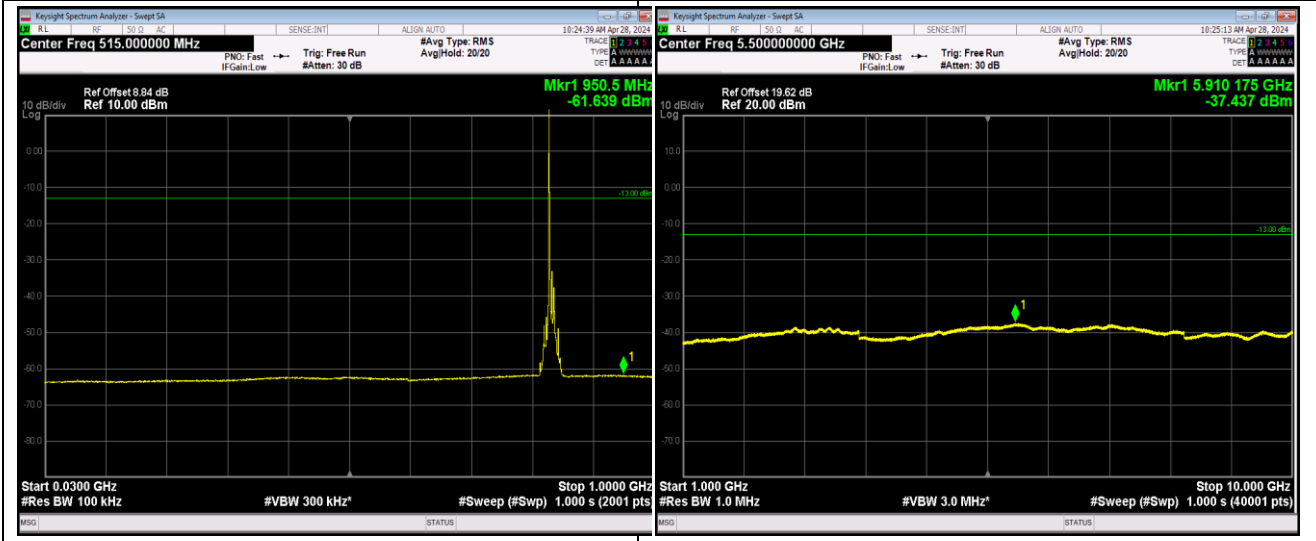
Band5_10MHz_QPSK_20525_1RB#0_30~1000_30~10
