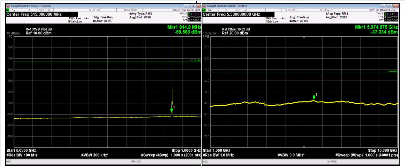
Band5_1.4MHz_64QAM_20643_1RB#0_30~1000_30~1 000
