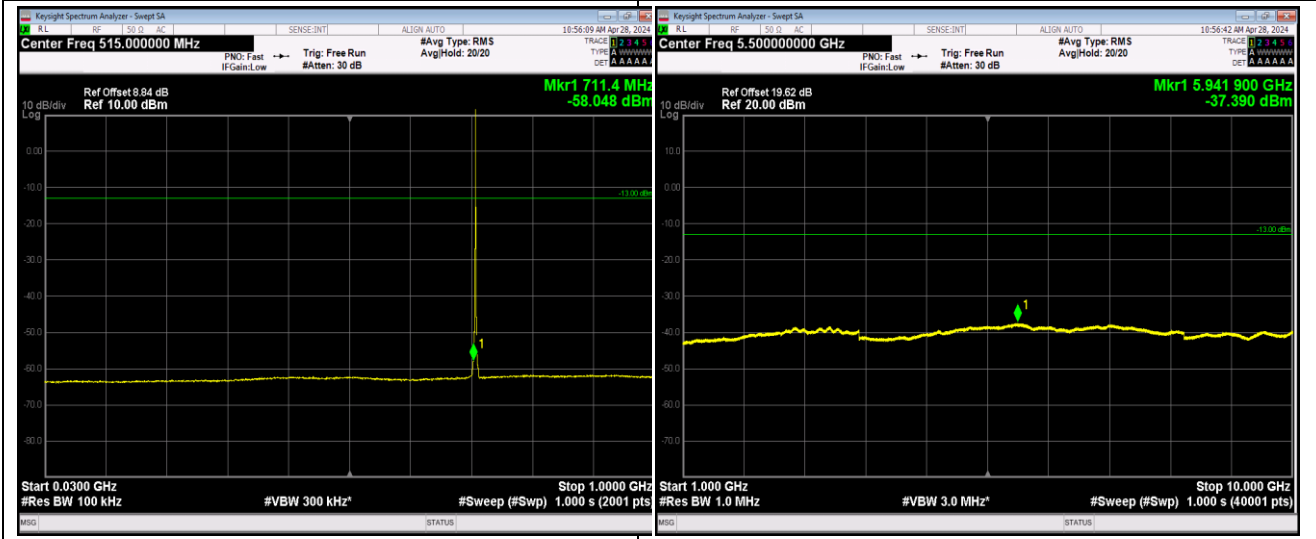
Band12_1.4MHz_64QAM_23173_1RB#0_30~1000_30~
