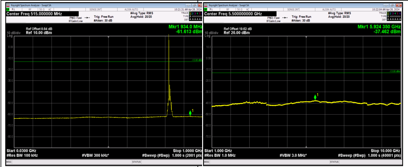
Band5_10MHz_QPSK_20450_1RB#0_30~1000_30~10 00
