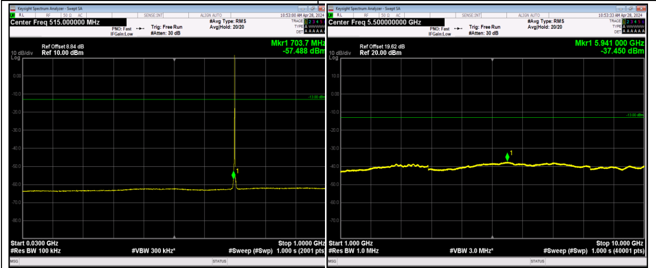
Band12_1.4MHz_64QAM_23095_1RB#0_30~1000_30~ 1000
