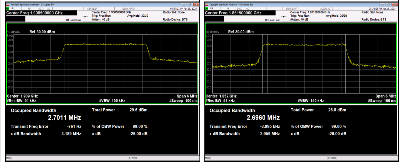
Band2-3MHz-16QAM-19185-15RB#0-PASS
