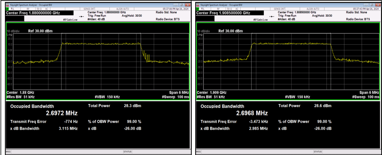
Band2-3MHz-64QAM-18900-15RB#0-PASS
