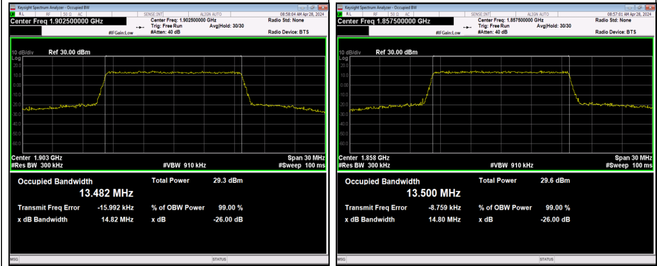
Band2-15MHz-QPSK-19125-75RB#0-PASS
