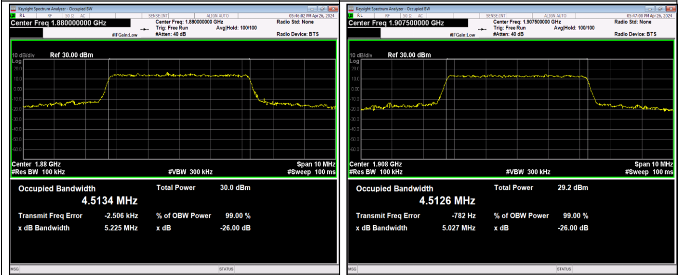
Band2-5MHz-16QAM-18900-25RB#0-PASS
