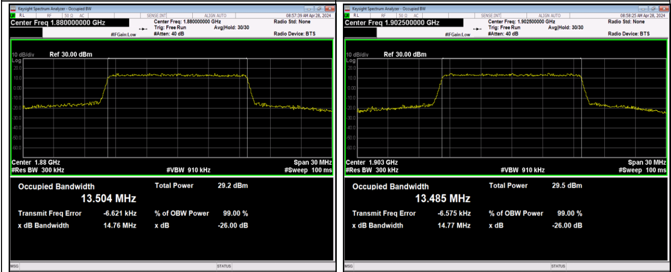
Band2-15MHz-16QAM-18900-75RB#0-PASS
