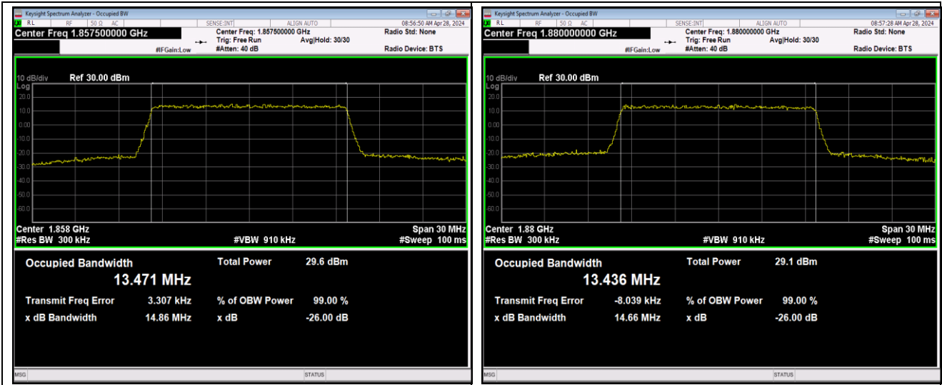
Band2-15MHz-QPSK-18675-75RB#0-PASS
