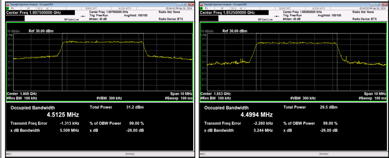
Band2-5MHz-QPSK-19175-25RB#0-PASS
