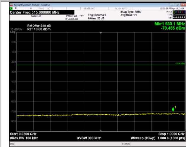
Band42_20MHz_64QAM_42590_1RB#0_30~1000_30~1000
