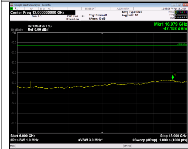
Band42_20MHz_16QAM_42590_1RB#0_6000~18000_60 00~18000
