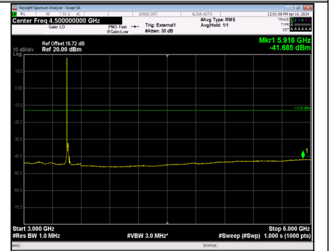
Band42_20MHz_64QAM_42190_1RB#0_3000~6000_300 0~6000
