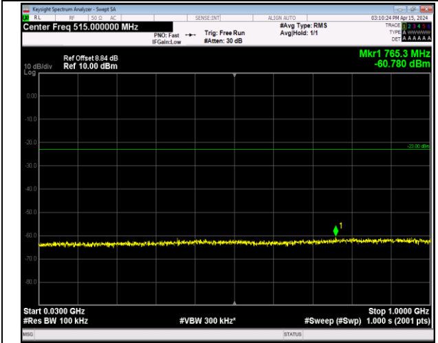
Band66_20MHz_64QAM_132322_1RB#0_30~1000_30~1000
