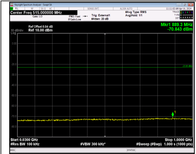
Band42_5MHz_64QAM_42115_1RB#0_30~1000_30~100 0
