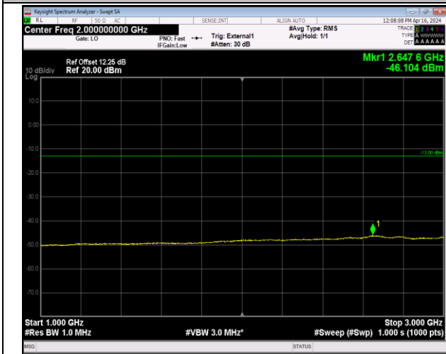
Band42_20MHz_QPSK_42990_1RB#0_1000~3000_1000~3000
