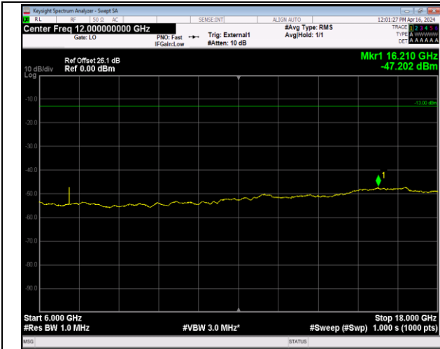
Band42_20MHz_64QAM_42190_1RB#0_6000~18000_6000~18000
