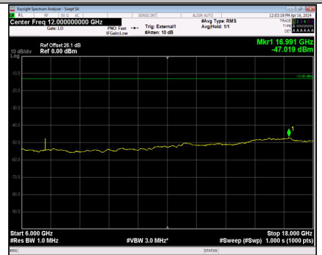
Band42_20MHz_QPSK_42590_1RB#0_6000~18000_6000~18000
