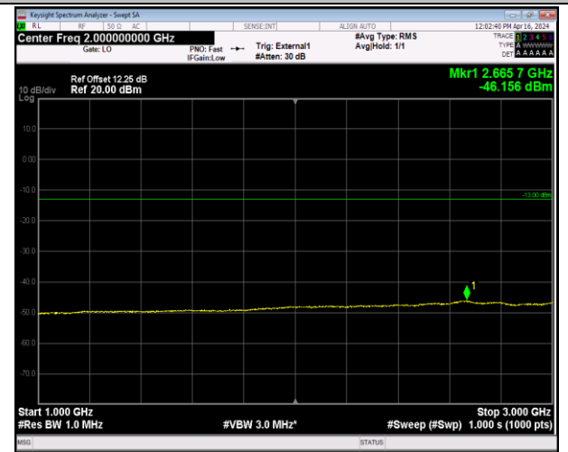
Band42_20MHz_QPSK_42590_1RB#0_1000~3000_1000~3000
