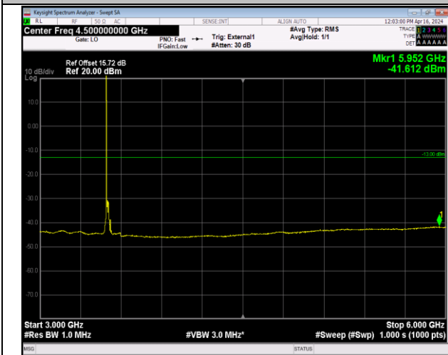
Band42_20MHz_QPSK_42590_1RB#0_3000~6000_3000~6000
