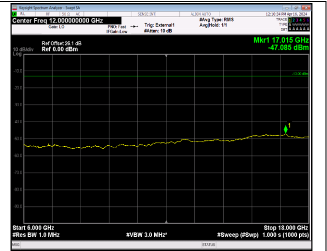
Band42_20MHz_16QAM_42990_1RB#0_6000~18000_60 00~18000
