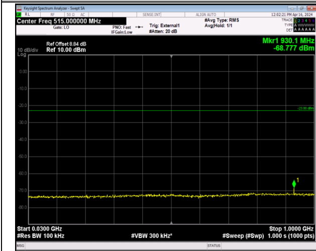
Band42_20MHz_QPSK_42590_1RB#0_30~1000_30~100 0
