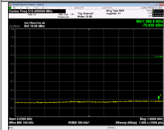
Band42_20MHz_16QAM_42990_1RB#0_30~1000_30~10 00
