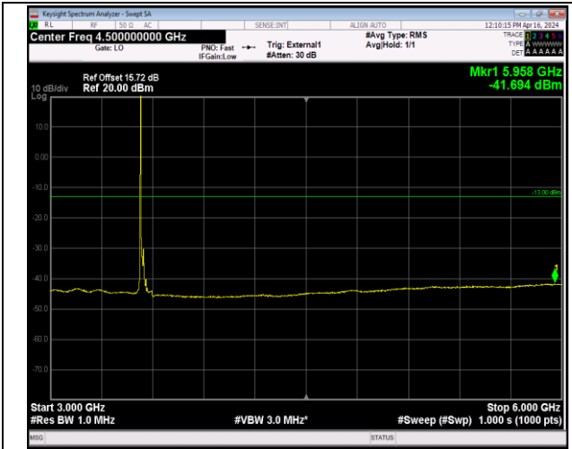
Band42_20MHz_16QAM_42990_1RB#0_3000~6000_300 0~6000
