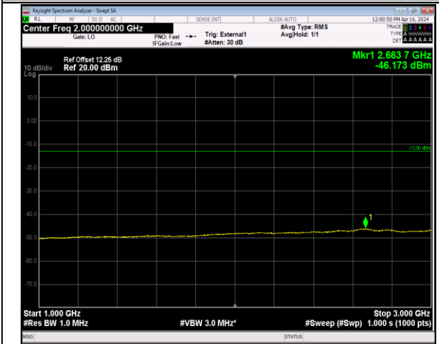
Band42_20MHz_64QAM_42190_1RB#0_1000~3000_100 0~3000
