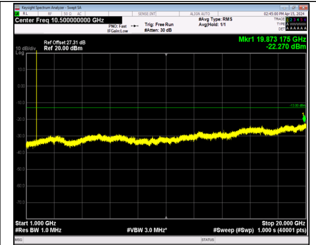
Band66_1.4MHz_QPSK_131979_1RB#0_1000~20000_10 00~20000
