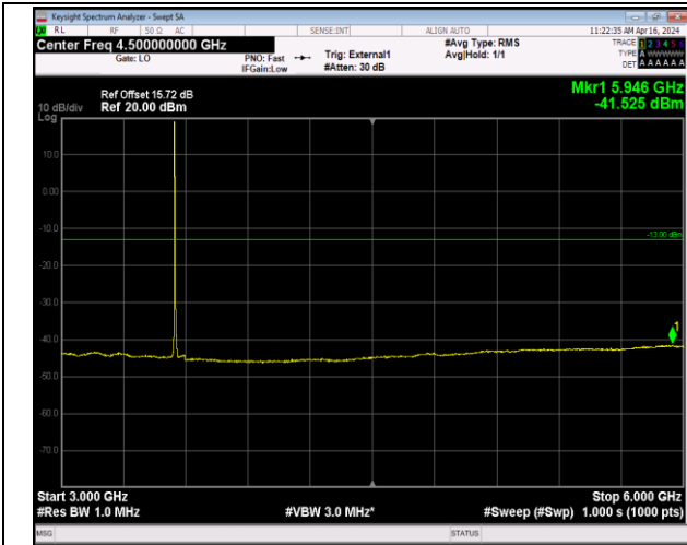
Band42_5MHz_64QAM_43065_1RB#0_3000~6000_3000 ~6000
