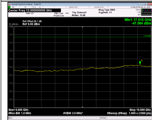
Band42_20MHz_QPSK_42990_1RB#0_6000~18000_6000~18000
