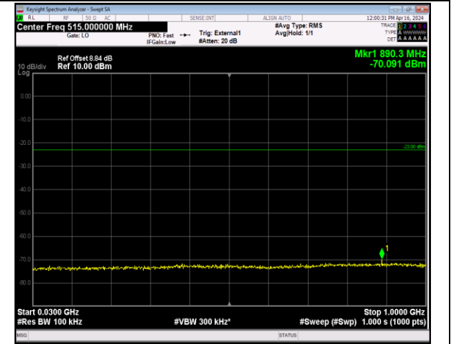
Band42_20MHz_64QAM_42190_1RB#0_30~1000_30~10 00
