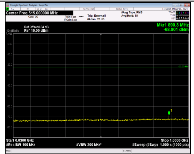
Band42_20MHz_QPSK_42190_1RB#0_30~1000_30~1000 0
