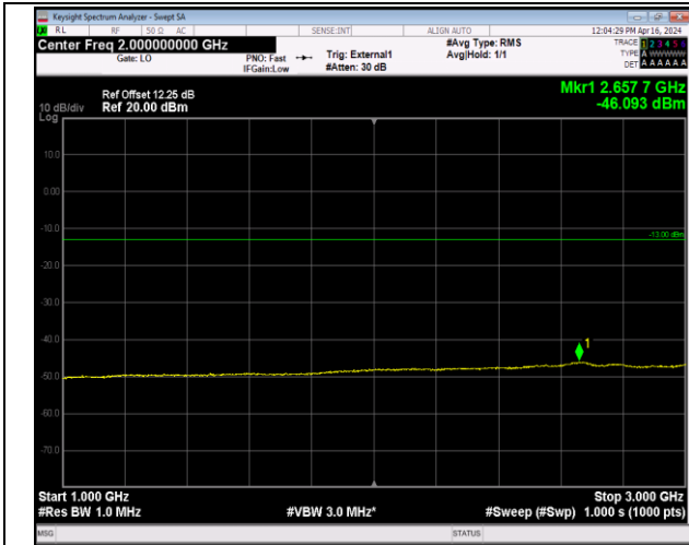
Band42_20MHz_16QAM_42590_1RB#0_1000~3000_100 0~3000
