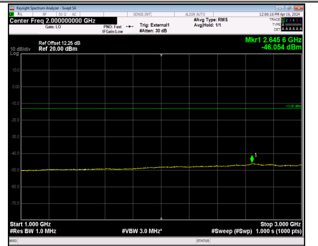
Band42_20MHz_64QAM_42590_1RB#0_1000~3000_1000~3000
