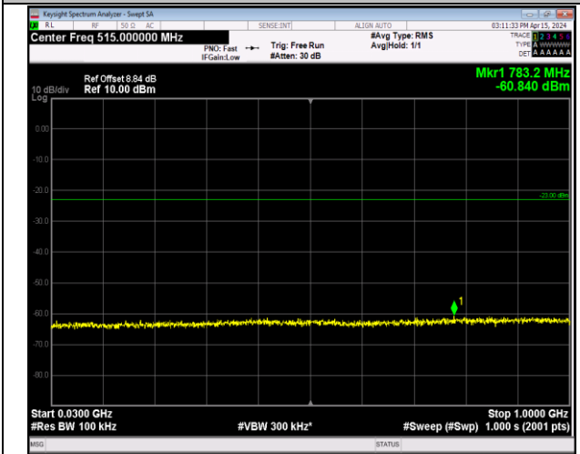
Band66_20MHz_64QAM_132572_1RB#0_30~1000_30~1000
