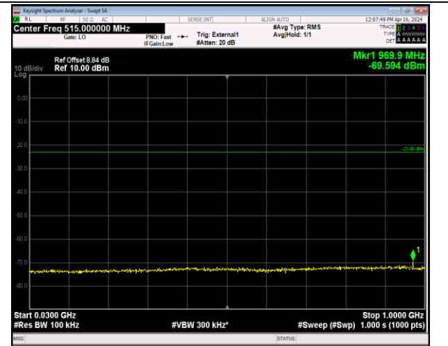
Band42_20MHz_QPSK_42990_1RB#0_30~1000_30~1000
