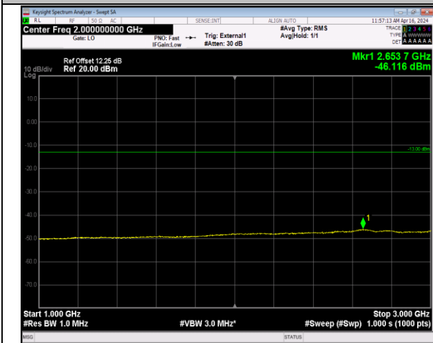
Band42_20MHz_QPSK_42190_1RB#0_1000~3000_1000~3000 ~3000
