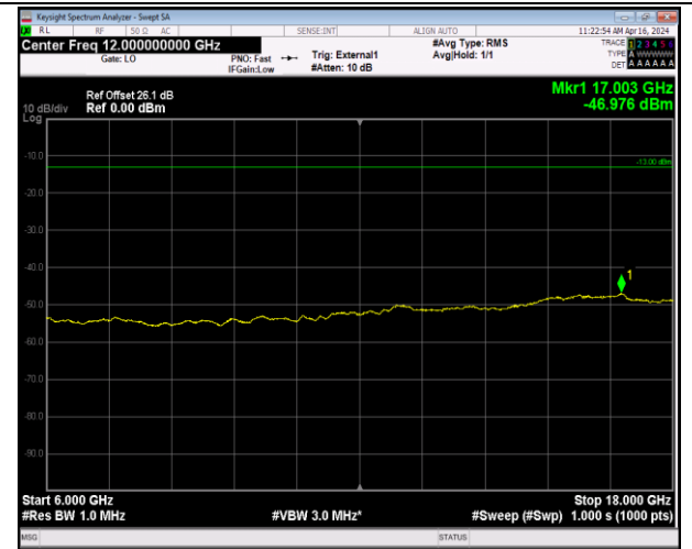
Band42_5MHz_64QAM_43065_1RB#0_6000~18000_600 0~18000
