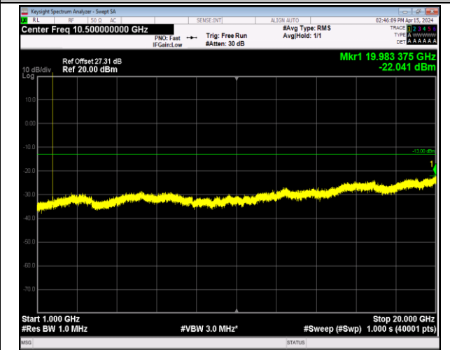
Band66_1.4MHz_QPSK_132322_1RB#0_1000~20000_10 00~20000
