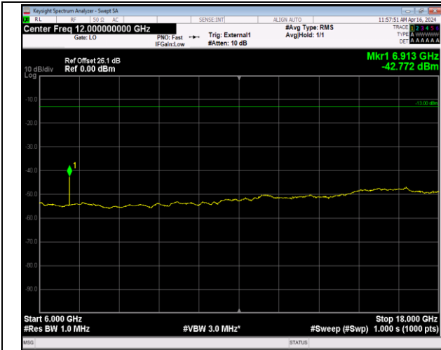
Band42_20MHz_QPSK_42190_1RB#0_6000~18000_600 0~18000
