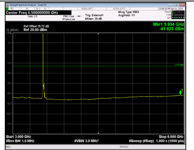
Band42_20MHz_QPSK_42990_1RB#0_3000~6000_3000~6000
