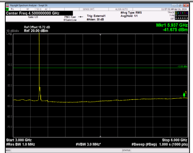
Band42_20MHz_QPSK_42190_1RB#0_3000~6000_3000~6000 ~6000
