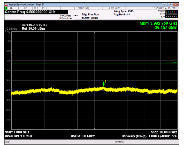
Band5_10MHz_64QAM_20450_1RB#0_1000~10000_100 0~10000
