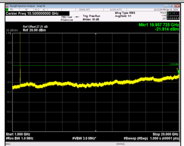
Band2_20MHz_64QAM_19100_1RB#0_1000~20000_100 0~20000
