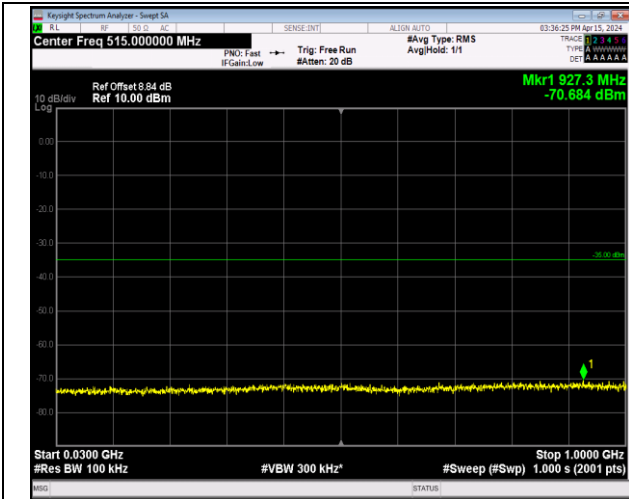
Band7_5MHz_64QAM_21425_1RB#0_30~1000_30~1000
