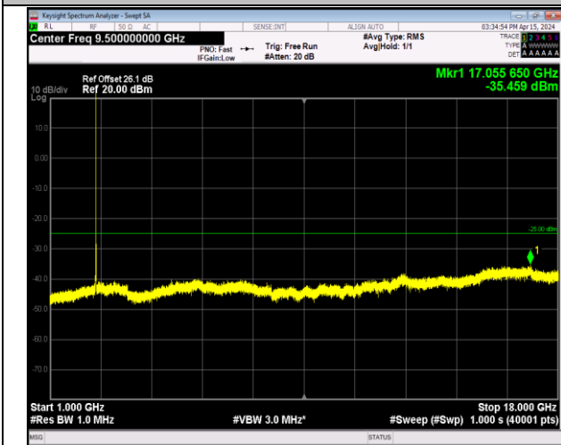
Band7_5MHz_64QAM_21100_1RB#0_1000~18000_1000~18000
