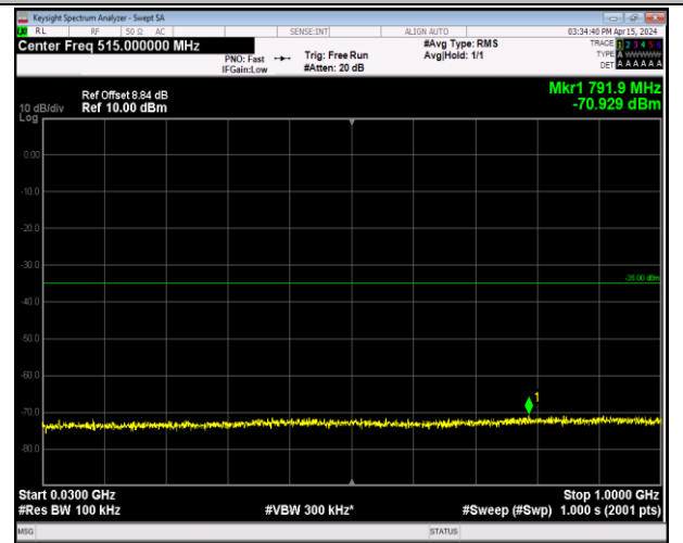
Band7_5MHz_64QAM_21100_1RB#0_30~1000_30~1000
