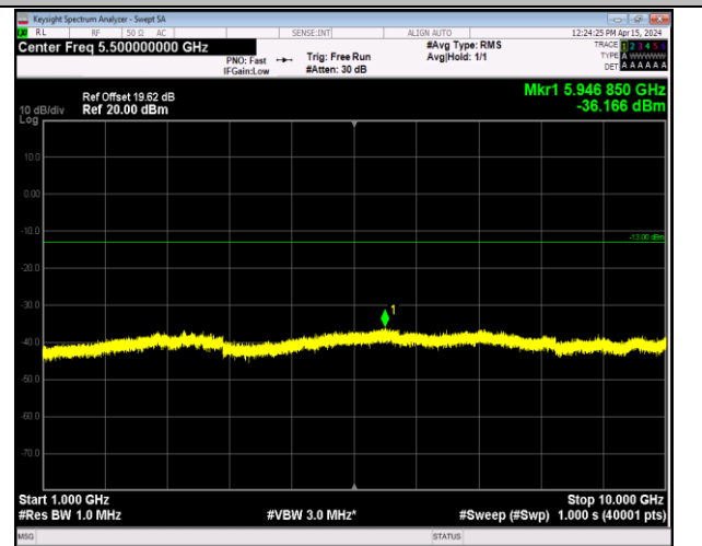
Band5_1.4MHz_64QAM_20643_1RB#0_1000~10000_100 0~10000
