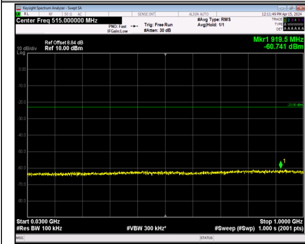
Band2_20MHz_QPSK_18900_1RB#0_30~1000_30~1000
