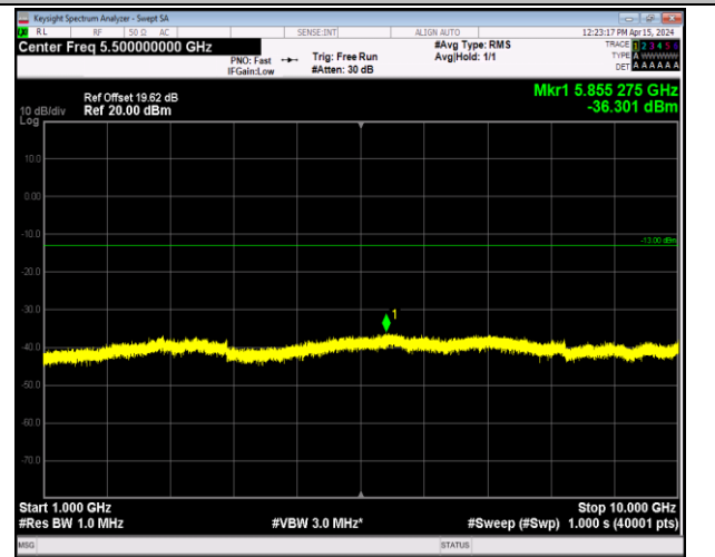
Band5_1.4MHz_64QAM_20525_1RB#0_1000~10000_100 0~10000
