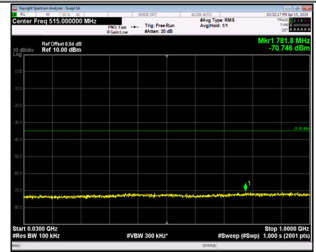
Band7_5MHz_16QAM_20775_1RB#0_30~1000_30~1000
