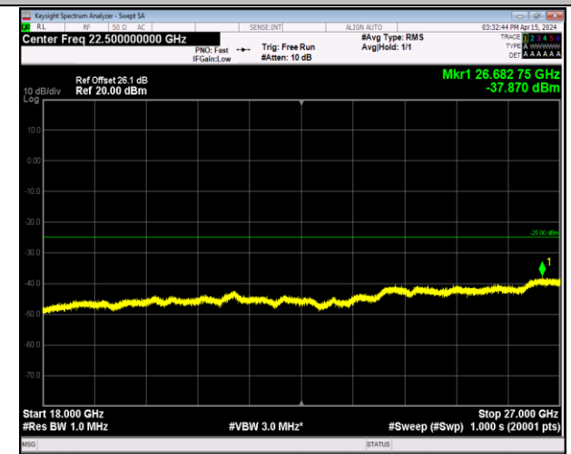
Band7_5MHz_16QAM_20775_1RB#0_18000~27000_18000~27000
