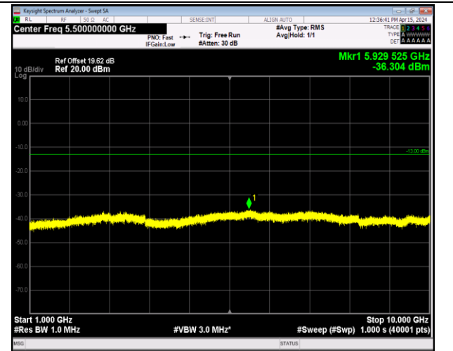
Band5_10MHz_16QAM_20450_1RB#0_1000~10000_100 0~10000
