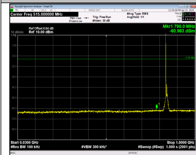
Band5_10MHz_64QAM_20600_1RB#0_30~1000_30~100 0
