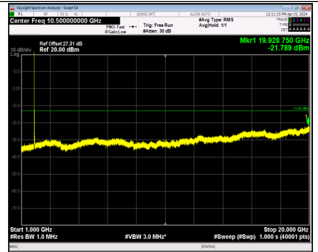
Band2_20MHz_16QAM_18700_1RB#0_1000~20000_100 0~20000
