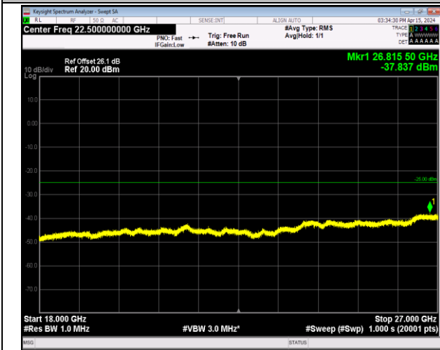
Band7_5MHz_16QAM_21100_1RB#0_18000~27000_18000~27000
