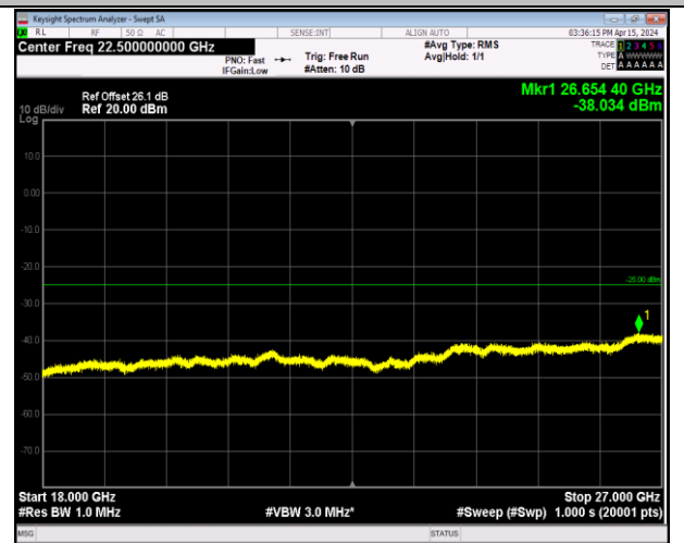
Band7_5MHz_16QAM_21425_1RB#0_18000~27000_18000~27000
