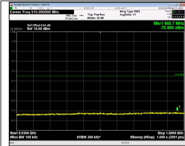
Band7_5MHz_64QAM_20775_1RB#0_30~1000_30~1000
