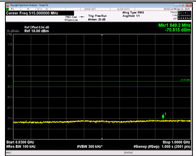
Band7_20MHz_QPSK_20850_1RB#0_30~1000_30~1000
