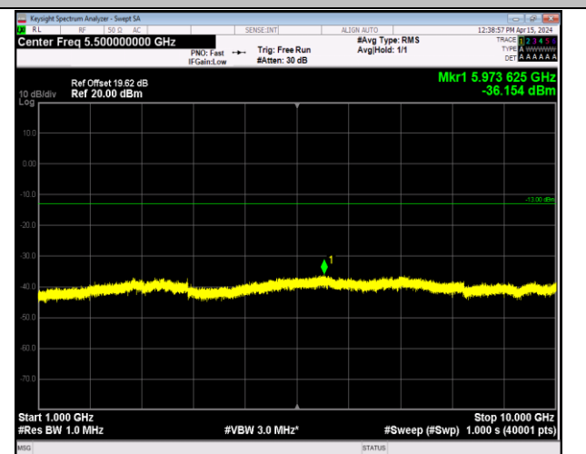
Band5_10MHz_16QAM_20600_1RB#0_1000~10000_100 0~10000
