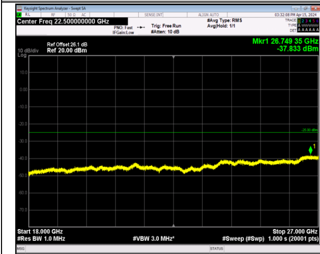
Band7_5MHz_QPSK_20775_1RB#0_18000~27000_18000~27000
