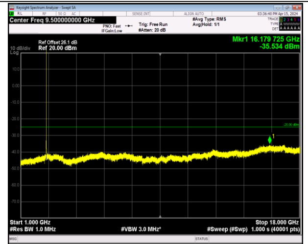
Band7_5MHz_64QAM_21425_1RB#0_1000~18000_1000~18000
