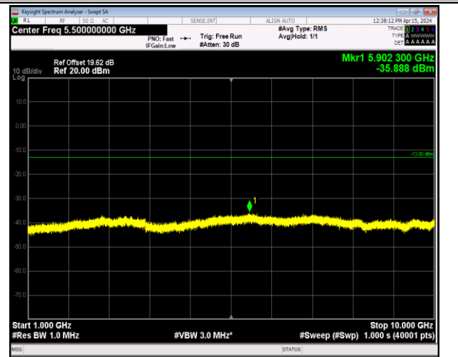
Band5_10MHz_64QAM_20525_1RB#0_1000~10000_100 0~10000
