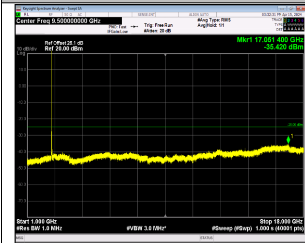
Band7_5MHz_16QAM_20775_1RB#0_1000~18000_1000~18000
