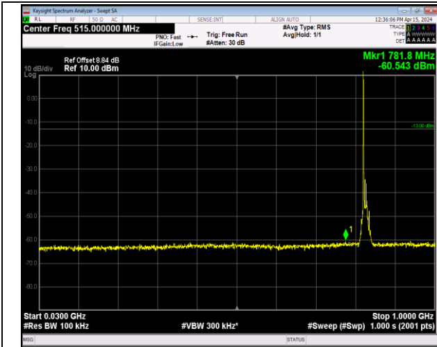
Band5_10MHz_QPSK_20450_1RB#0_30~1000_30~1000
