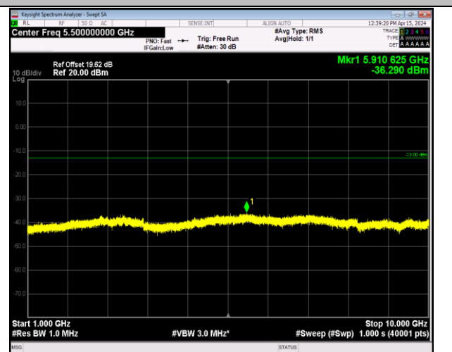
Band5_10MHz_64QAM_20600_1RB#0_1000~10000_100 0~10000
