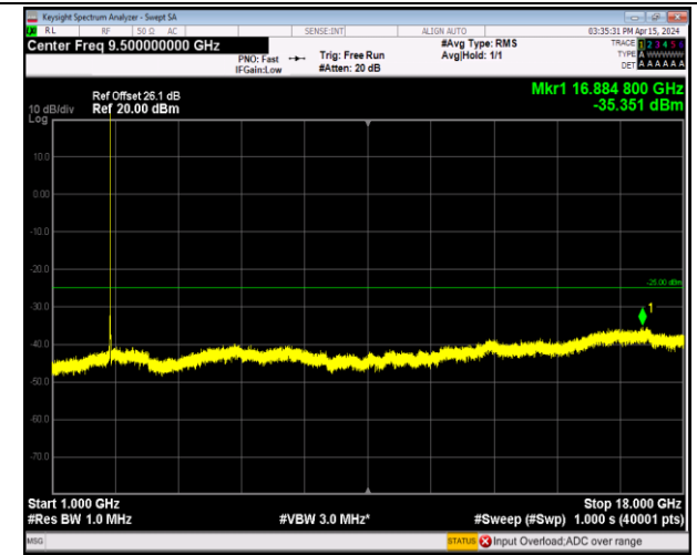
Band7_5MHz_QPSK_21425_1RB#0_1000~18000_1000~18000
