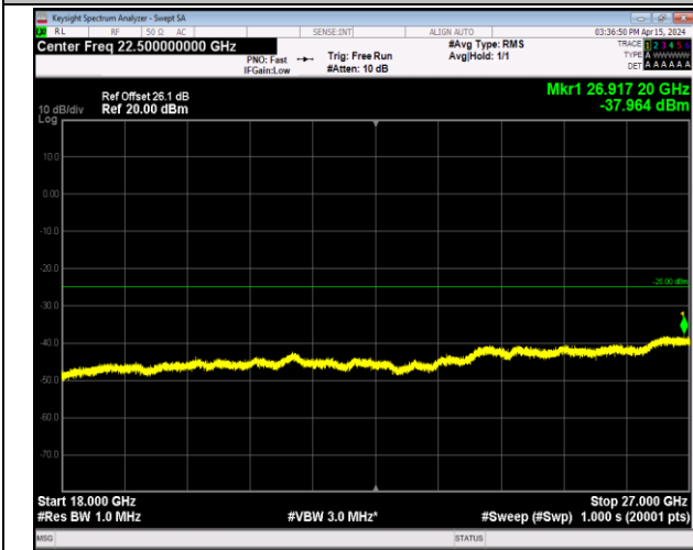
Band7_5MHz_64QAM_21425_1RB#0_18000~27000_18000~27000
