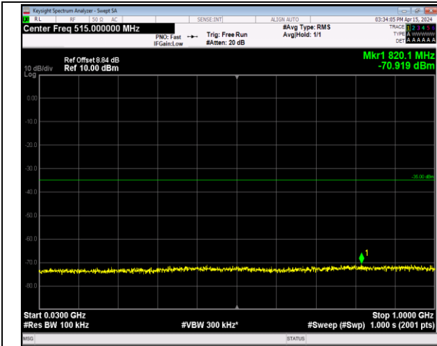
Band7_5MHz_16QAM_21100_1RB#0_30~1000_30~1000
