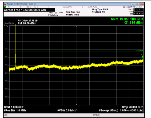
Band2_20MHz_QPSK_18900_1RB#0_1000~20000_1000 ~20000
