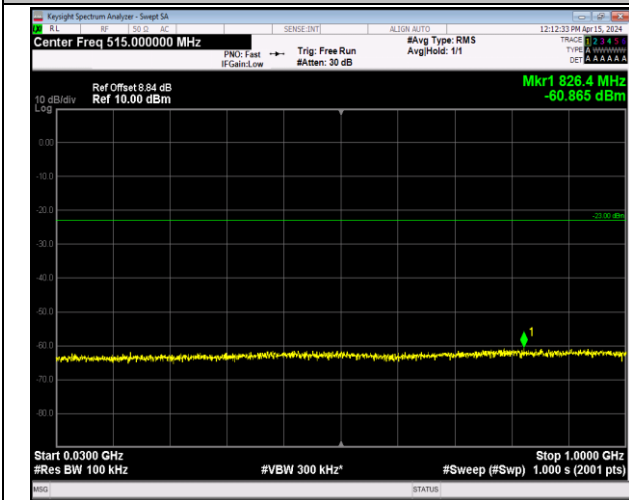
Band2_20MHz_64QAM_18900_1RB#0_30~1000_30~100 0
