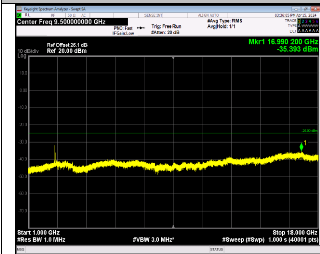
Band7_5MHz_16QAM_21425_1RB#0_1000~18000_1000~18000
