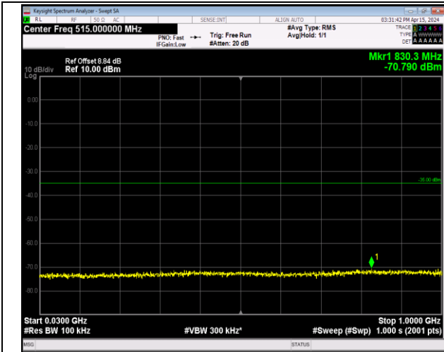
Band7_5MHz_QPSK_20775_1RB#0_30~1000_30~1000
