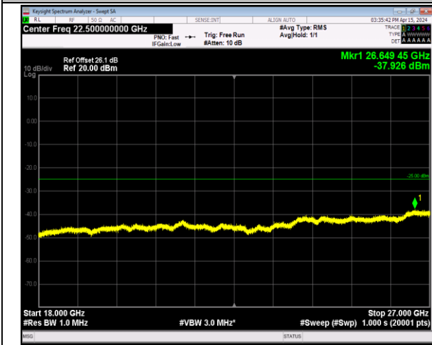
Band7_5MHz_QPSK_21425_1RB#0_18000~27000_18000~27000
