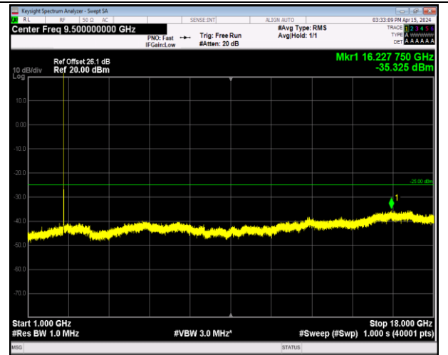
Band7_5MHz_64QAM_20775_1RB#0_1000~18000_1000~18000
