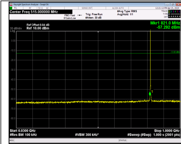
Band5_1.4MHz_QPSK_20407_1RB#0_30~1000_30~1000
