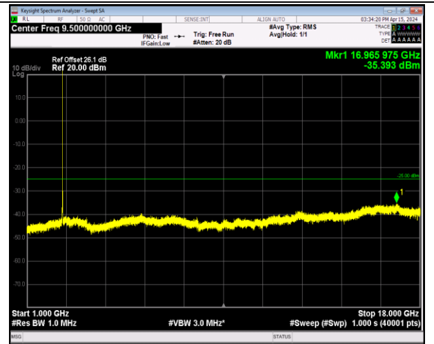
Band7_5MHz_16QAM_21100_1RB#0_1000~18000_1000~18000
