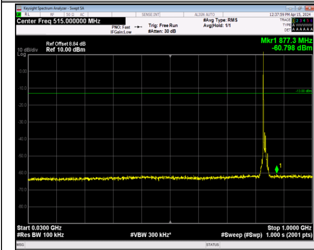
Band5_10MHz_64QAM_20525_1RB#0_30~1000_30~100 0
