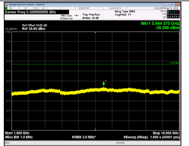
Band5_1.4MHz_64QAM_20407_1RB#0_1000~10000_100 0~10000
