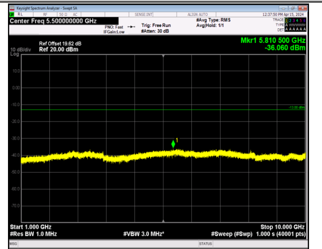
Band5_10MHz_16QAM_20525_1RB#0_1000~10000_100 0~10000
