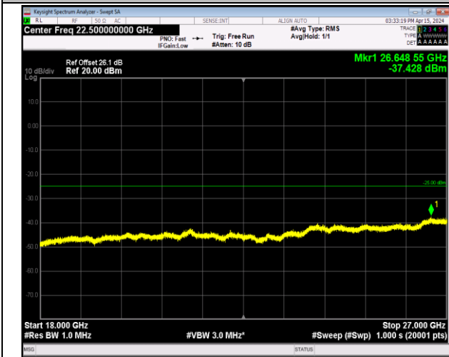
Band7_5MHz_64QAM_20775_1RB#0_18000~27000_18000~27000
