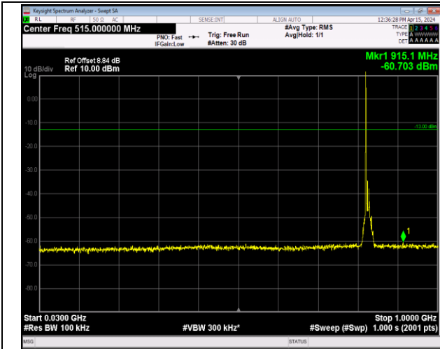
Band5_10MHz_16QAM_20450_1RB#0_30~1000_30~100 0
