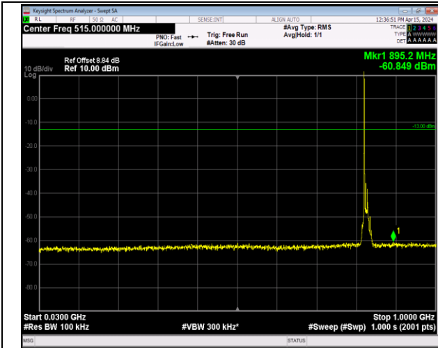
Band5_10MHz_64QAM_20450_1RB#0_30~1000_30~100 0
