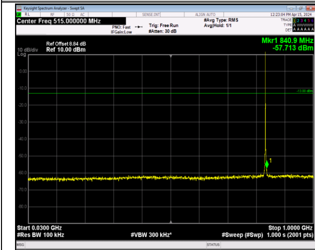
Band5_1.4MHz_64QAM_20525_1RB#0_30~1000_30~10 00
