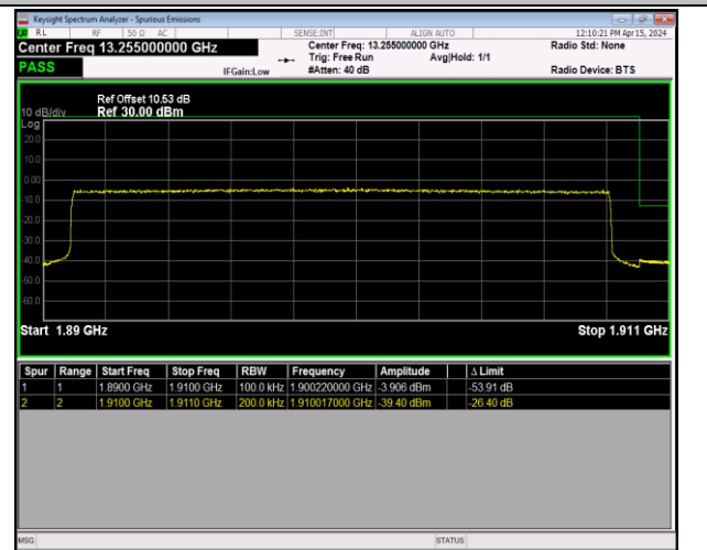
Band2_20MHz_64QAM_19100_100RB#0
