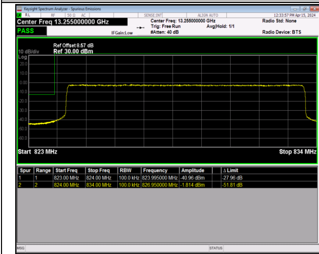
Band5_10MHz_64QAM_20450_50RB#0
