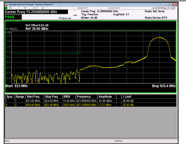
Band5_1.4MHz_64QAM_20407_1RB#5
