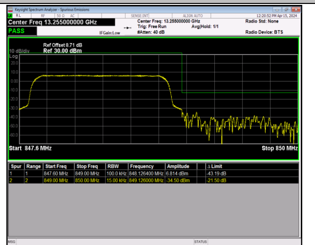
Band5_1.4MHz_64QAM_20643_6RB#0
