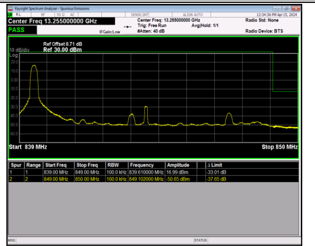
Band5_10MHz_64QAM_20600_1RB#0
