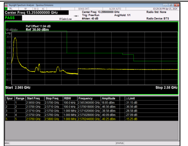
Band7_5MHz_16QAM_21425_1RB#0
