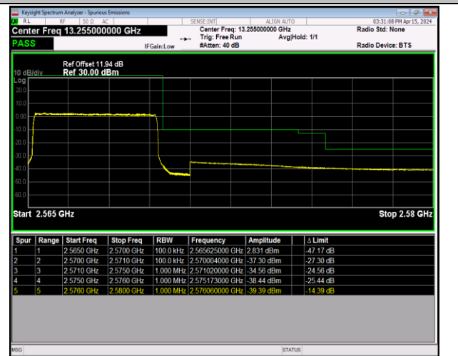
Band7_5MHz_16QAM_21425_25RB#0
