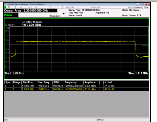
Band2_20MHz_QPSK_19100_100RB#0
