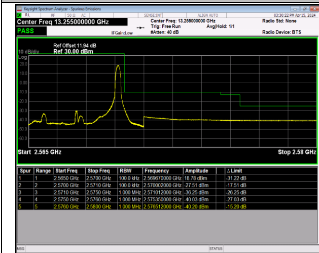
Band7_5MHz_16QAM_21425_1RB#24
