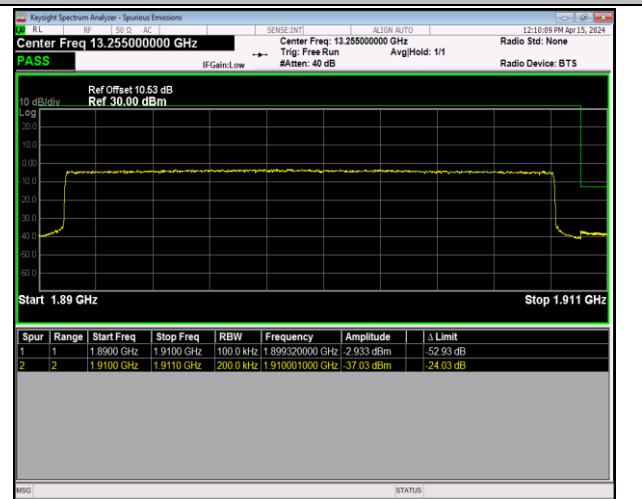
Band2_20MHz_16QAM_19100_100RB#0
