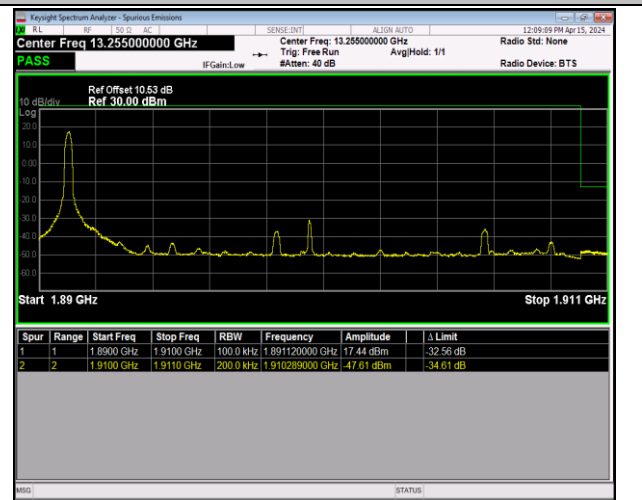
Band2_20MHz_64QAM_19100_1RB#0
