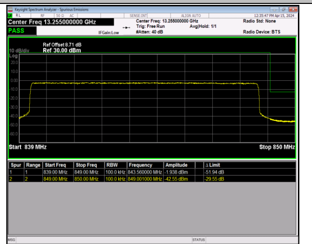
Band5_10MHz_64QAM_20600_50RB#0
