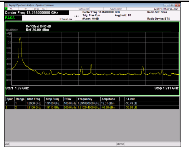
Band2_20MHz_QPSK_19100_1RB#0
