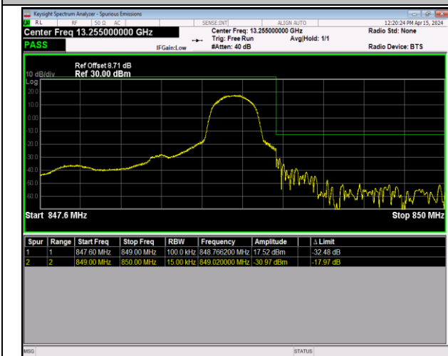
Band5_1.4MHz_64QAM_20643_1RB#5
