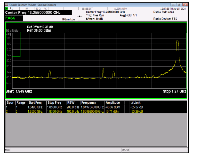
Band2_20MHz_64QAM_18700_1RB#99
