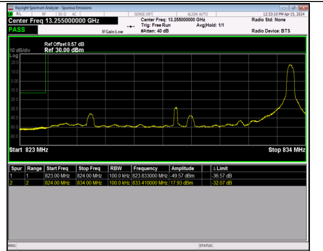
Band5_10MHz_16QAM_20450_1RB#49
