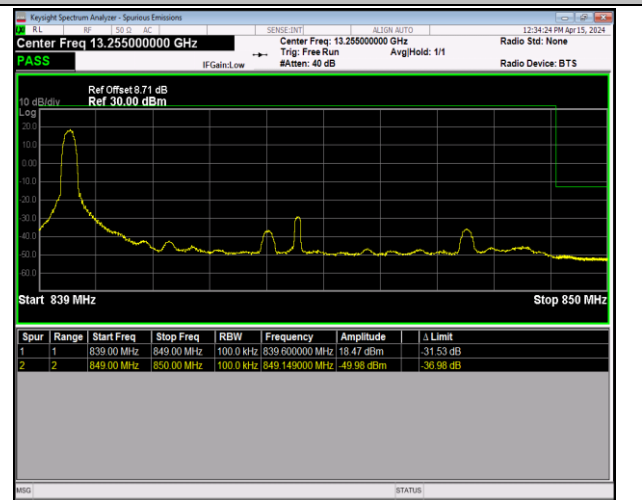
Band5_10MHz_16QAM_20600_1RB#0
