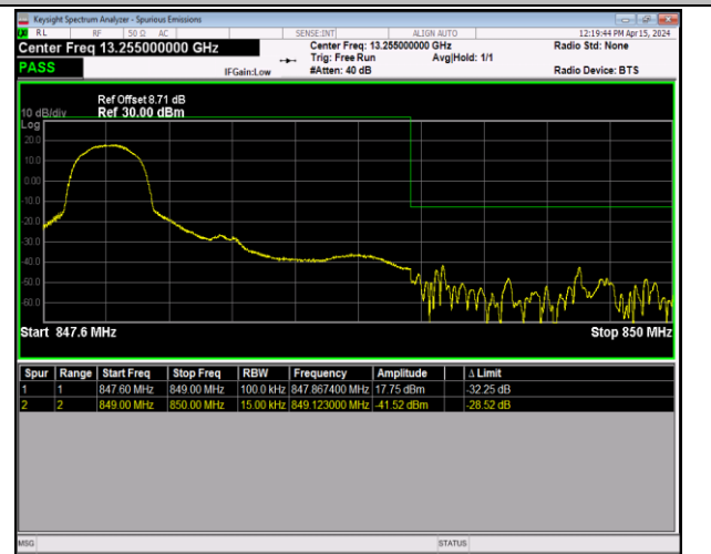
Band5_1.4MHz_16QAM_20643_1RB#0
