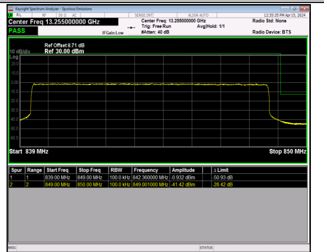
Band5_10MHz_16QAM_20600_50RB#0
