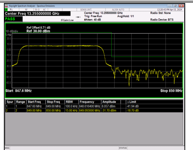
Band5_1.4MHz_16QAM_20643_6RB#0
