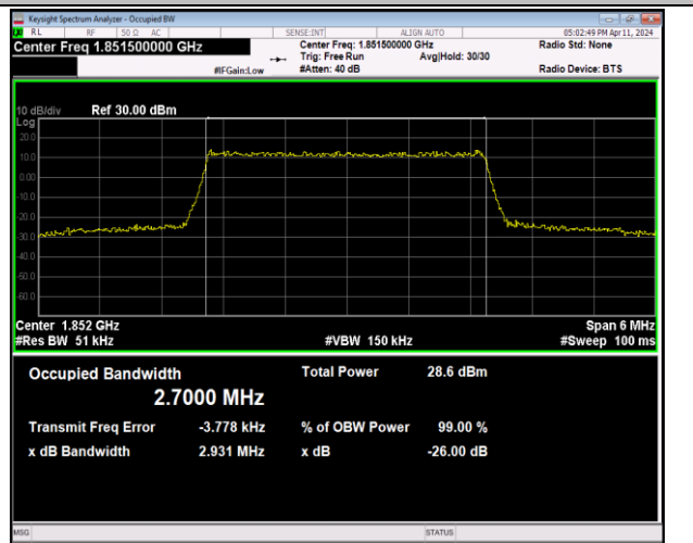
Band2-3MHz-64QAM-18615-15RB#0-PASS
