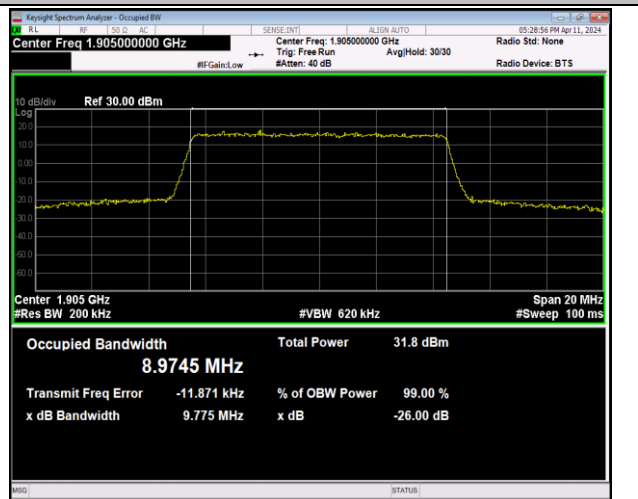
Band2-10MHz-QPSK-19150-50RB#0-PASS
