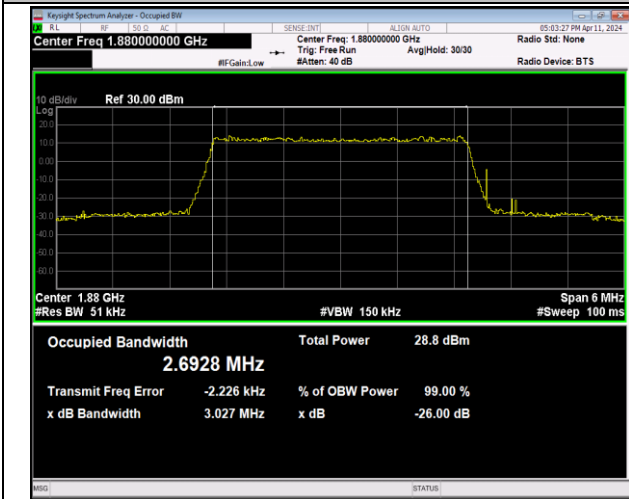
Band2-3MHz-64QAM-18900-15RB#0-PASS
