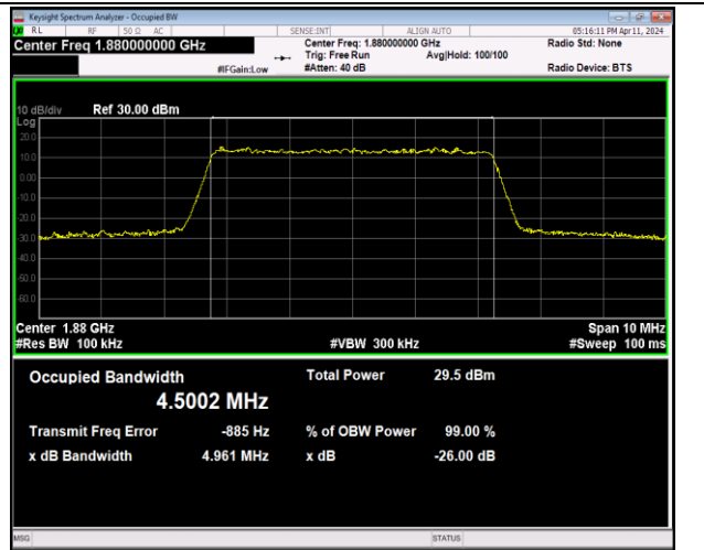
Band2-5MHz-64QAM-18900-25RB#0-PASS
