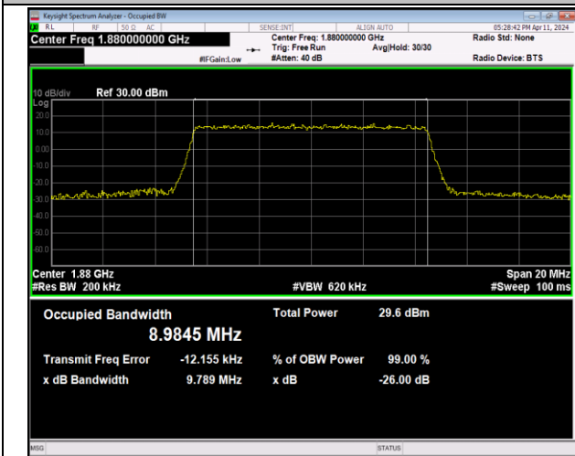
Band2-10MHz-64QAM-18900-50RB#0-PASS
