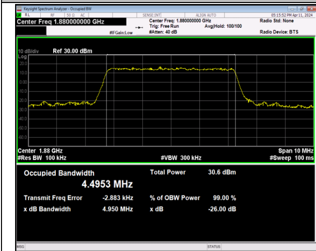
Band2-5MHz-16QAM-18900-25RB#0-PASS
