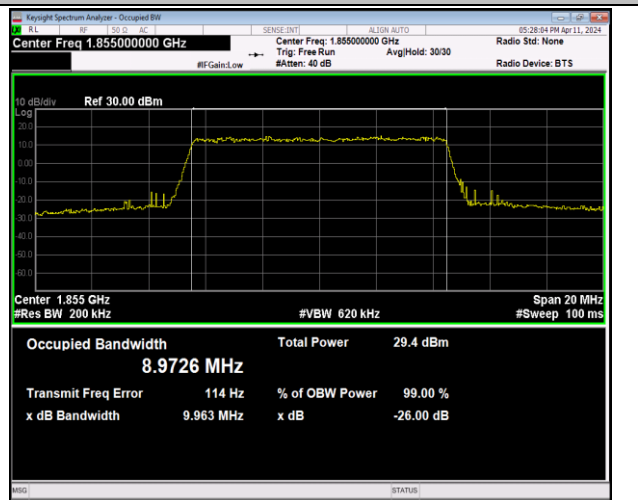
Band2-10MHz-64QAM-18650-50RB#0-PASS
