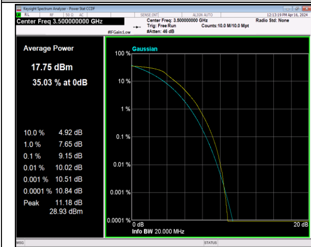
42(3450-3550)-20MHz-QPSK-42590-100RB#0-PASS
