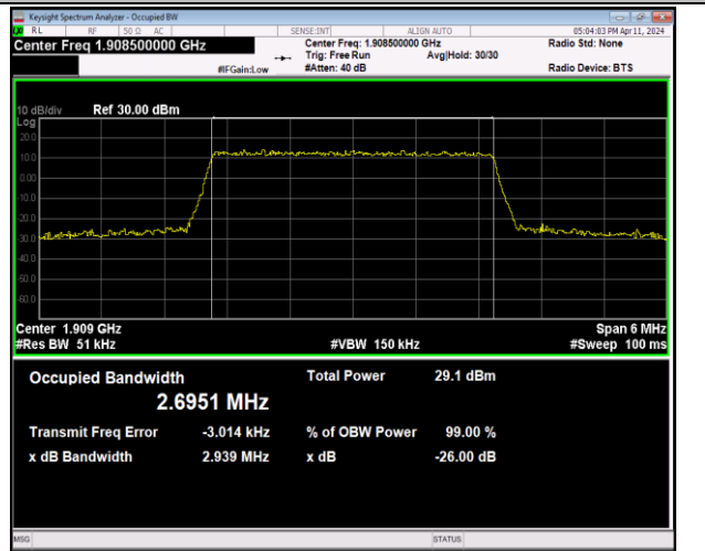
Band2-3MHz-64QAM-19185-15RB#0-PASS
