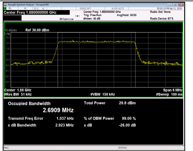
Band2-3MHz-16QAM-18900-15RB#0-PASS
