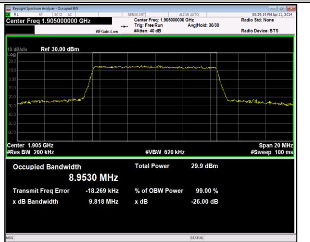
Band2-10MHz-64QAM-19150-50RB#0-PASS
