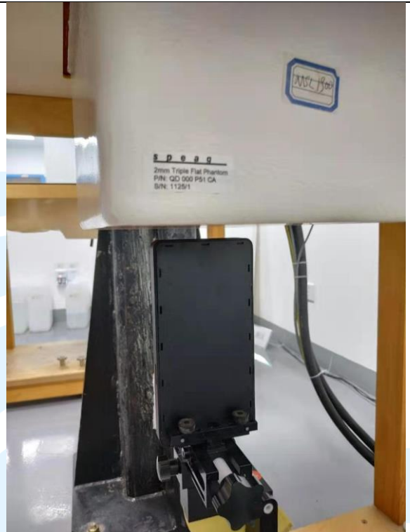
Bottom Side of EUT with 1.0 cm Gap
