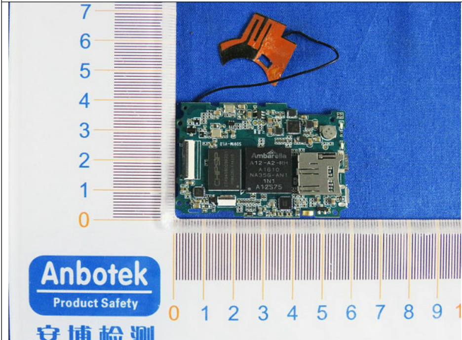
3. Figure PCB of the EUT-Front View
