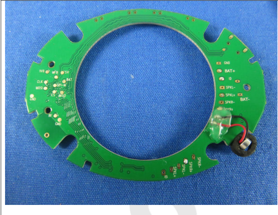
7. Figure PCB of the EUT-Back View
