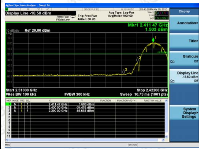
802.11b_Low Channel / 2412MHz
