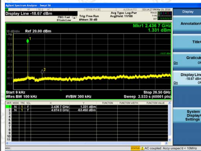
802.11b_Middle Channel / 2437MHz
