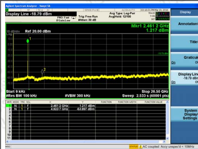
802.11b_High Channel / 2462MHz
