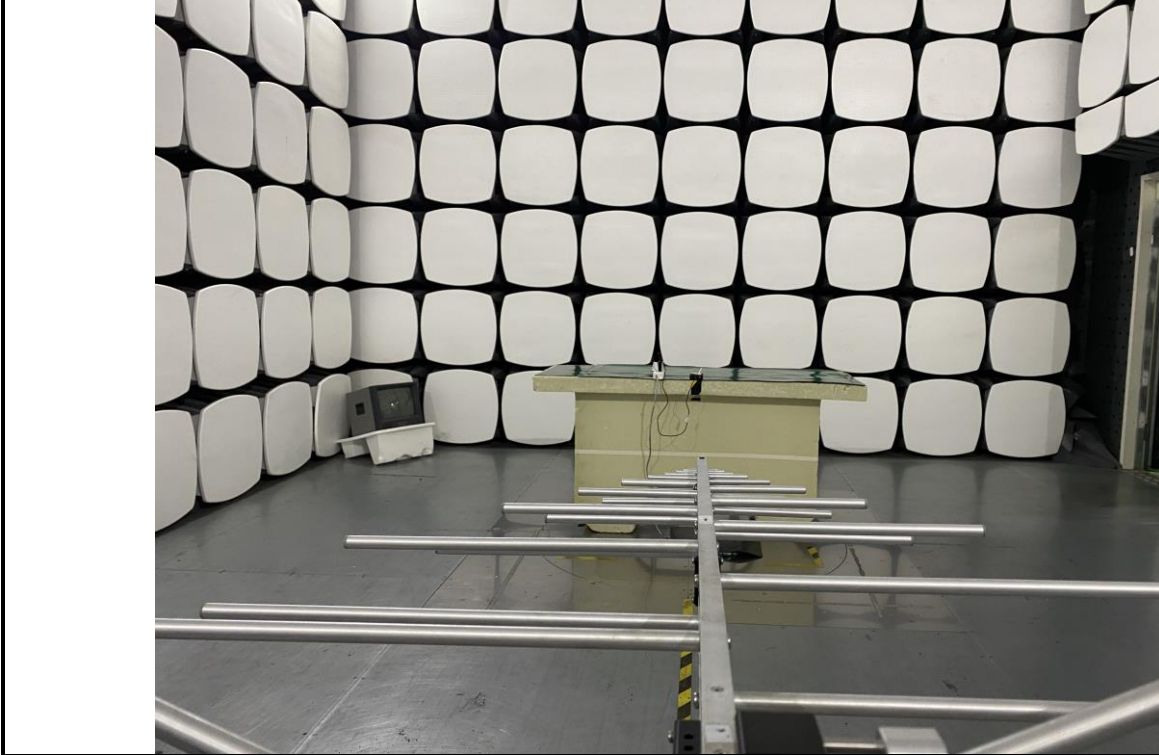
Radiated emission Test Setup (30 MHz to 1000 MHz)
