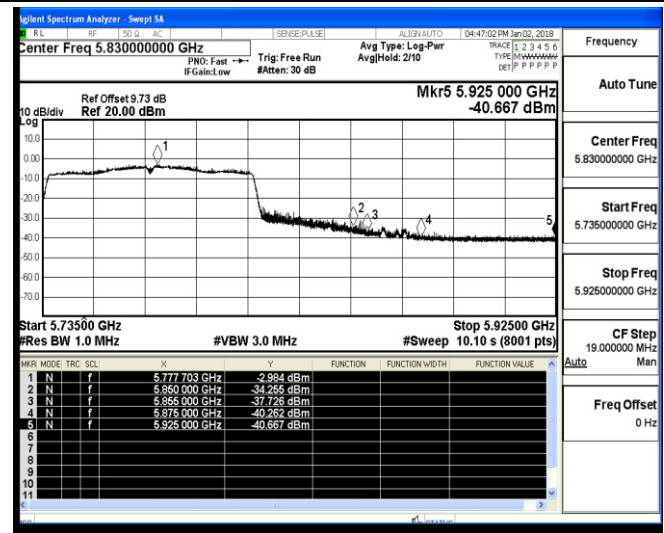
Channel 155 / 5775 MHz – Peak
