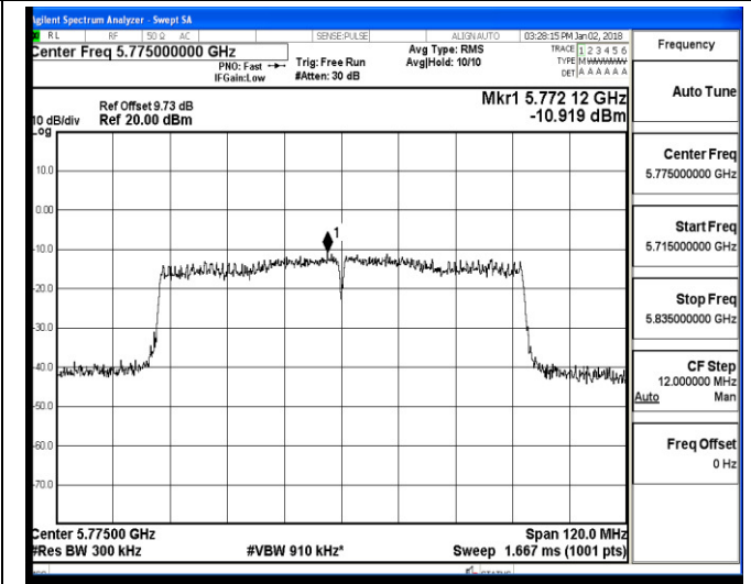
Channel 155 / 5775 MHz
