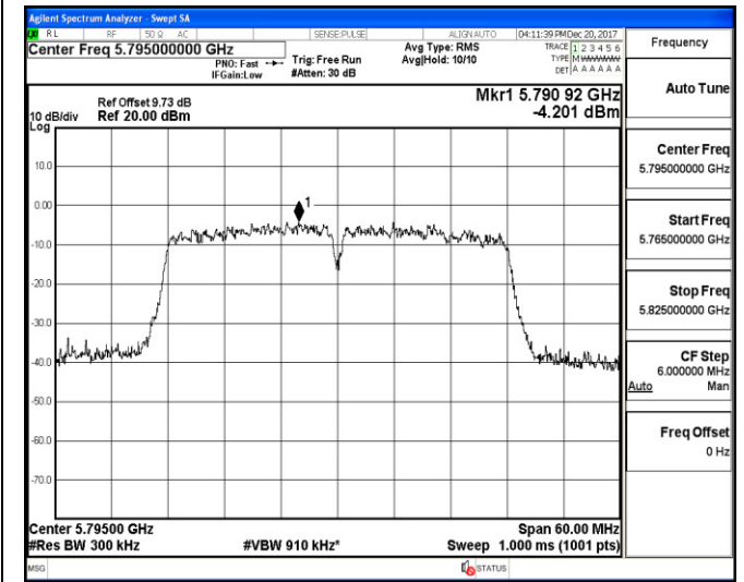
Channel 159 / 5795 MHz
