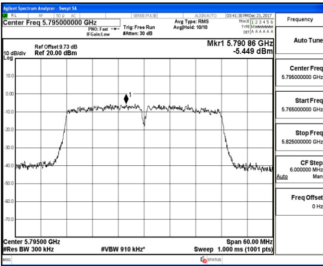
Channel 159 / 5795 MHz
