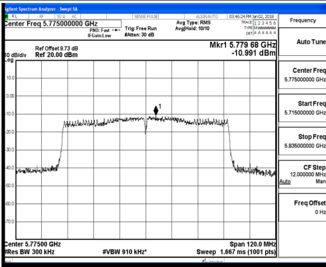
Channel 155 / 5775 MHz
