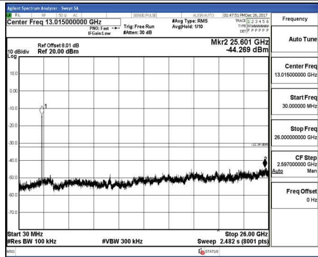
30 MHz – 26 GHz
