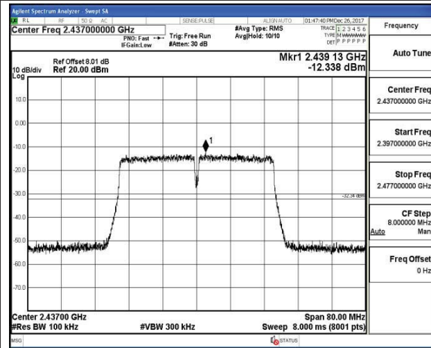
2422 MHz – 2452 MHz
