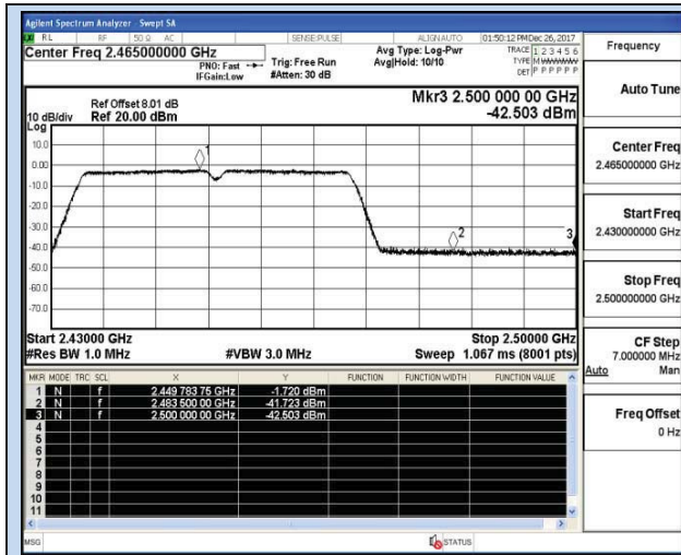
Channel 11 / 2462 MHz – Peak
