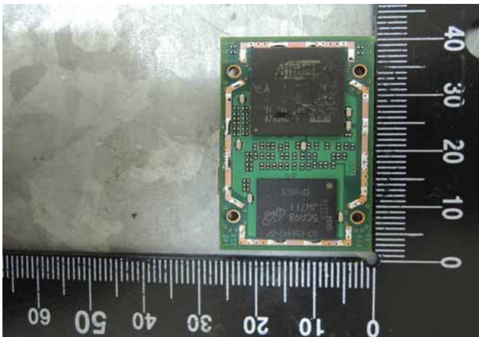
Internal View of EUT – 9
