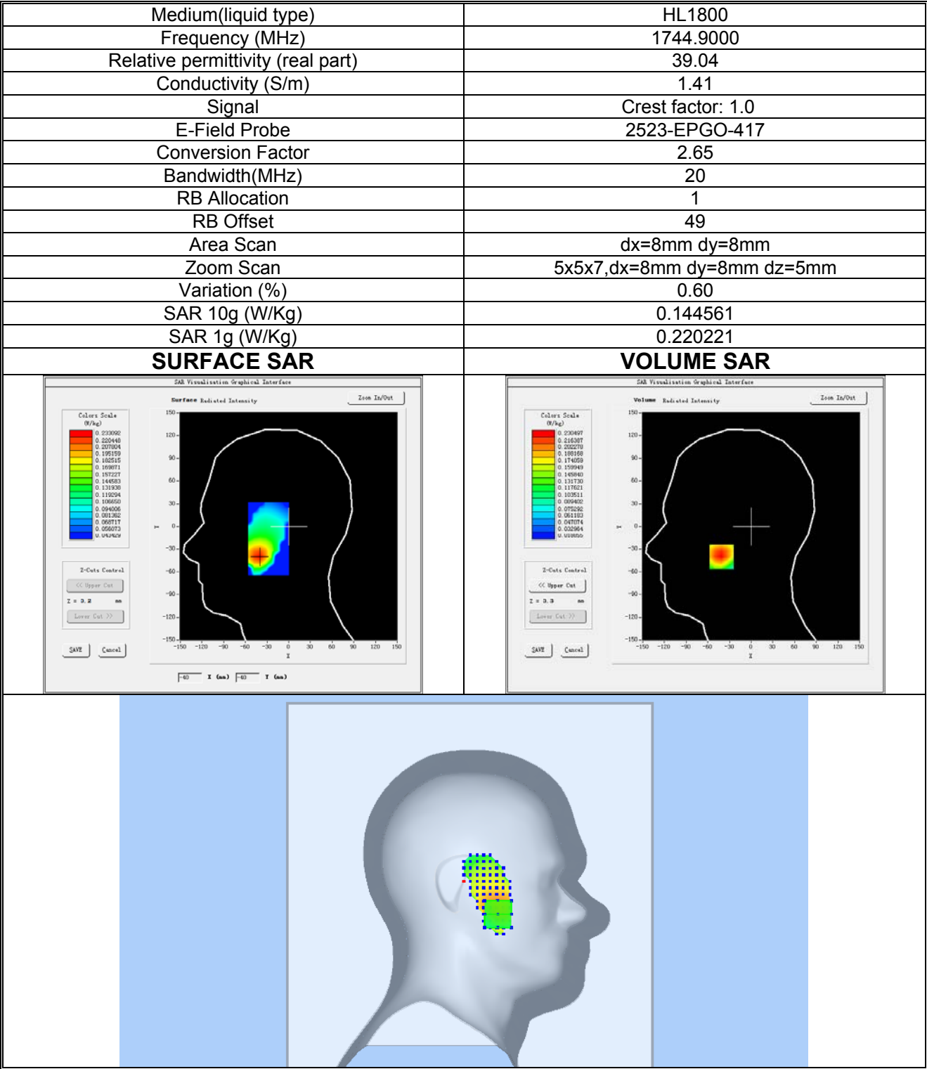
Plot 23:LTE BAND 66, Middle channel (Left Head Cheek) Product Description: Smart Phone Test Date: 2024-07-02
