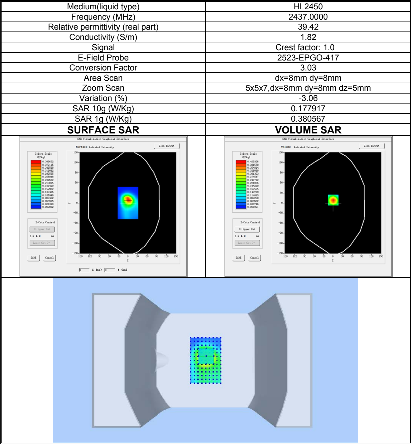
Plot 26: 2.4G Wi-Fi, Middle channel (Body-worn/ Hotspot, Back Side) Product Description: Smart Phone Test Date: 2024-06-26
