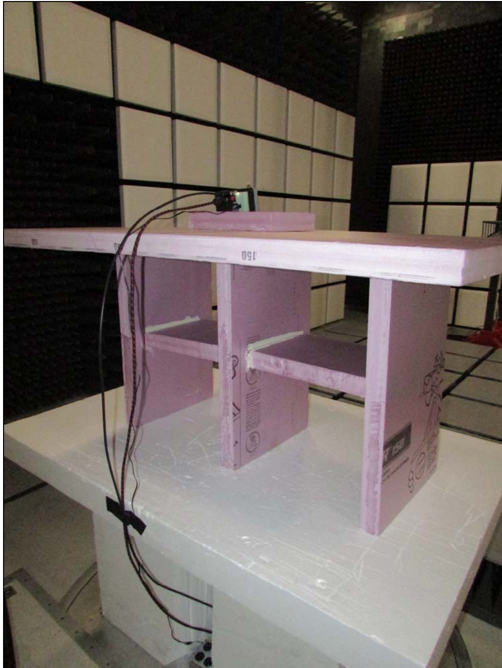
Figure 2: Back View – Above 1 GHz
